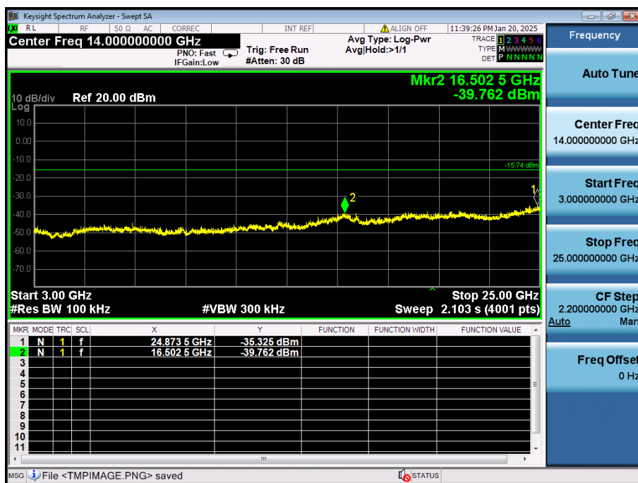
Conducted Spurious Emissions (Test Mode:2DH5) (NTNV)
