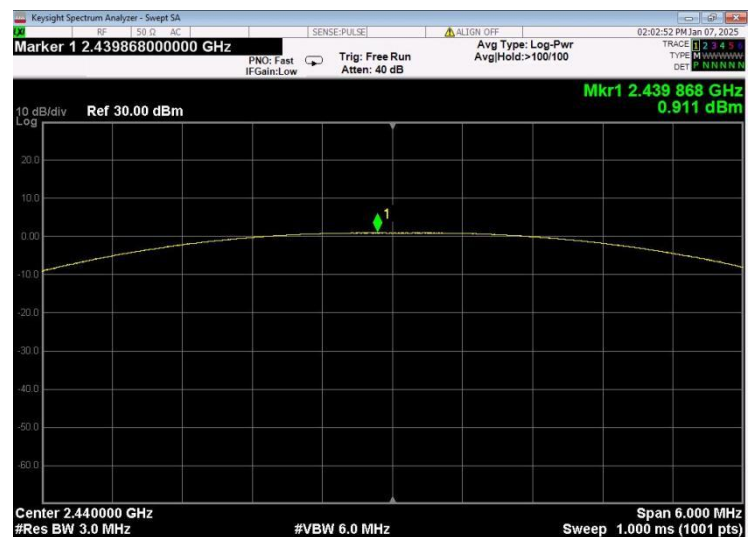
BLE_1M, 2440MHz
