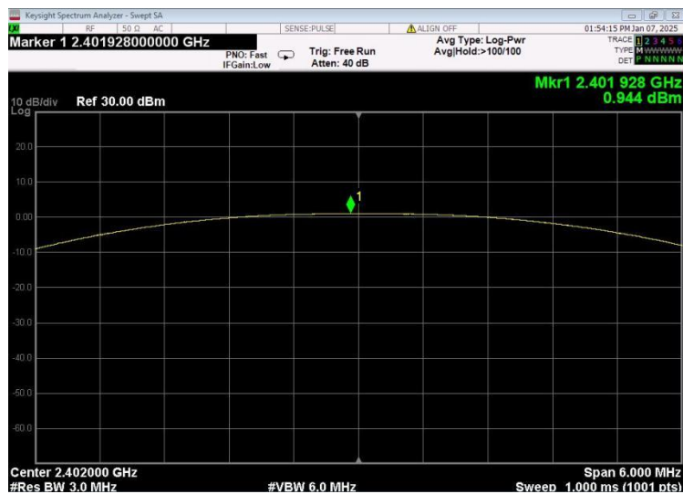
BLE_1M, 2402MHz
