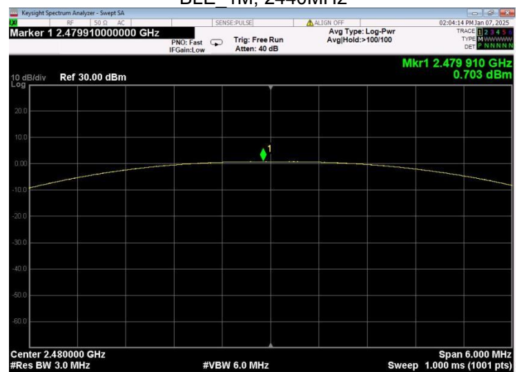
BLE_1M, 2480MHz
