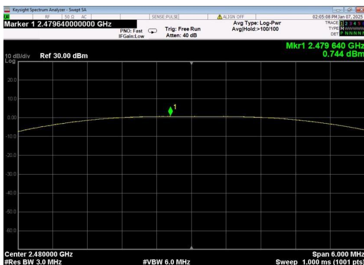
BLE_2M, 2480MHz
