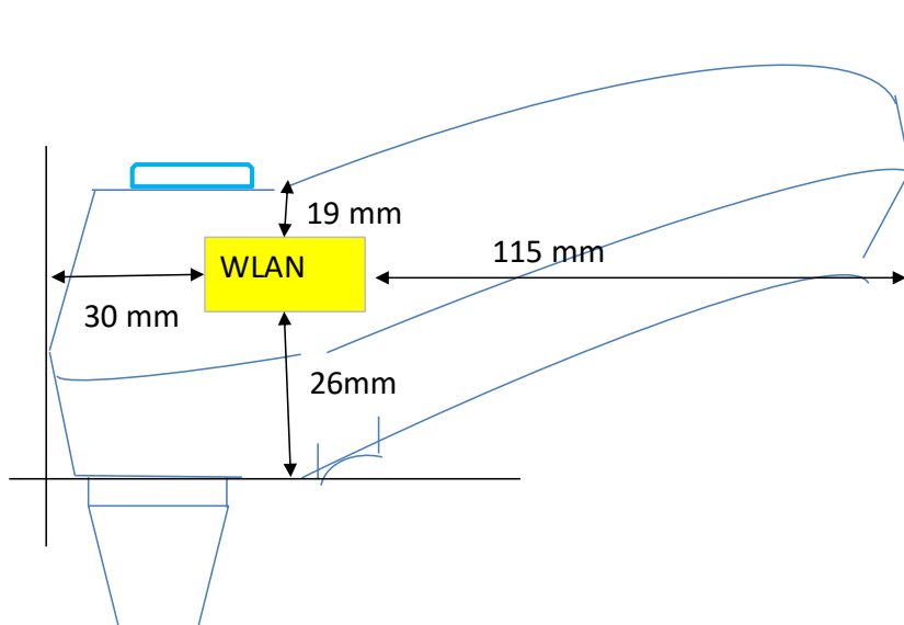
Photograph 16. Antenna position of EUT
