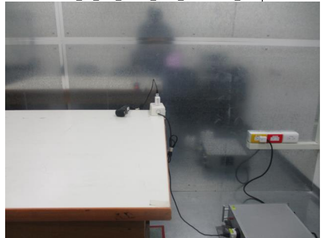
Part_15_247_WLAN_2.4G_Conduction_Setup
