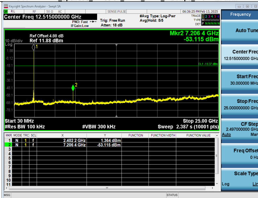
2 Spurious Emission NVNT_ANT1_125 kbps 2402
