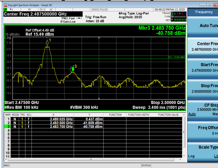
2_Bandedge_NVNT_ANT1_125 kbps_2480
