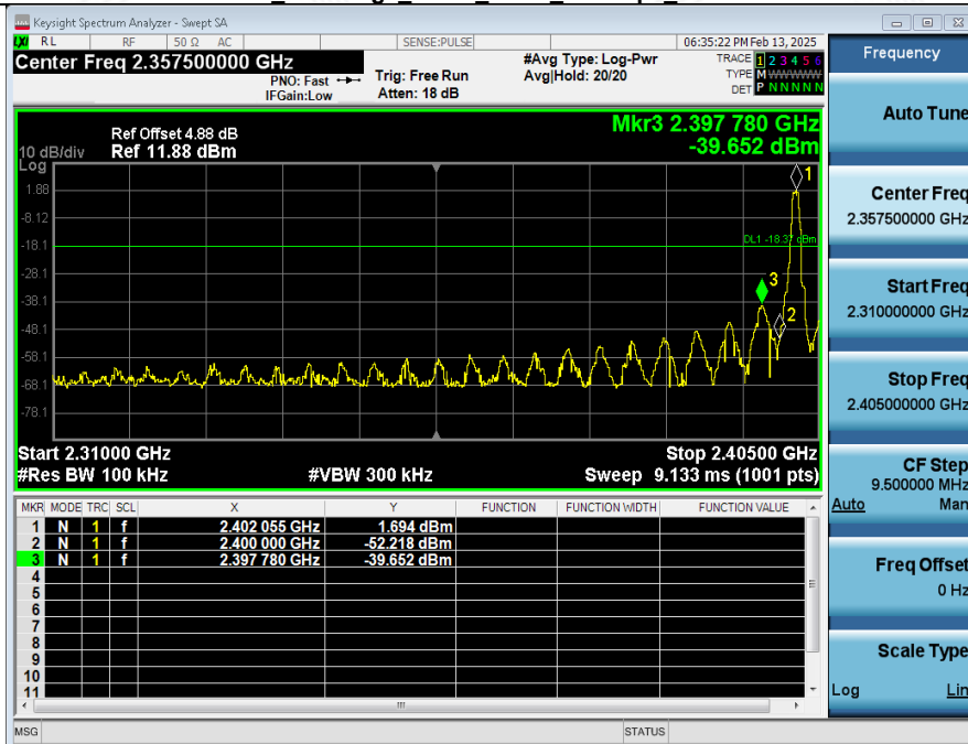
2 Bandedge NVNT_ANT1_125 kbps_2402
