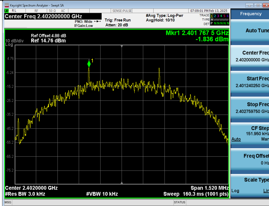
Power Spectral Density NVNT ANT1 500 kbps 2402
