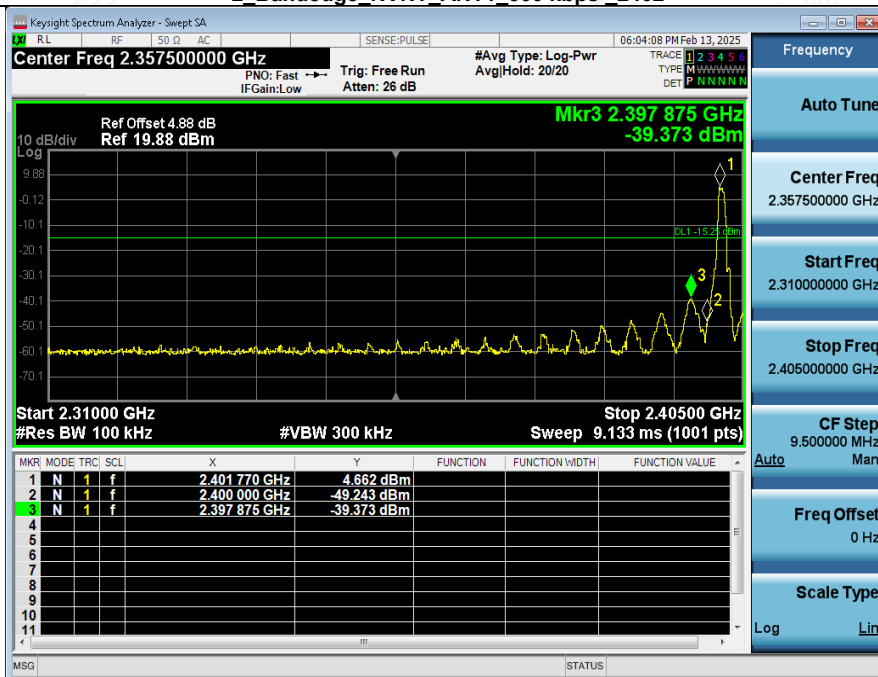
2 Bandedge_NVNT_ANT1_500 kbps_2402
