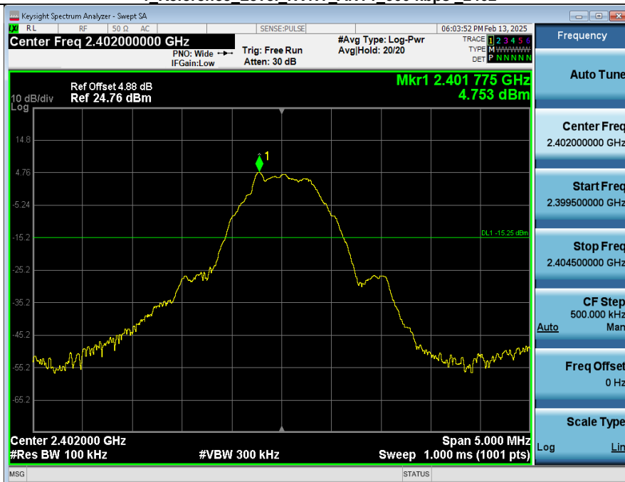
2 Bandedge_NVNT_ANT1_500 kbps_2402
