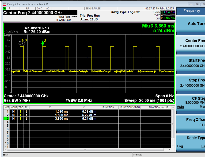
Duty_Cycle_NVNT_ANT1_1Mbps_2440
