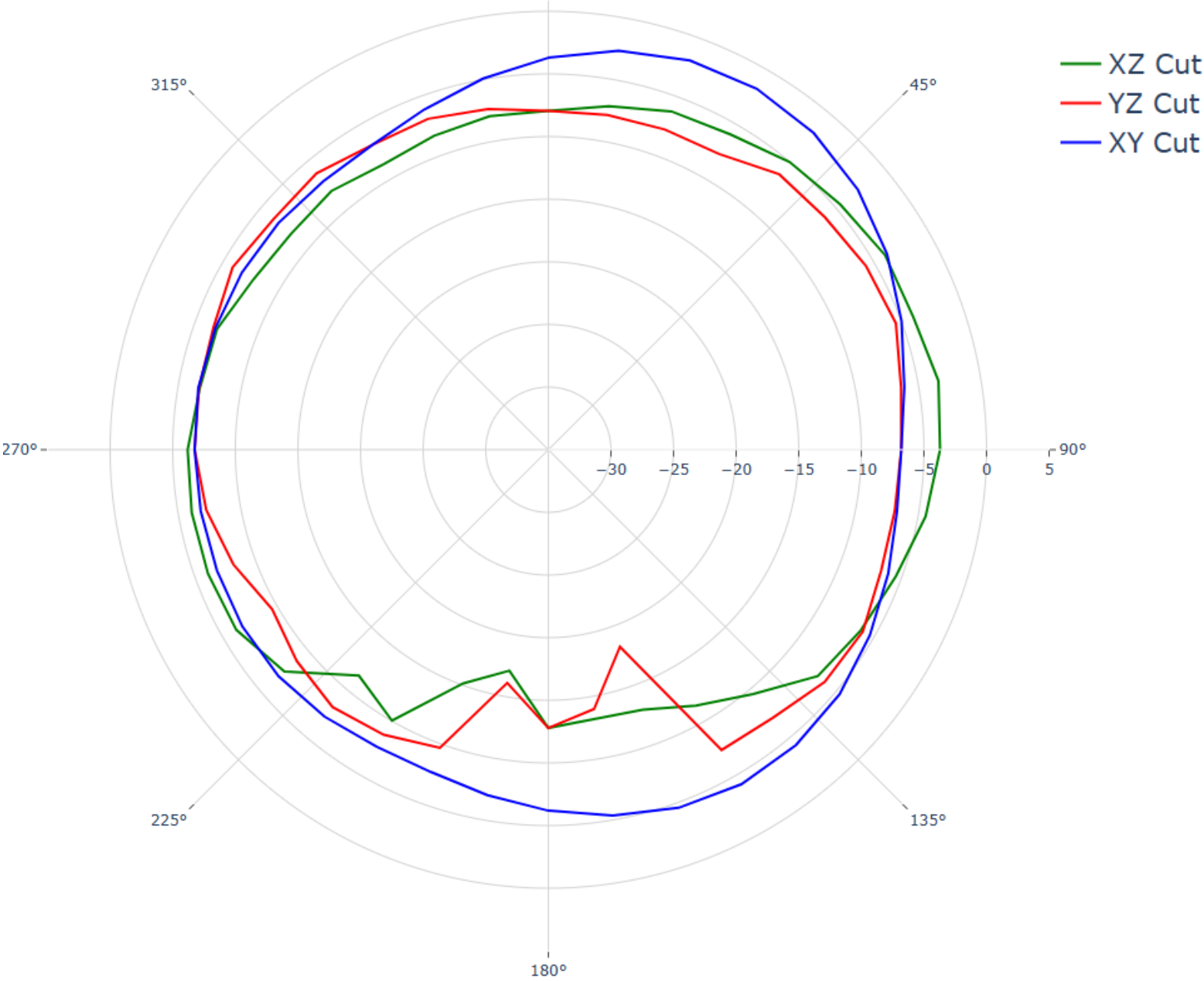
Measured Antenna Gain 2025-02-27 Device-Solutions BT Classic Antenna, Tab: Magnitude
