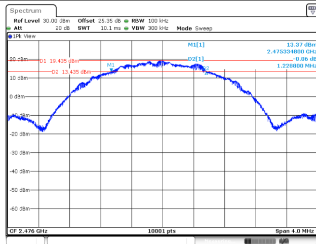
6 dB Bandwidth Plot on Channel 37
