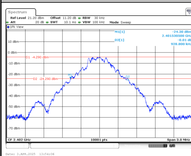
20 dB Bandwidth Plot in Channel 00
