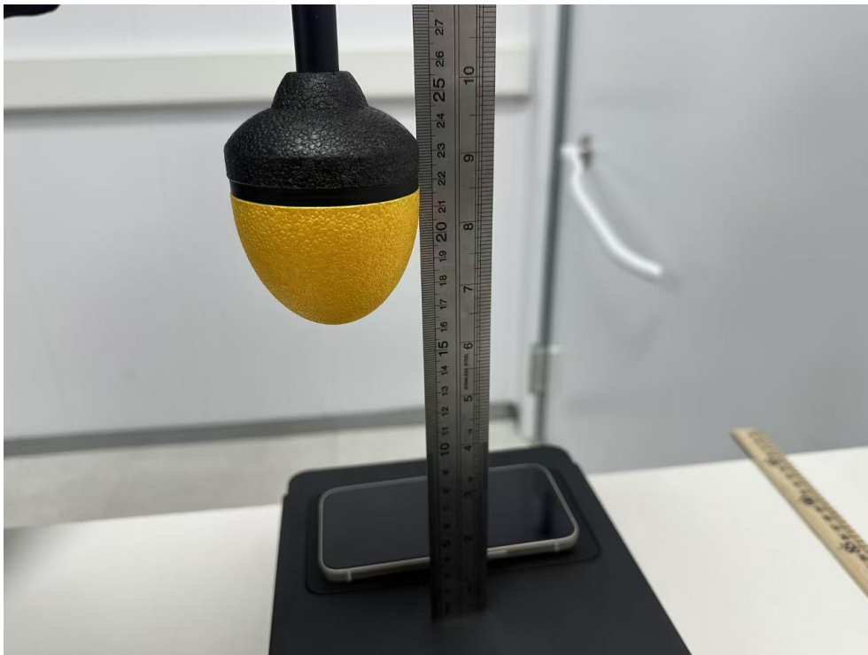
WPT Test View(position E)
