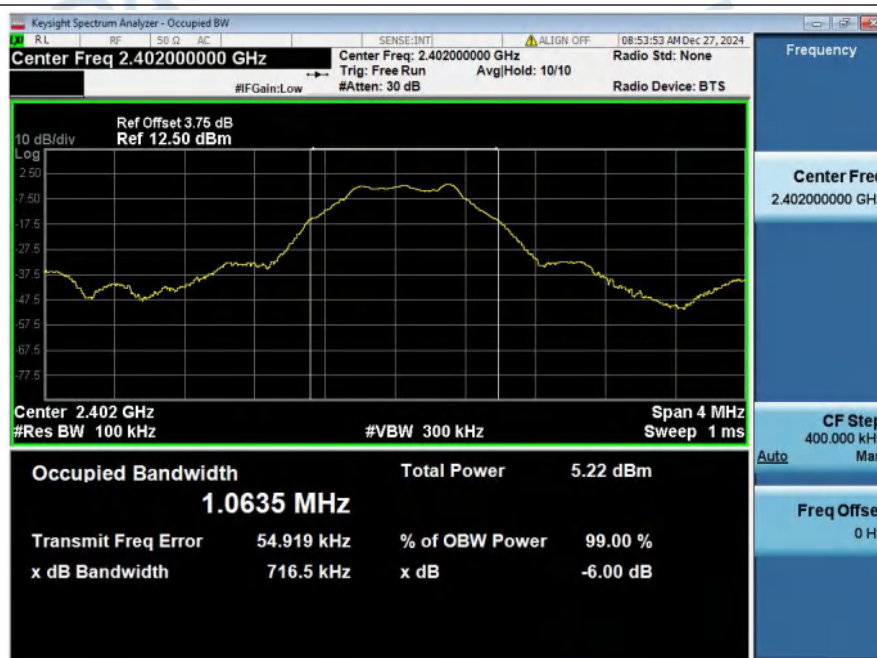
-6dB_Bandwidth_NVNT_ANT1_1Mbps_2402
