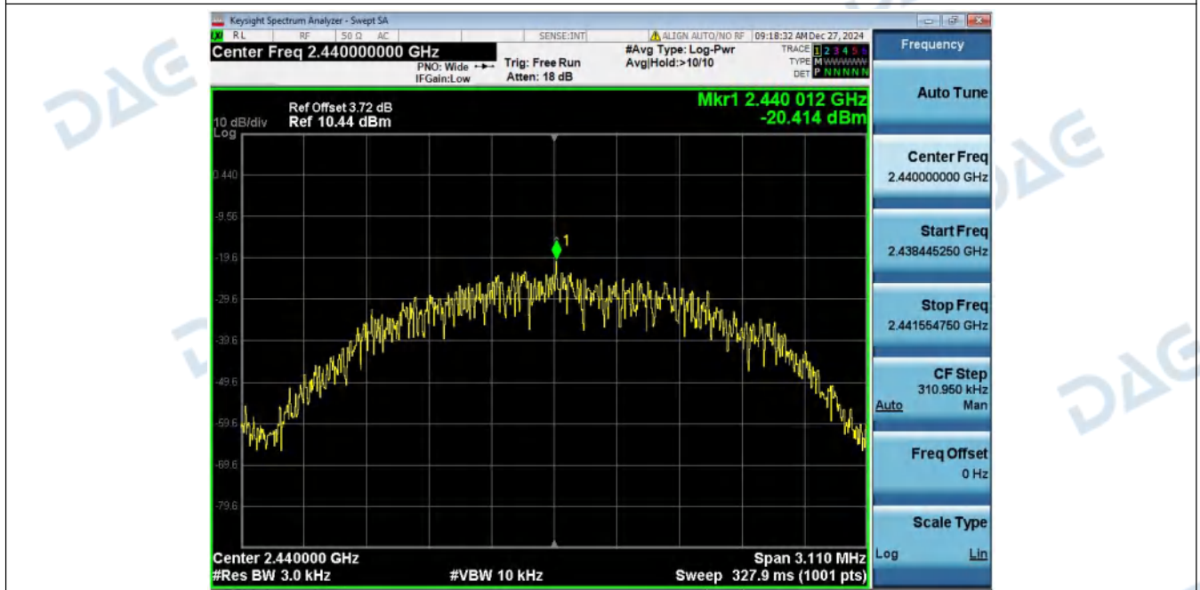
Power_Spectral_Density_NVNT_ANT1_2Mbps_2440
