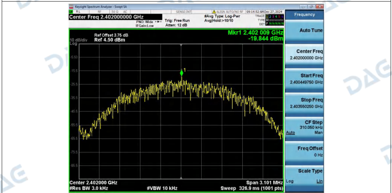
Power_Spectral_Density_NVNT_ANT1_2Mbps_2402
