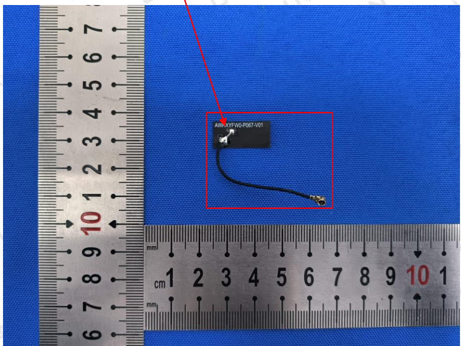
FPC Antenna
