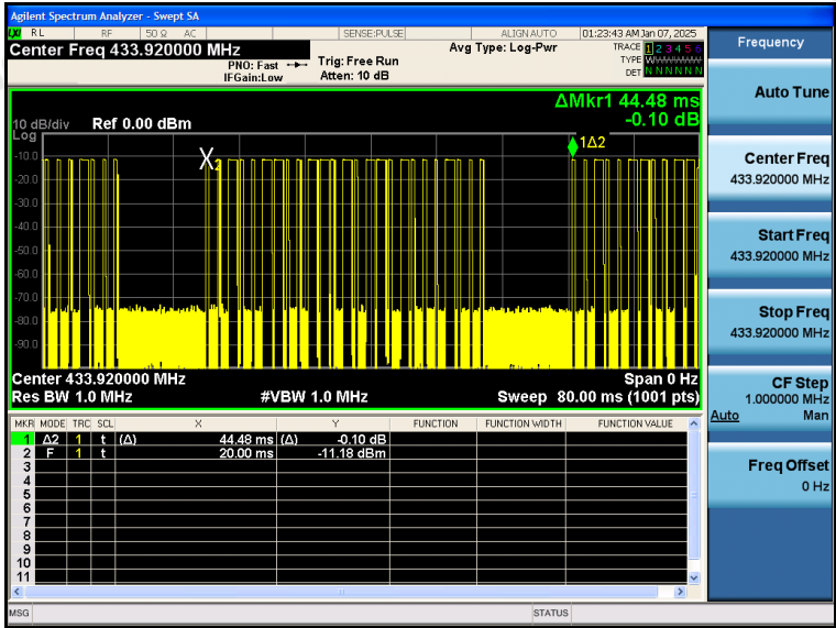
(Transmit cycle 44.48ms)
