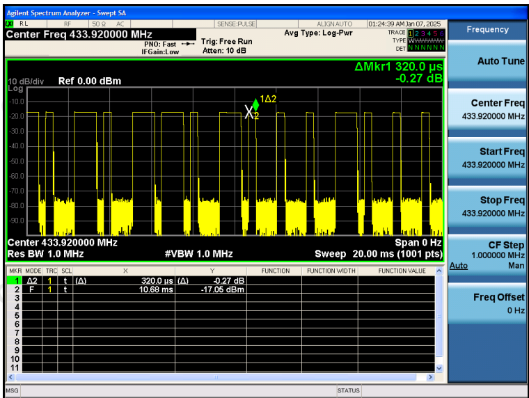
(Time per burst: 0.320 ms*15pcs)
