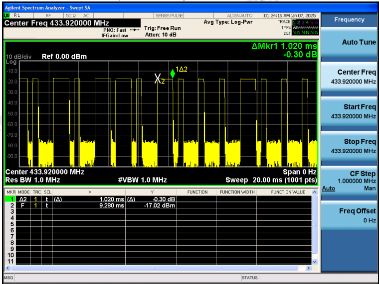
(Time per burst: 1.020ms*10pcs)
