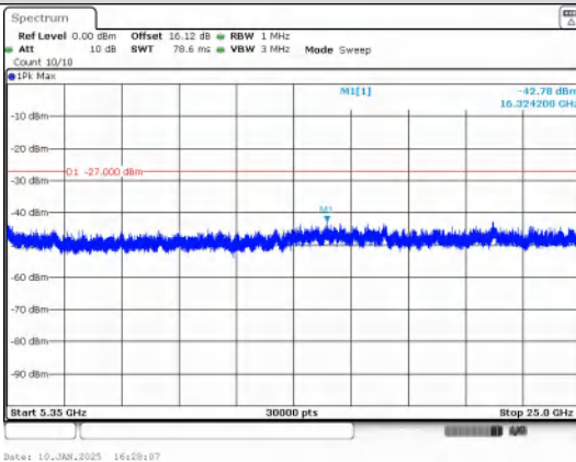
Spurious Emission:5350~25000.0 MHz IEEE 802.11a_Channel 60_20MHz_Antenna 0
