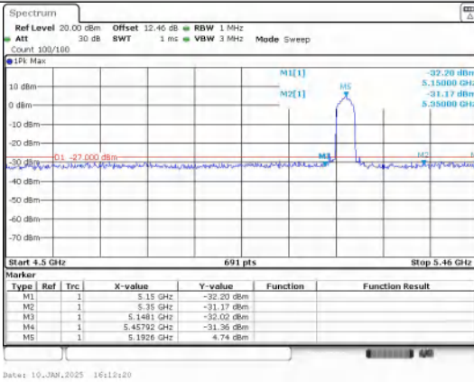
Out Of Band Emission IEEE 802.11n_Channel 38_40MHz_Antenna 0
