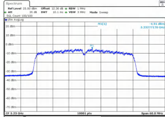
IEEE 802.11n_Channel 46_40MHz_Antenna 0
