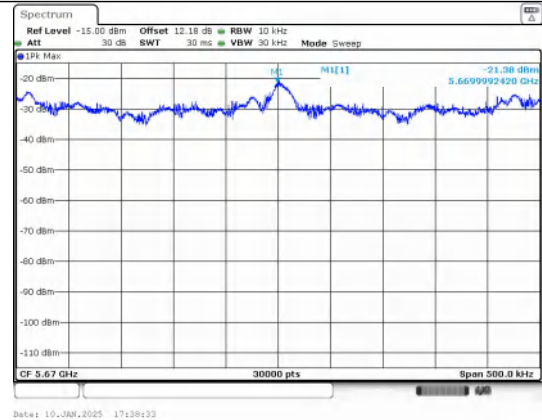
NT/NV_Antenna 0 IEEE 802.11n_Channel 134_40MHz
