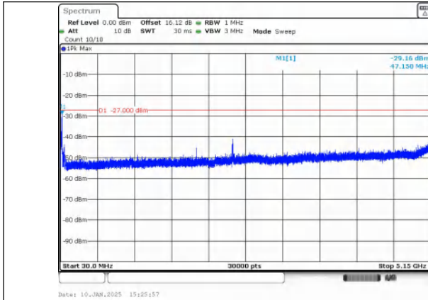
Spurious Emission:30.0~5150 MHz IEEE 802.11a_Channel 40_20MHz_Antenna 0
