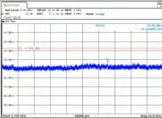
Out Of Band Emission IEEE 802.11n_Channel 110_40MHz_Antenna 0
