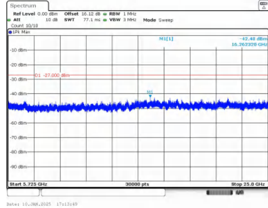
Spurious Emission:5725~25000.0 MHz IEEE 802.11n_Channel 100_20MHz_Antenna 0
