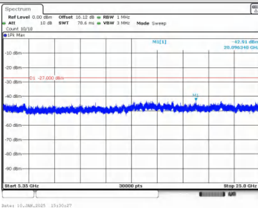
Spurious Emission:5350~25000.0 MHz IEEE 802.11a_Channel 48_20MHz_Antenna 0
