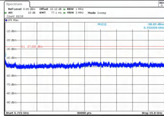
Spurious Emission:5725~25000.0 MHz IEEE 802.11n_Channel 140_20MHz_Antenna 0
