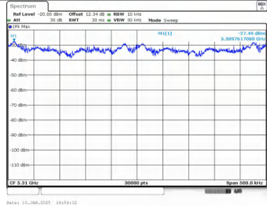
NT/NV_Antenna 0 IEEE 802.11n_Channel 62_40MHz
