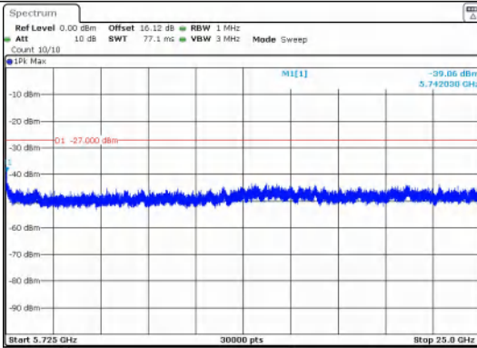
Out Of Band Emission IEEE 802.11a_Channel 140_20MHz_Antenna 0
