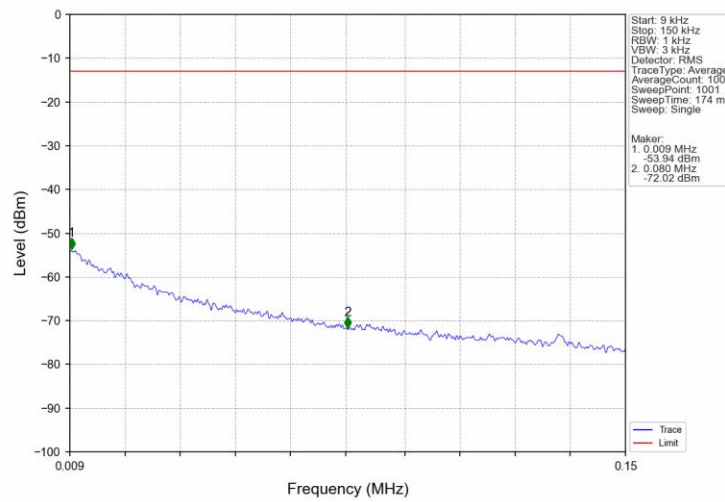
Band2_1.4MHz_16QAM_HCH_1909.3MHz_RB_1_0_NTNV
