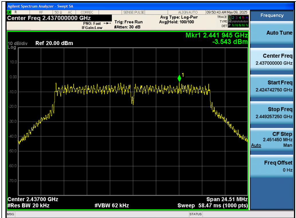
Test_Graph_802.11g_ANT1_2437_6Mbps_PSD
