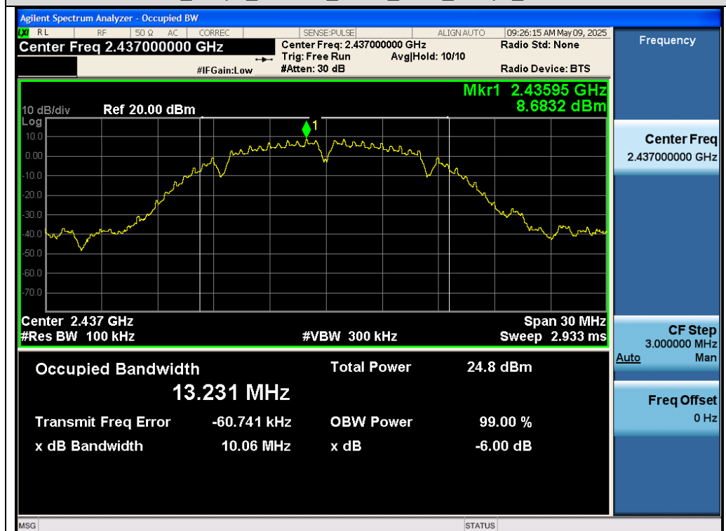
Test_Graph_802.11b_ANT1_2437_1Mbps_DTSPW
