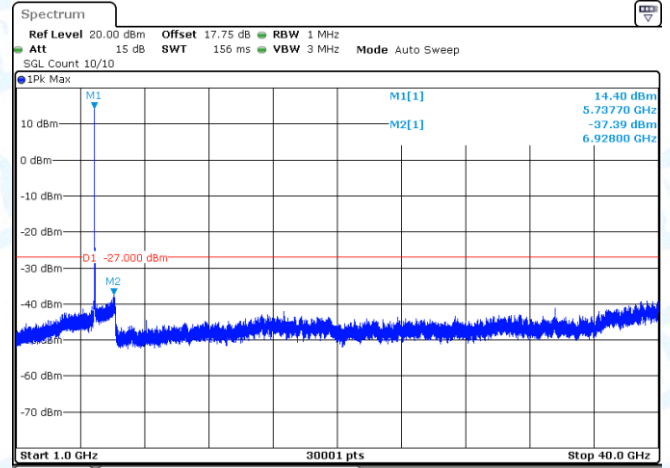
11AX20SISO-Ant1-5745-1000~40000-PASS
