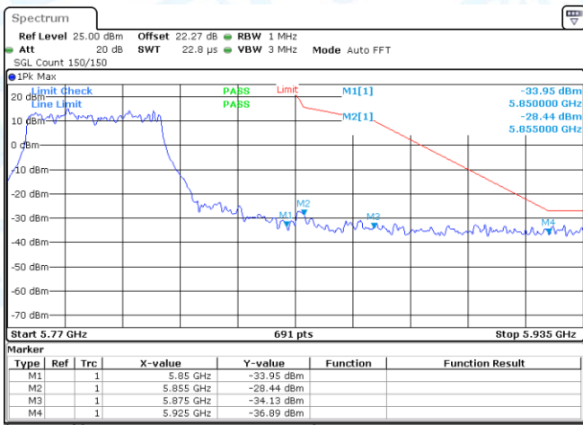
11AX40SISO-Ant1-5755-PASS
