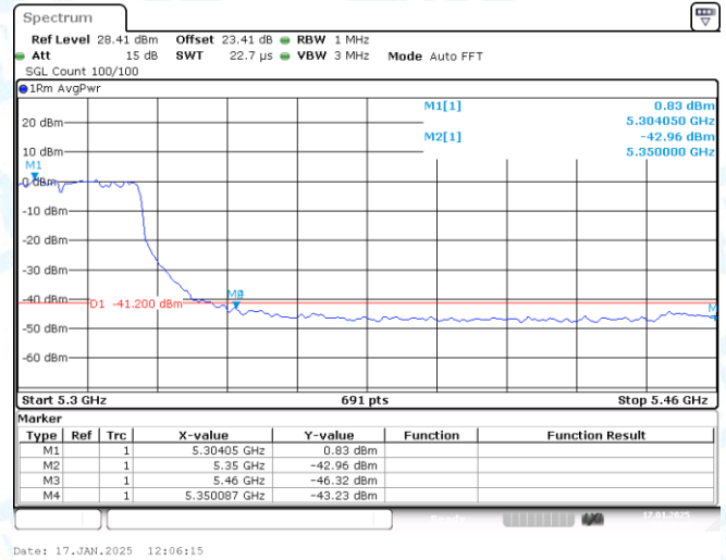
11AC40SISO-Ant1-5310-PASS
