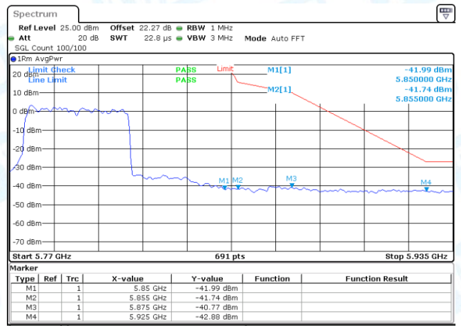
11AX40SISO-Ant1-5755-PASS
