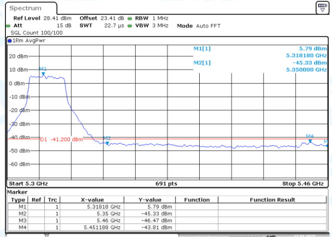
11N20SISO-Ant1-5320-PASS
