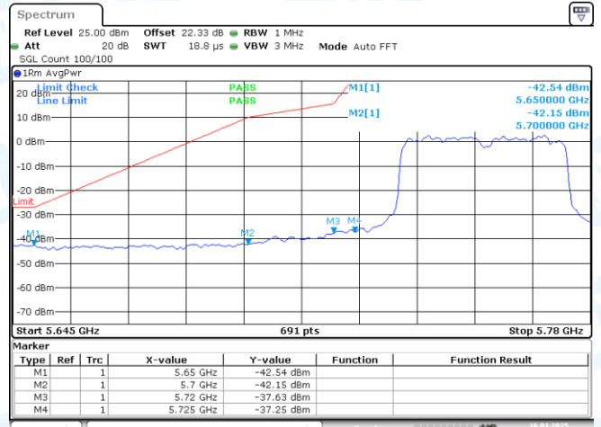
11AX40SISO-Ant1-5755-PASS
