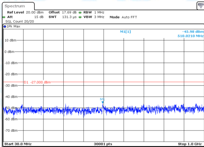
11AX40SISO-Ant1-5755-30~1000-PASS
