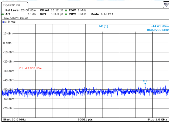
11AX40SISO-Ant1-5510-30~1000-PASS
