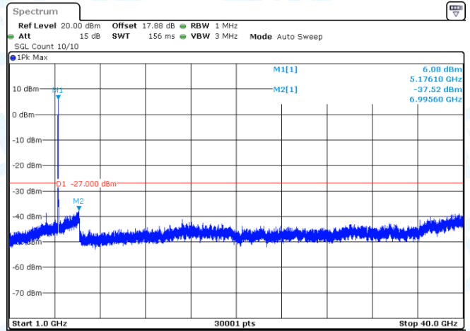
11AX40SISO-Ant1-5190-1000~40000-PASS
