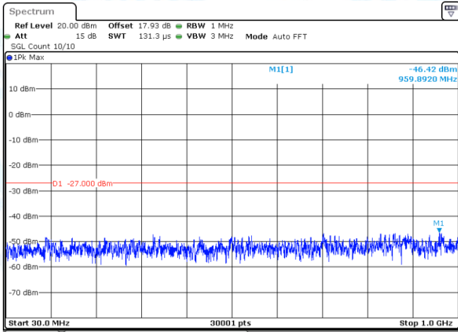
11AX40SISO-Ant1-5310-30~1000-PASS
