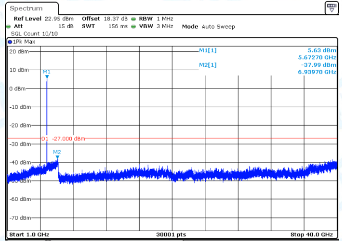
11AX40SISO-Ant1-5670-1000~40000-PASS
