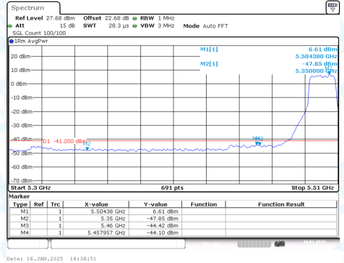
11A-Ant1-5500-PASS
