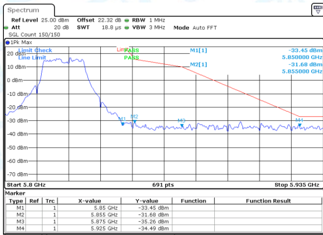
11AC20SISO-Ant1-5745-PASS
