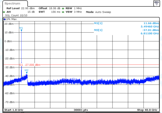
11AX20SISO-Ant1-5500-1000~40000-PASS
