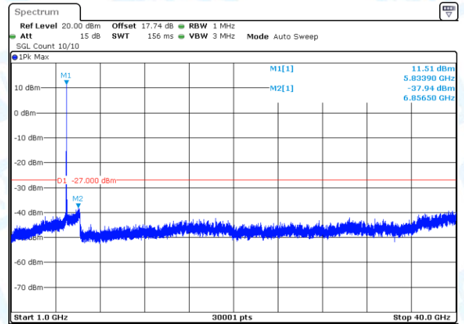
11AX20SISO-Ant1-5785-1000~40000-PASS
