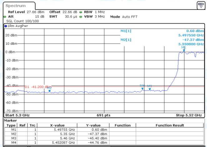
11N40SISO-Ant1-5510-PASS
