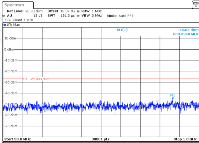
11AX40SISO-Ant1-5670-30~1000-PASS
