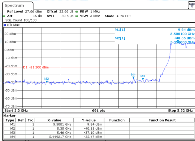
11N40SISO-Ant1-5510-PASS
