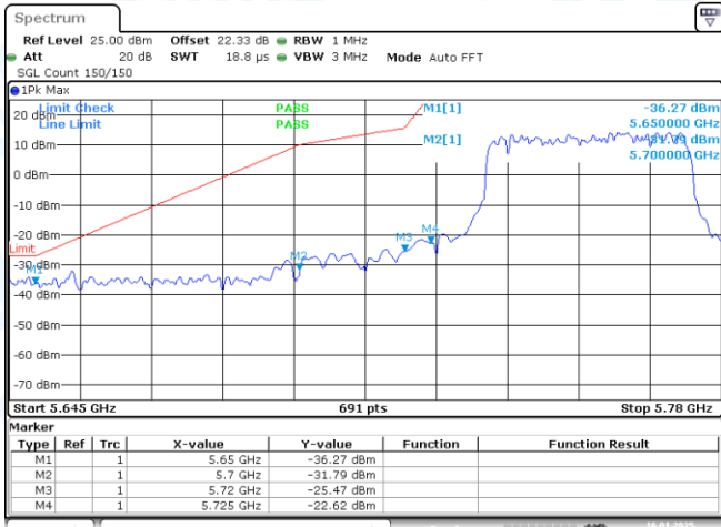
11AX40SISO-Ant1-5755-PASS
