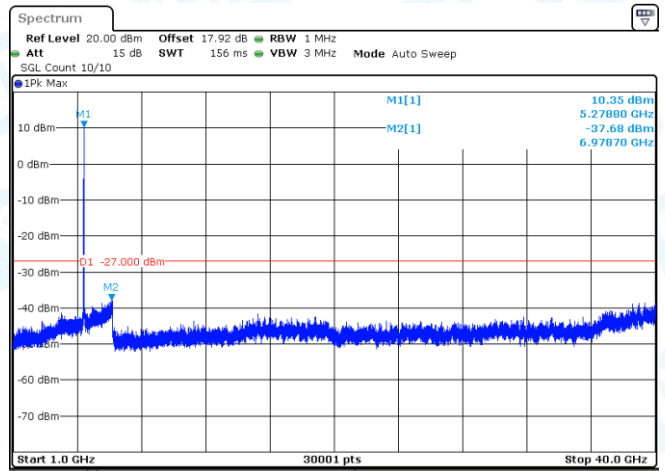
11N20SISO-Ant1-5260-1000~40000-PASS
