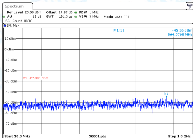
11A-Ant1-5260-30~1000-PASS
