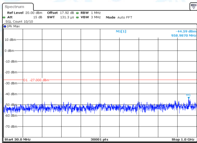
11A-Ant1-5260-30~1000-PASS
