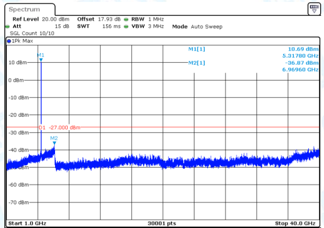
11N20SISO-Ant1-5280-1000~40000-PASS
