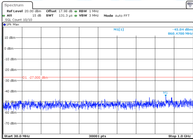
11N20SISO-Ant1-5200-30~1000-PASS
