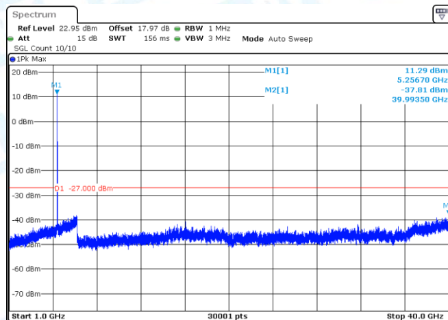
11A-Ant1-5260-1000~40000-PASS
