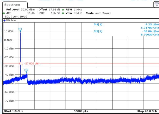
11A-Ant1-5280-1000~40000-PASS
