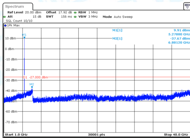
11A-Ant1-5260-1000~40000-PASS
