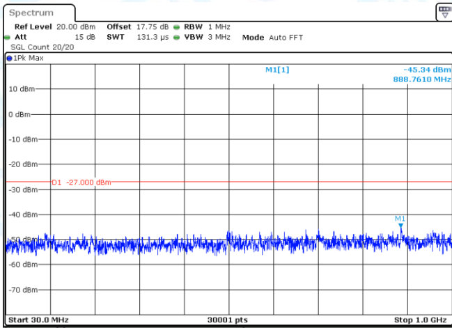
11AC40SISO-Ant1-5670-30~1000-PASS
