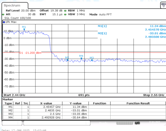
11AX40SISO-Ant1-2452-PASS
