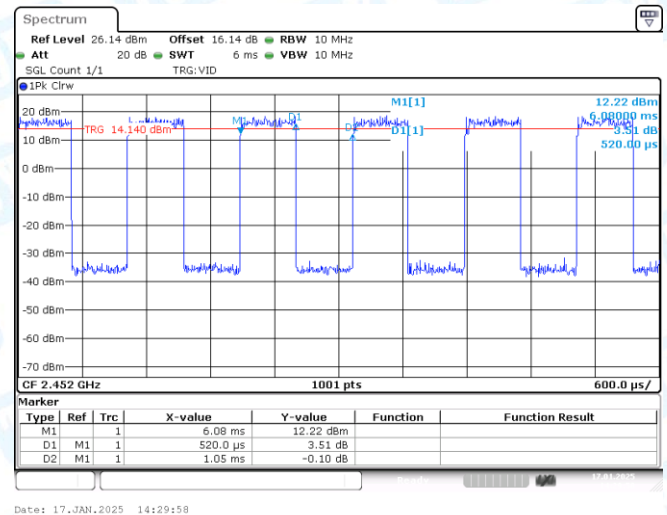
NTNV-11N40SISO-Ant1-2452
