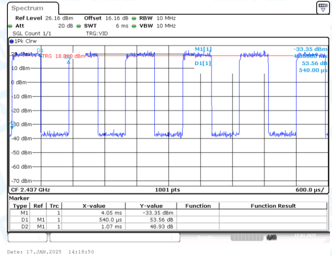
NTNV-11N20SISO-Ant1-2437
