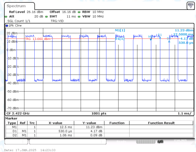
NTNV-11N40SISO-Ant1-2422
