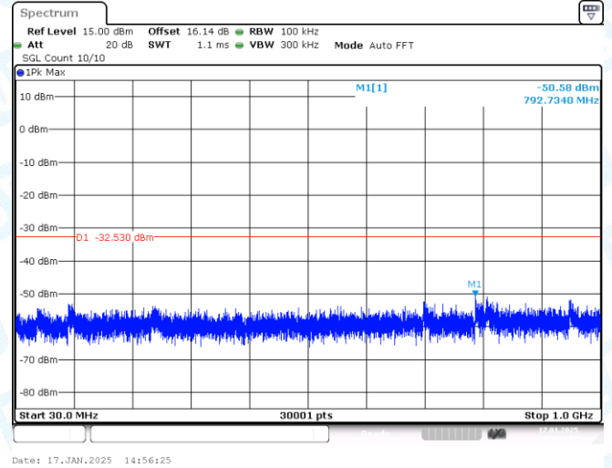
11AX20SISO-Ant1-2462-30~1000-PASS
