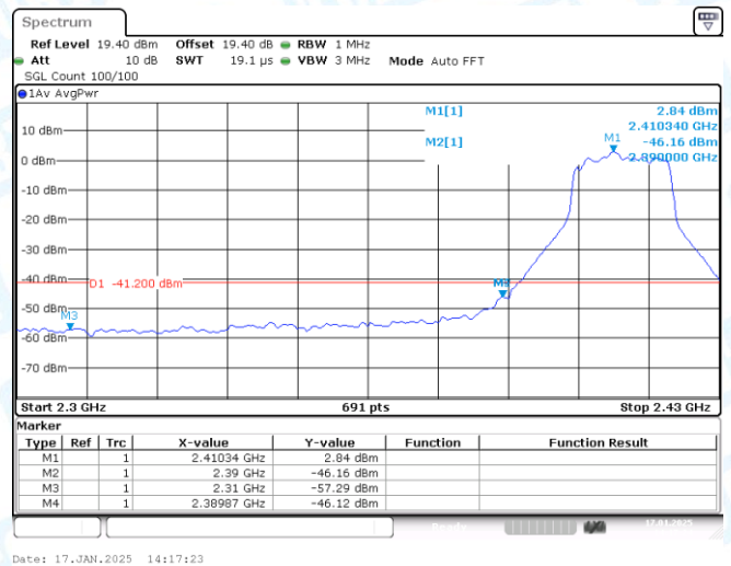
11N20SISO-Ant1-2412-PASS
