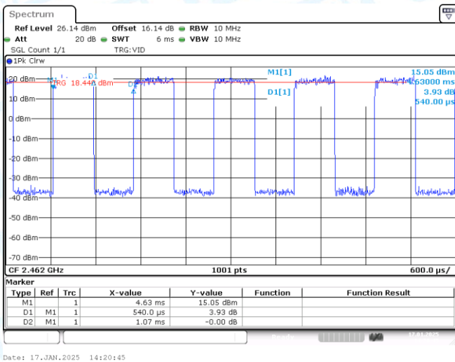
NTNV-11N20SISO-Ant1-2462
