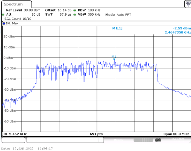
11AX20SISO-Ant1-2462-0~Reference-PASS
