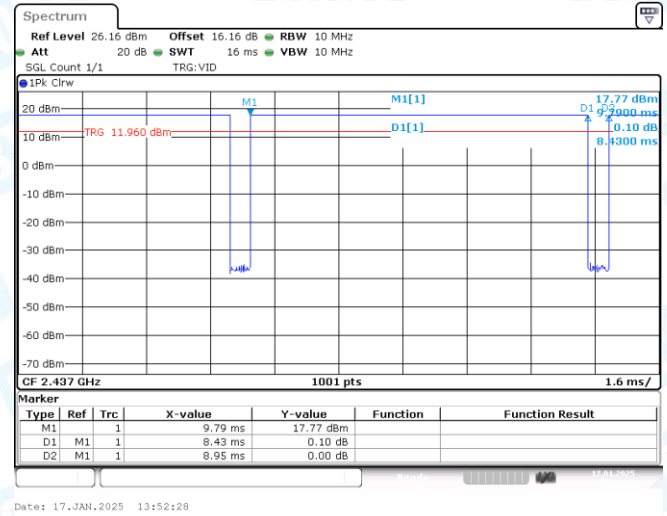
NTNV-11B-Ant1-2437
