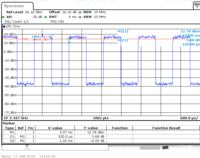
NTNV-11N40SISO-Ant1-2437
