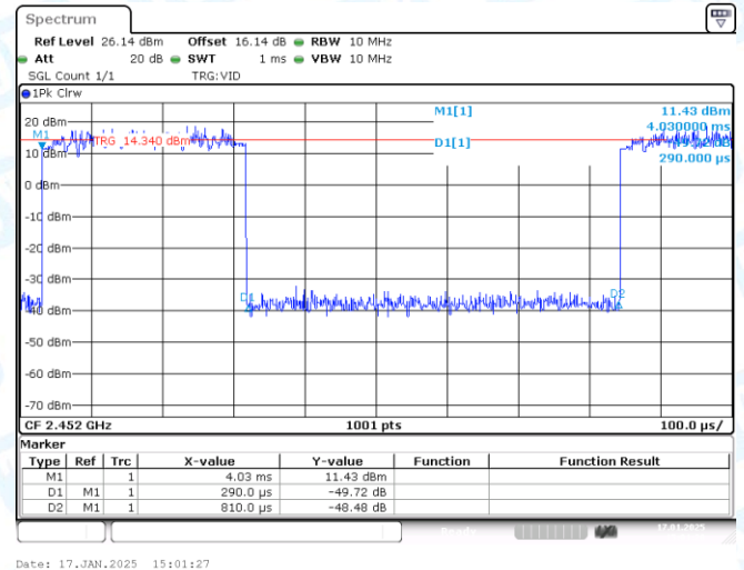
NTNV-11AX40SISO-Ant1-2452
