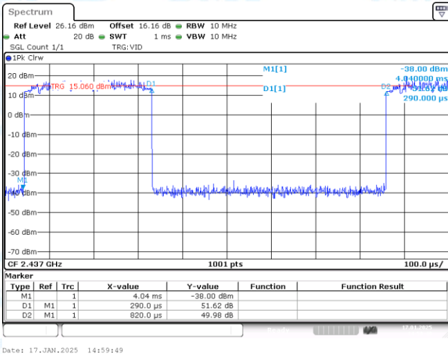
NTNV-11AX40SISO-Ant1-2437
