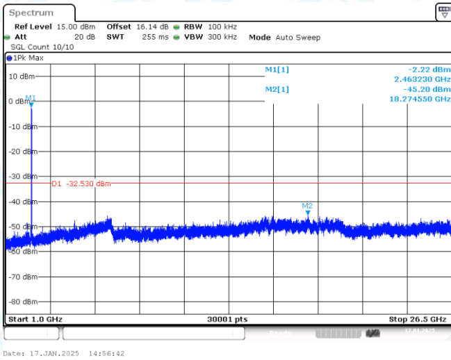
11AX20SISO-Ant1-2462-1000~26500-PASS
