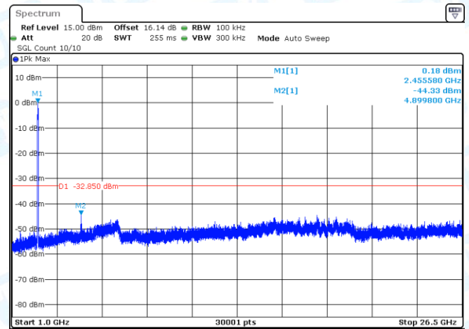
11AX40SISO-Ant1-2452-0~Reference-PASS
