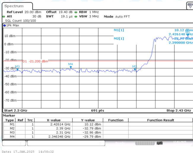
11AX40SISO-Ant1-2422-PASS
