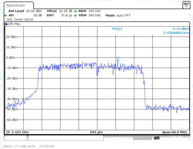
11AX40SISO-Ant1-2422-0~Reference-PASS
