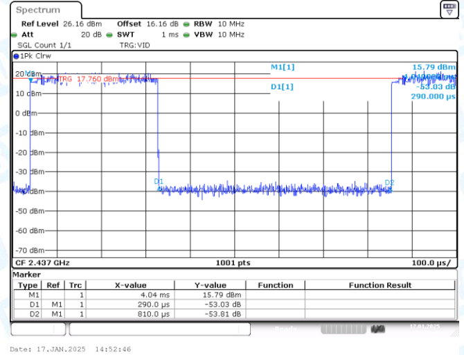
NTNV-11AX20SISO-Ant1-2437
