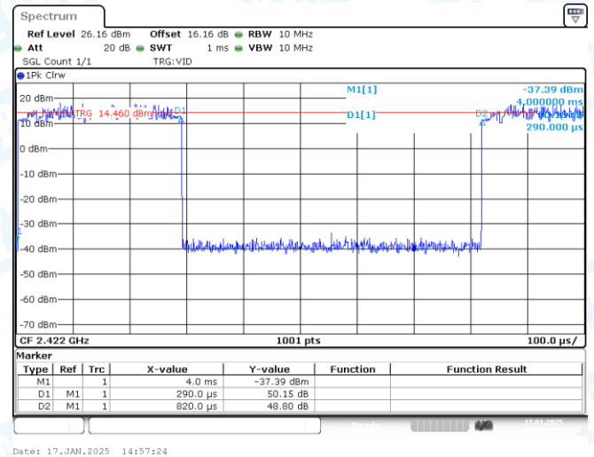
NTNV-11AX40SISO-Ant1-2422
