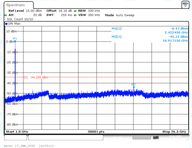
11AX40SISO-Ant1-2422-1000~26500-PASS
