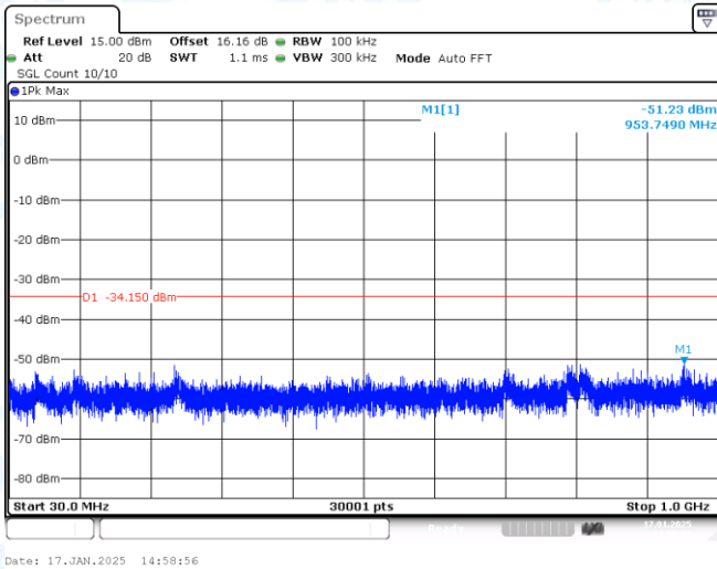
11AX40SISO-Ant1-2422-30~1000-PASS
