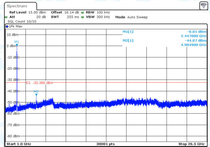
11N40SISO-Ant1-2452-0~Reference-PASS
