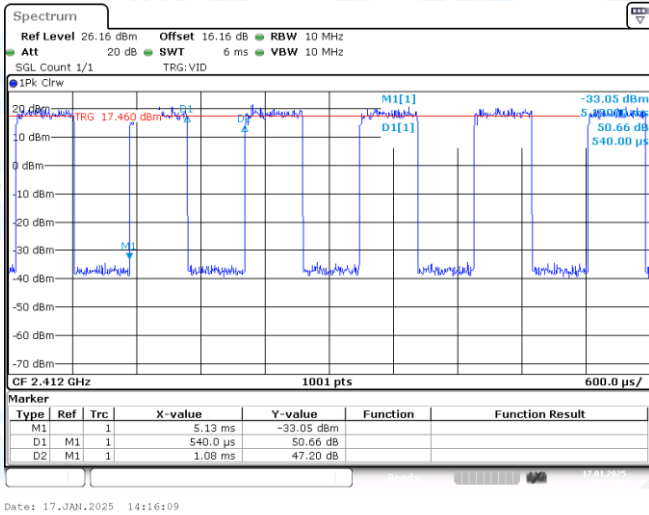
NTNV-11N20SISO-Ant1-2412
