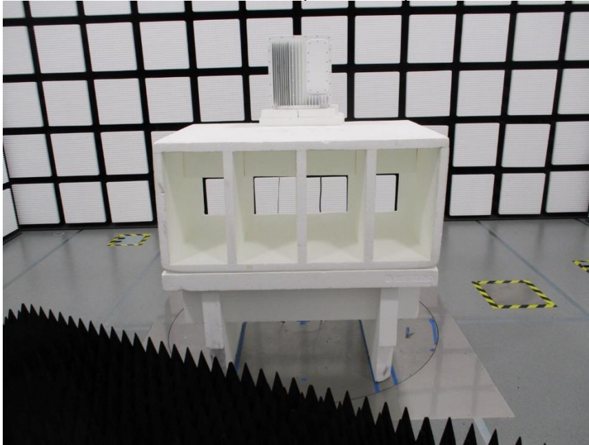
RADIATED SPURIOUS PHOTO (1 - 18 GHz)
