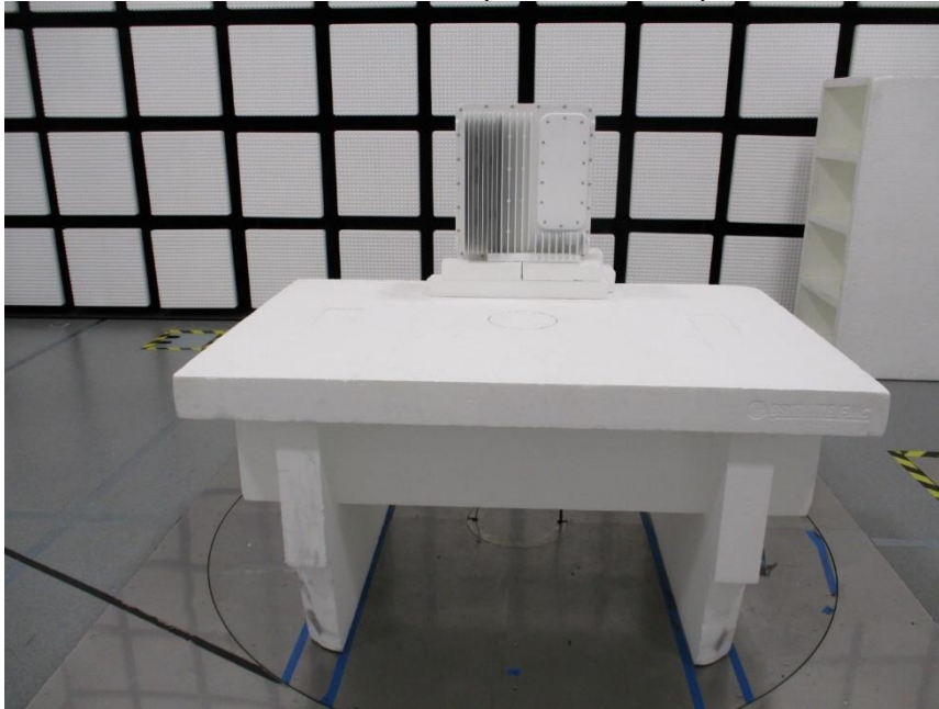
RADIATED SPURIOUS PHOTO (30 - 1000 MHz)
