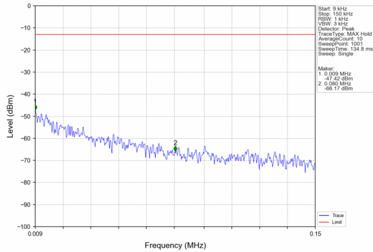
Band66_3MHz_QPSK_HCH_1778.5MHz_RB_1_0_NTNV
