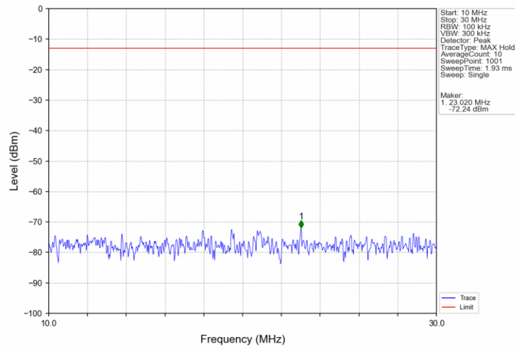
Band12_3MHz_16QAM_MCH_707.5MHz_RB_1_0_NTNV
