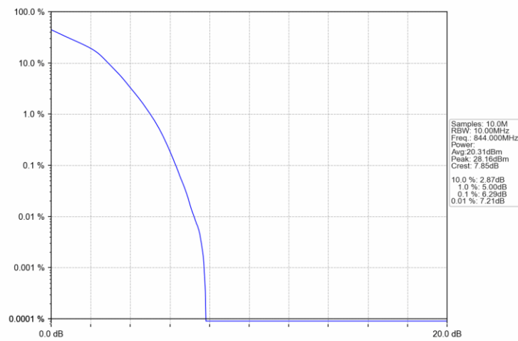
Band5_10MHz_16QAM_HCH_844MHz_RB_50_0_NTNV
