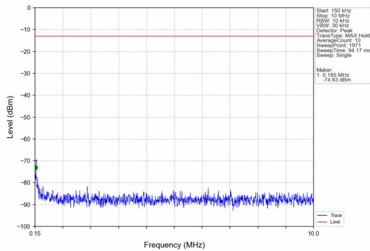
Band4_3MHz_16QAM_MCH_1732.5MHz_RB_1_0_NTNV
