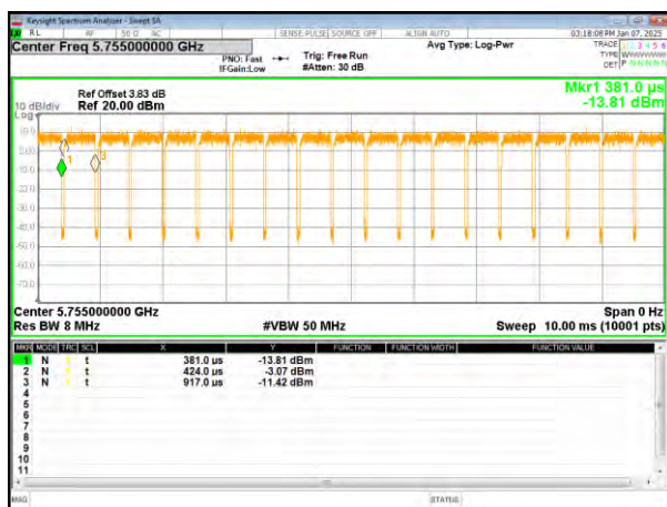
(802.11ac40) plot
