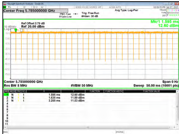
(802.11ac20) plot
