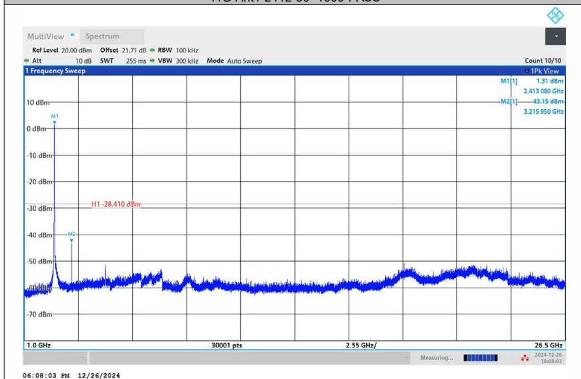
11G-Ant1-2412-1000~26500-PASS
