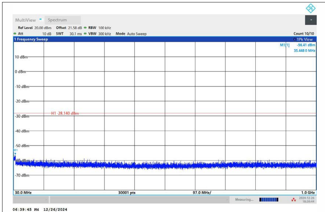
11AX20SISO-Ant1-2462-30~1000-PASS
