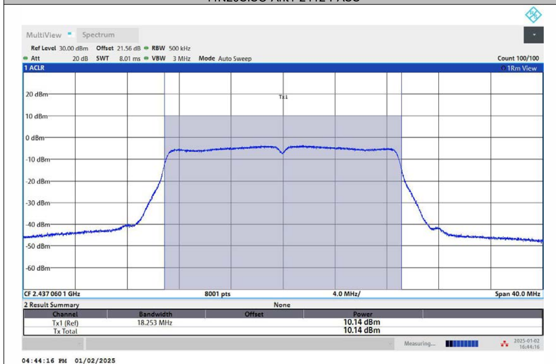
11N20SISO-Ant1-2437-PASS
