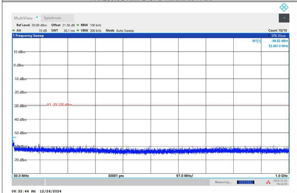
11AX20SISO-Ant1-2437-30~1000-PASS
