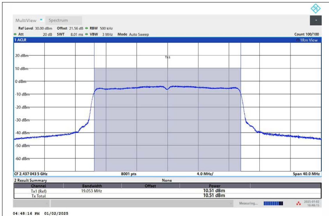
11AX20SISO-Ant1-2437-PASS
