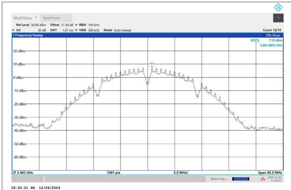
11B-Ant1-2462-0~Reference-PASS
