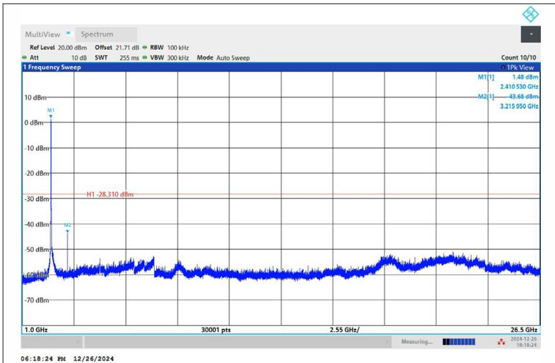
11N20SISO-Ant1-2412-1000~26500-PASS
