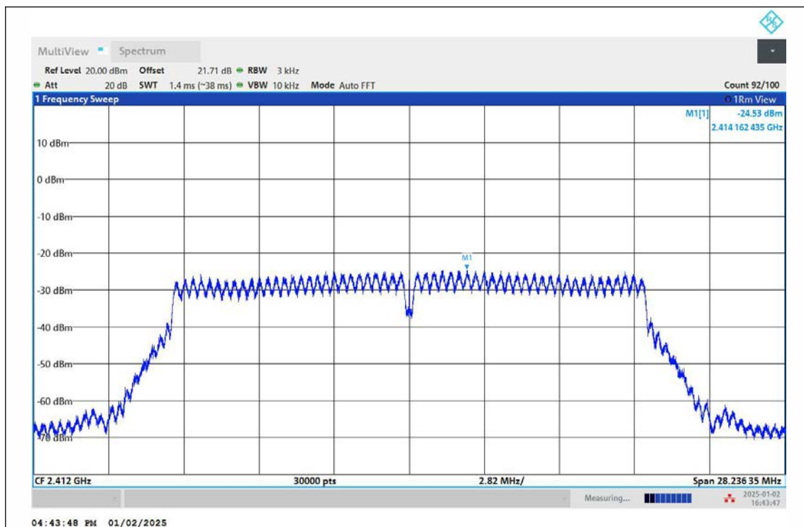
11N20SISO-Ant1-2412-PASS
