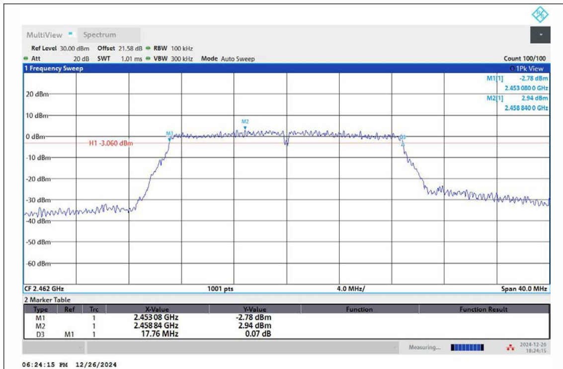
11N20SISO-Ant1-2462-PASS
