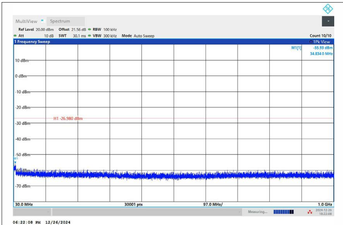
11N20SISO-Ant1-2437-30~1000-PASS
