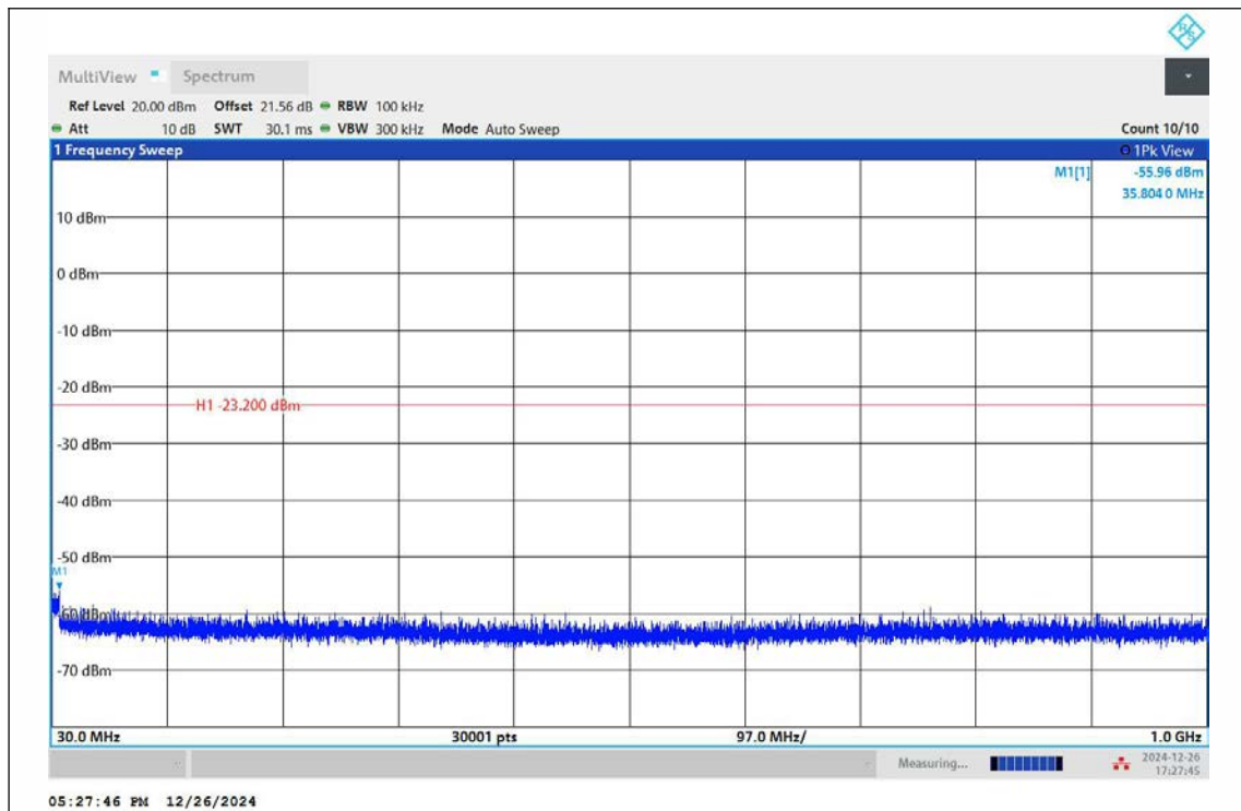
11B-Ant1-2437-30~1000-PASS
