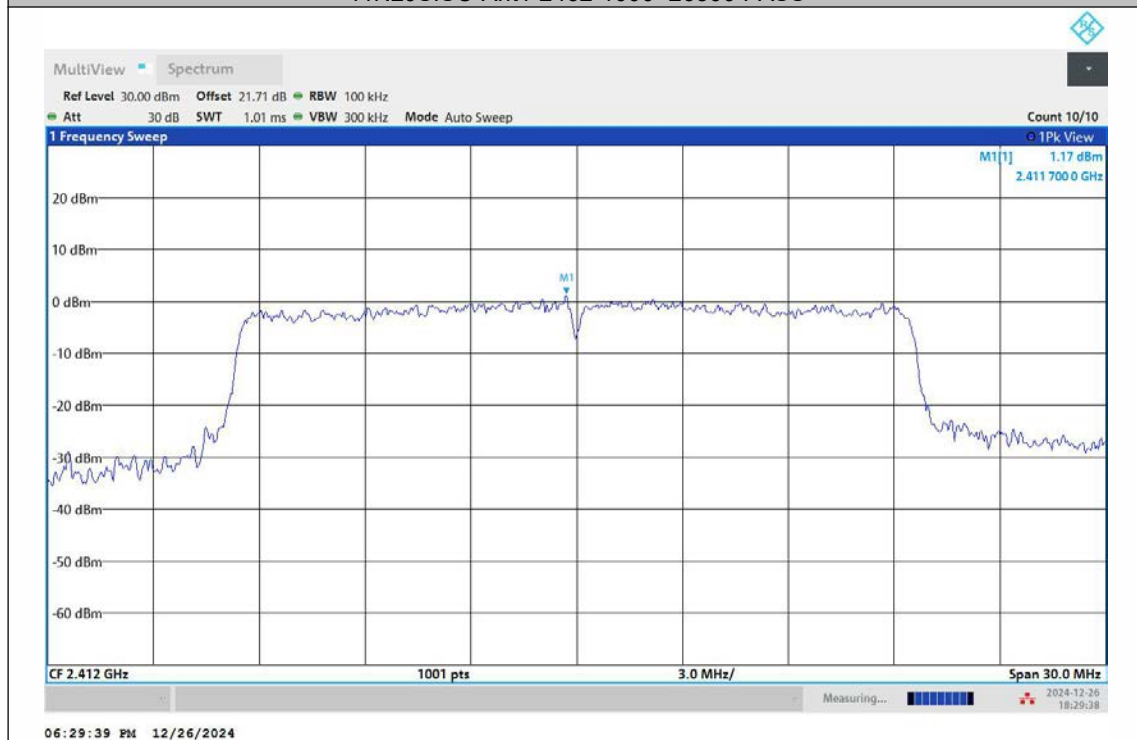
11AX20SISO-Ant1-2412-0~Reference-PASS
