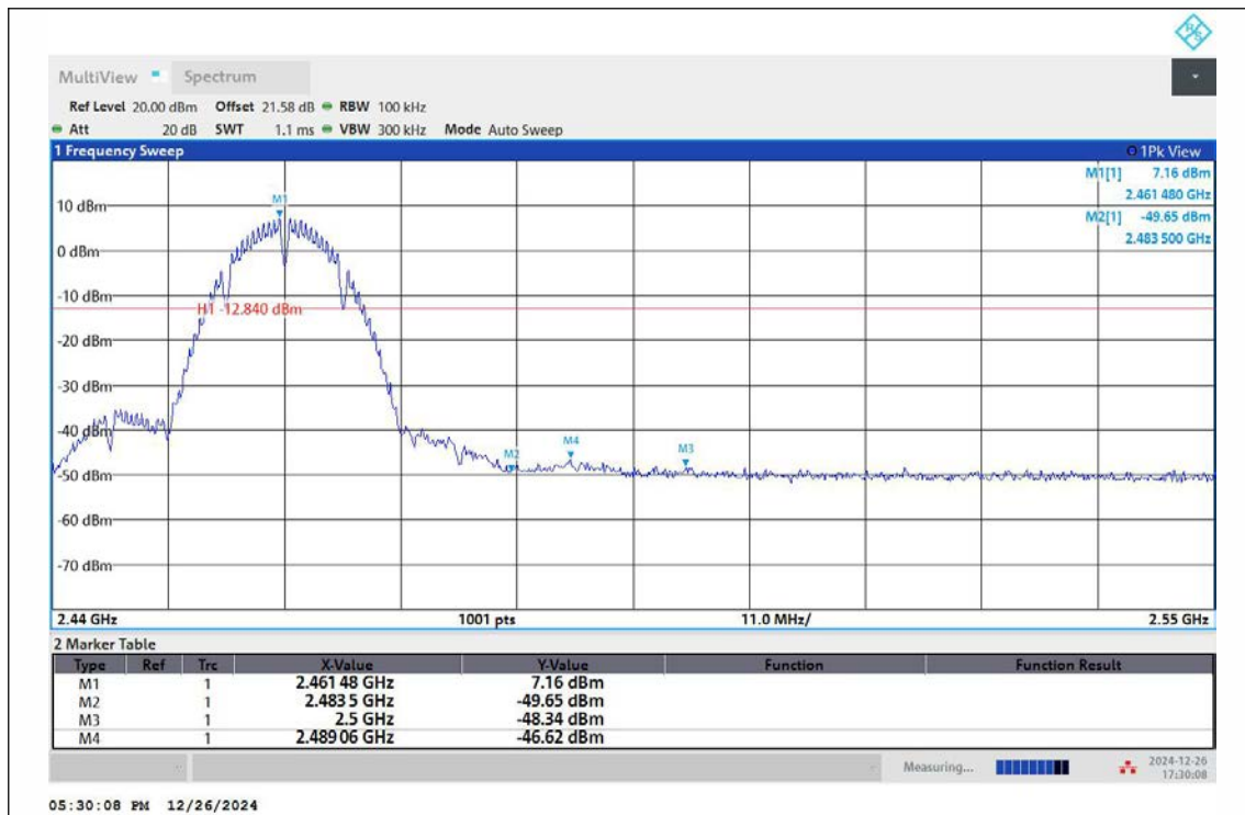
11B-Ant1-2462-PASS
