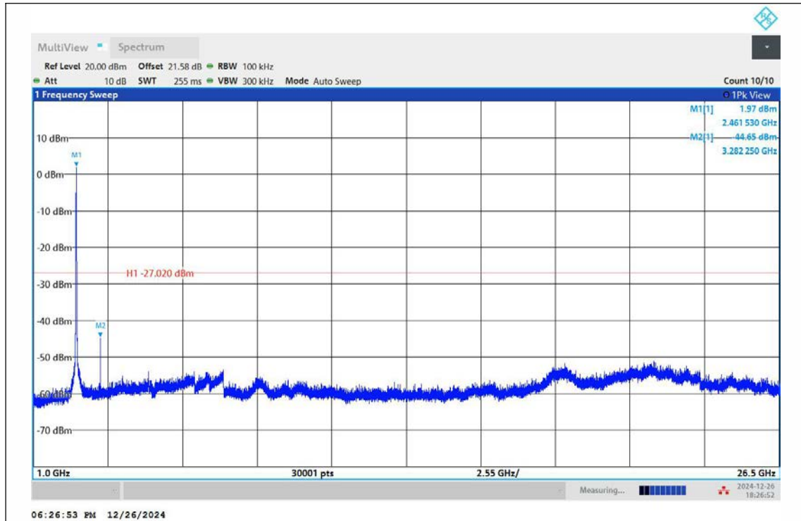
11N20SISO-Ant1-2462-1000~26500-PASS
