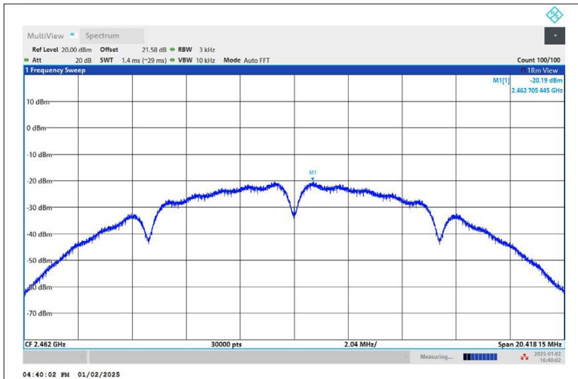
11B-Ant1-2462-PASS
