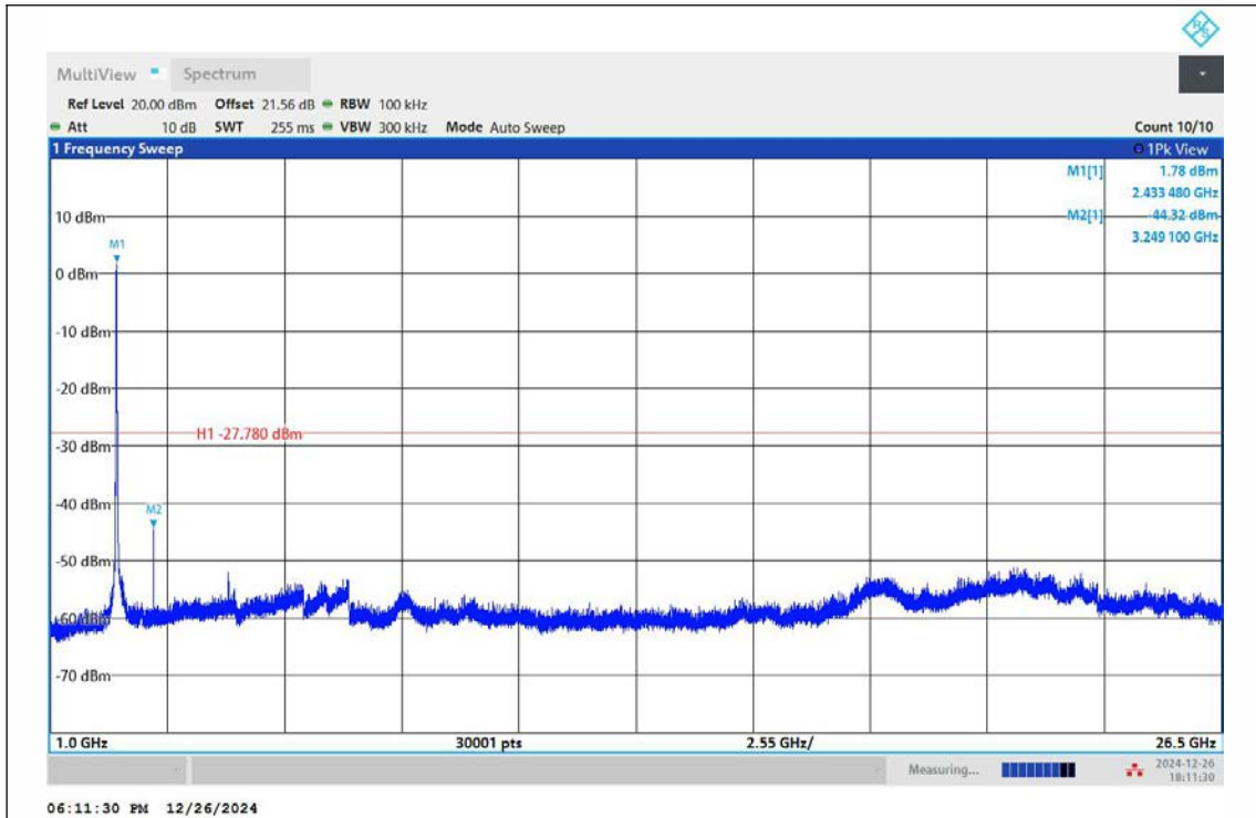
11G-Ant1-2437-1000~26500-PASS
