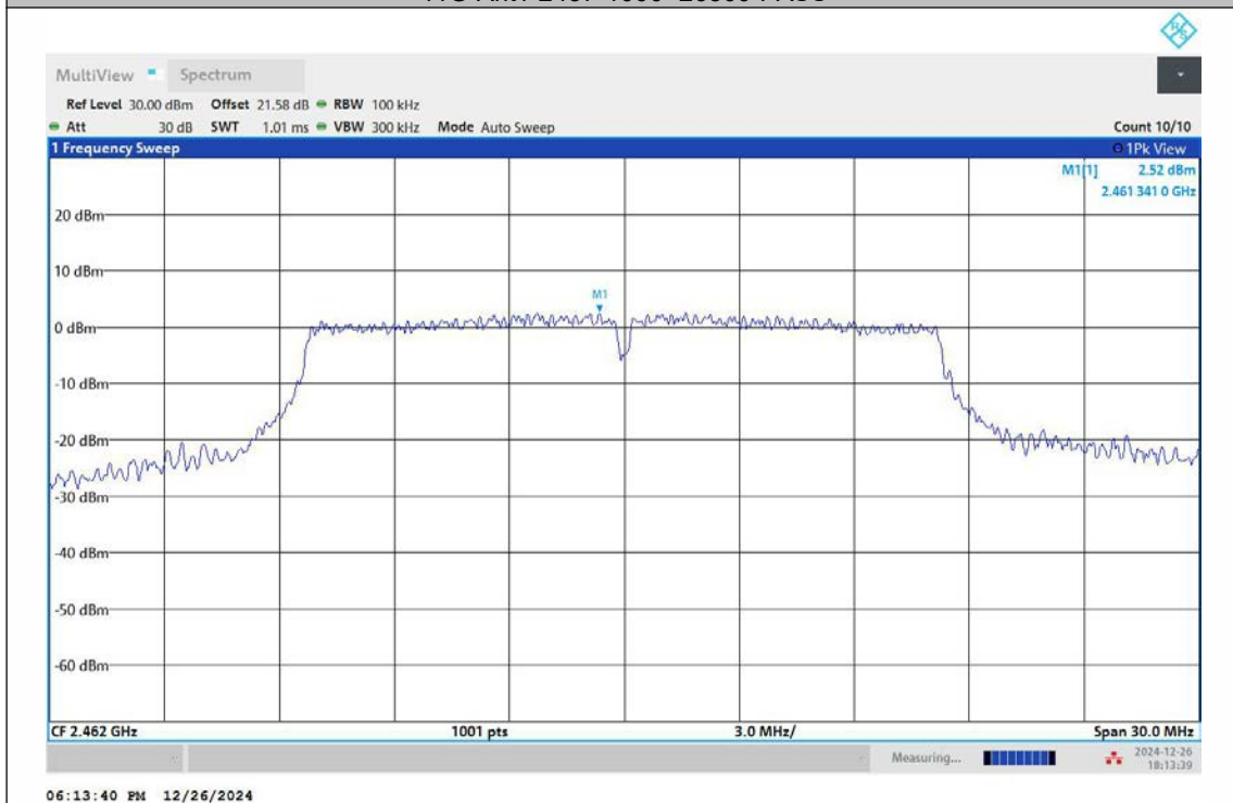
11G-Ant1-2462-0~Reference-PASS
