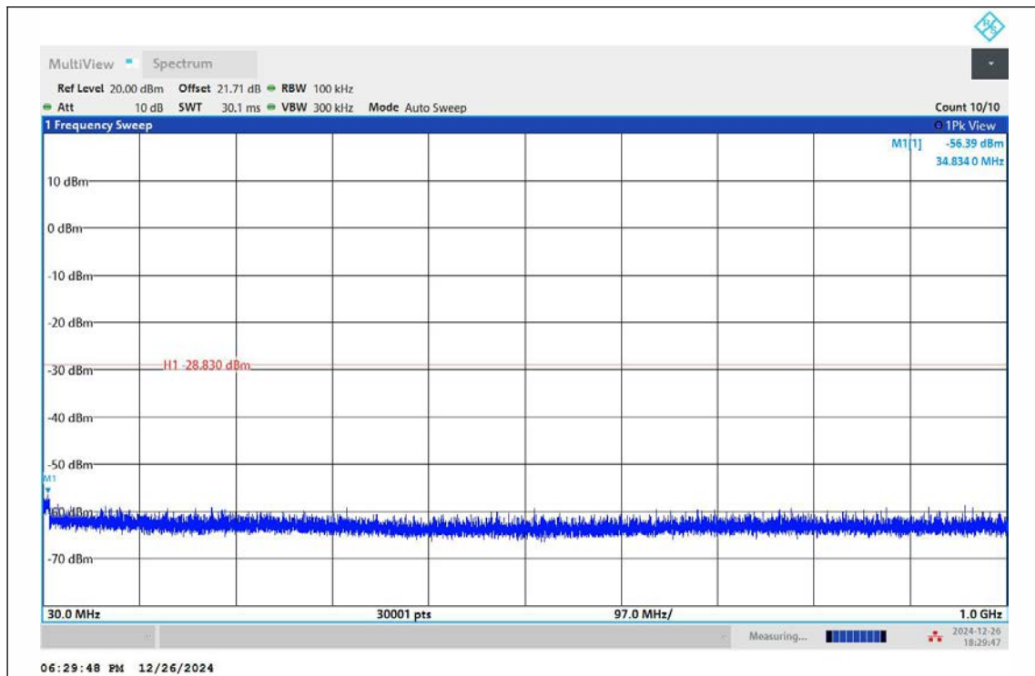
11AX20SISO-Ant1-2412-30~1000-PASS
