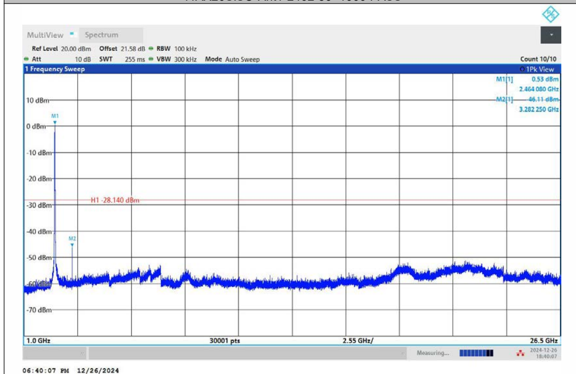
11AX20SISO-Ant1-2462-1000~26500-PASS
