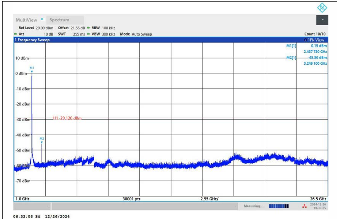
11AX20SISO-Ant1-2437-1000~26500-PASS
