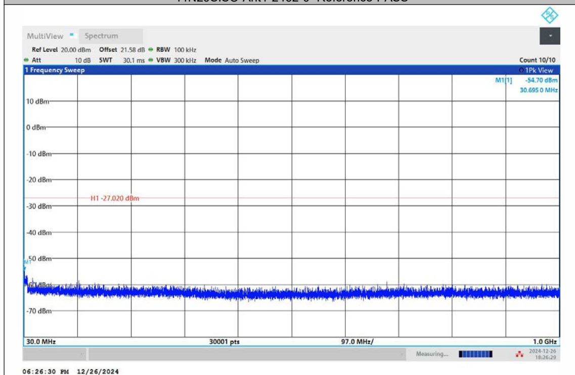
11N20SISO-Ant1-2462-30~1000-PASS
