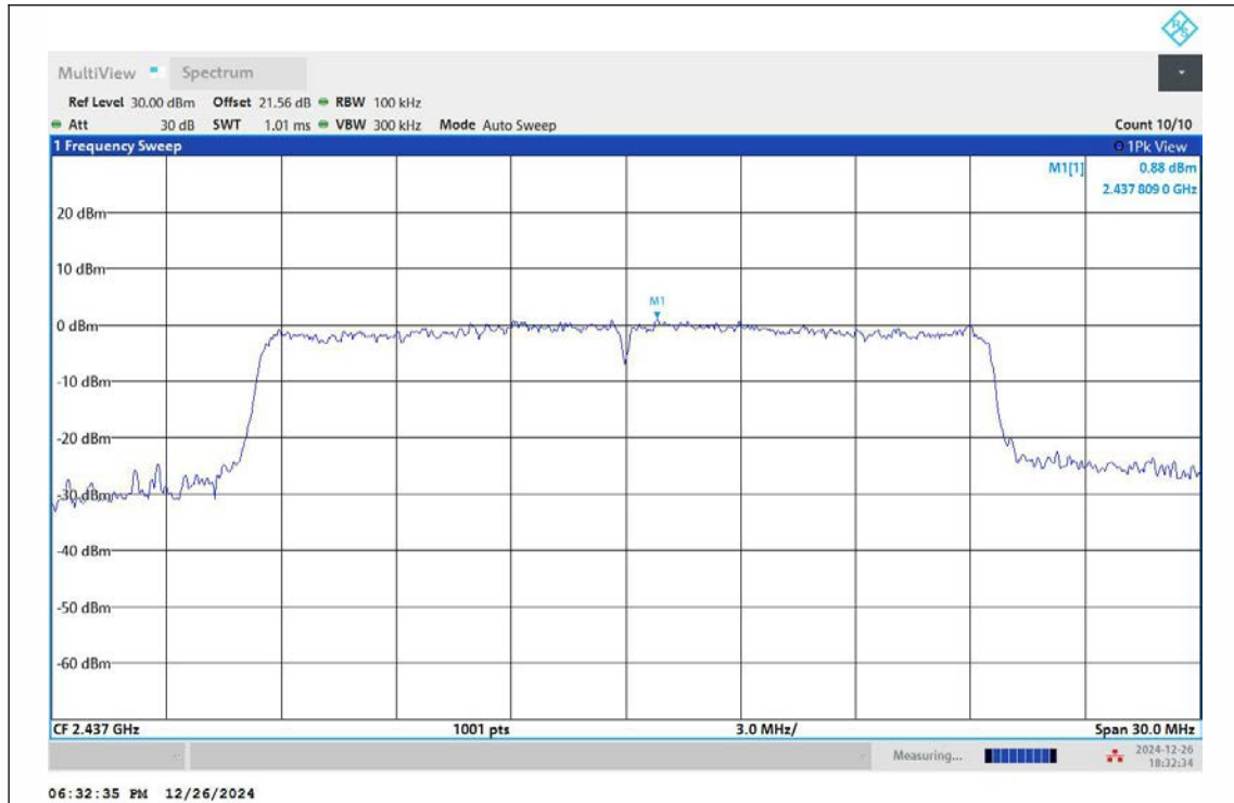
11AX20SISO-Ant1-2437-0~Reference-PASS
