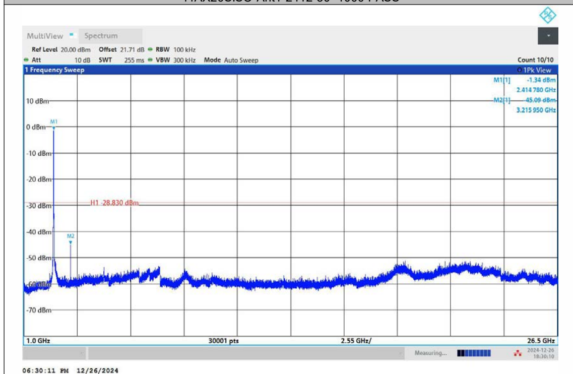
11AX20SISO-Ant1-2412-1000~26500-PASS
