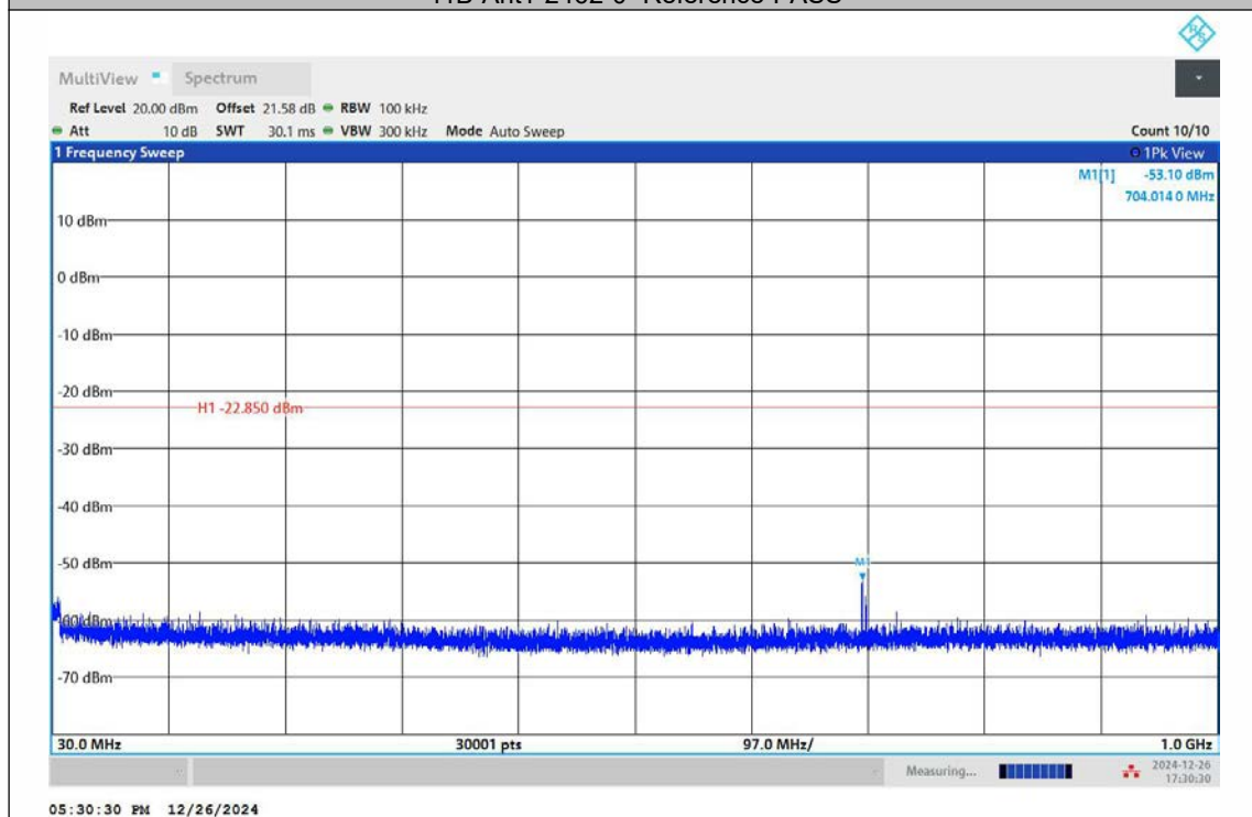
11B-Ant1-2462-30~1000-PASS
