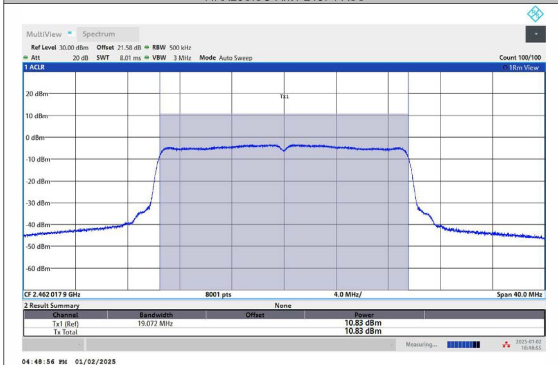
11AX20SISO-Ant1-2462-PASS
