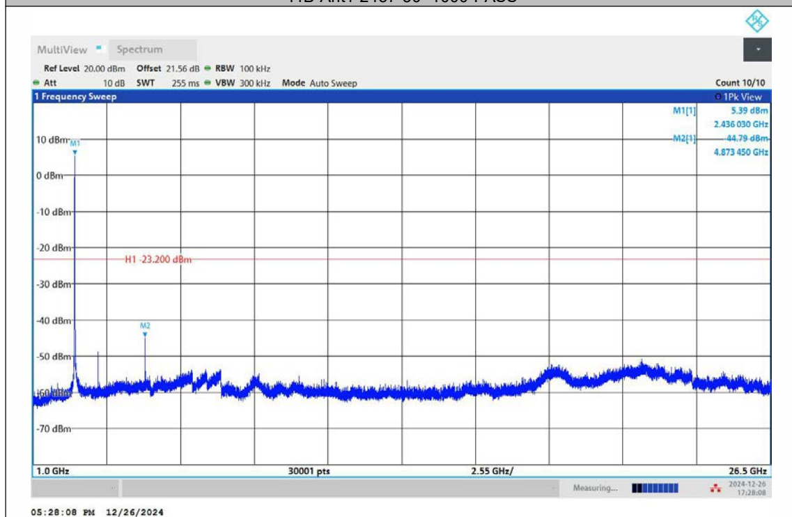
11B-Ant1-2437-1000~26500-PASS
