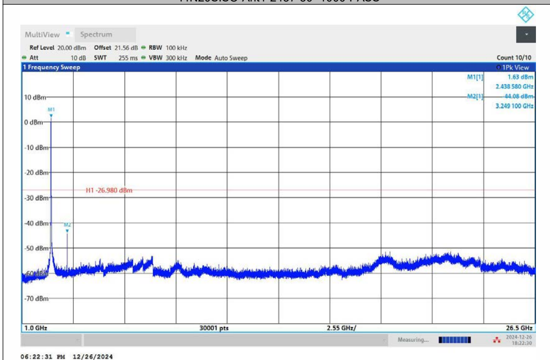
11N20SISO-Ant1-2437-1000~26500-PASS
