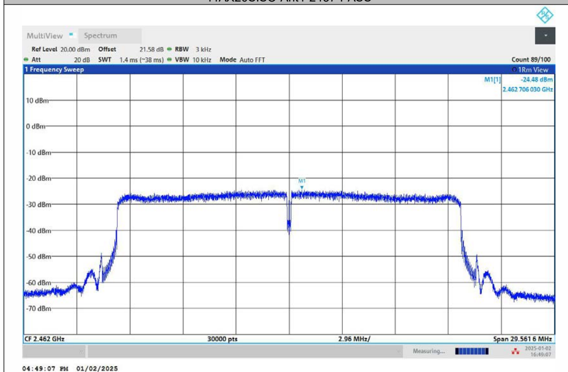
11AX20SISO-Ant1-2462-PASS
