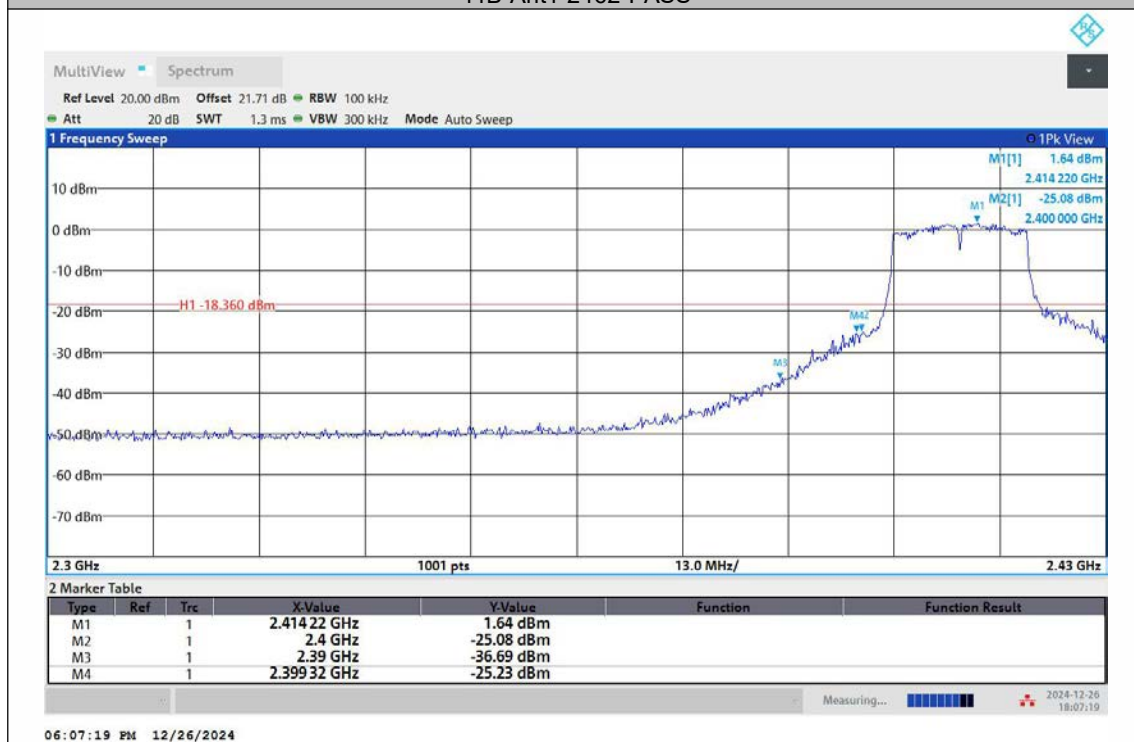
11G-Ant1-2412-PASS
