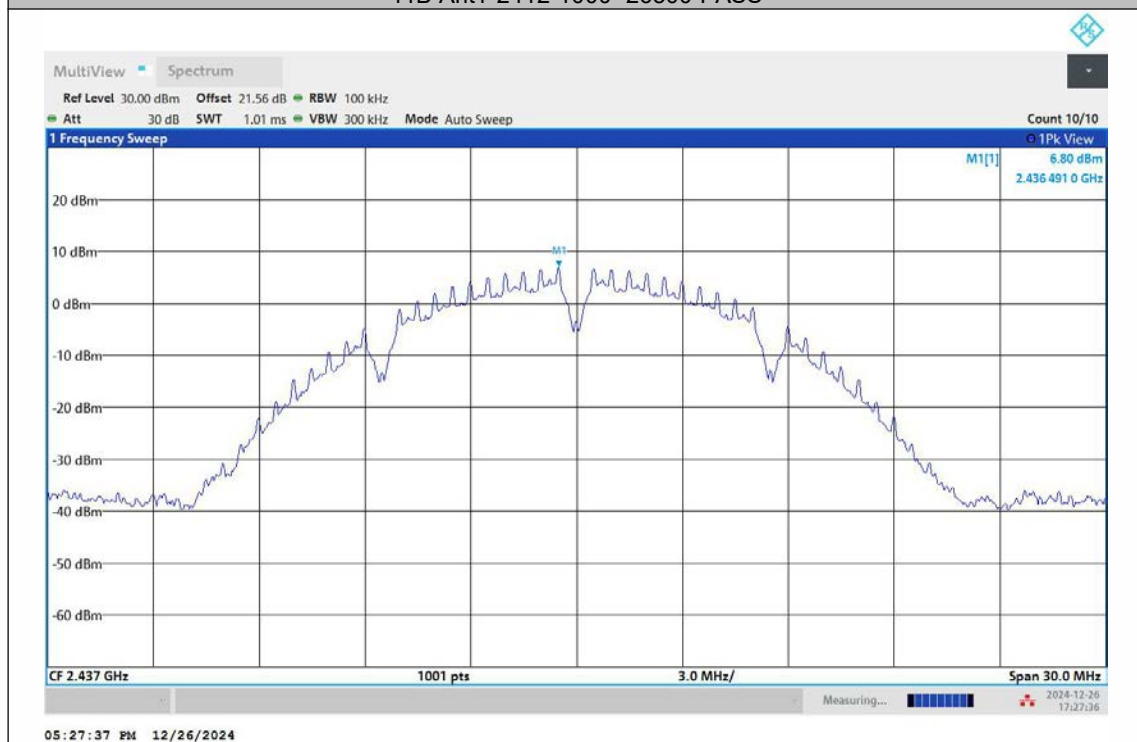
11B-Ant1-2437-0~Reference-PASS
