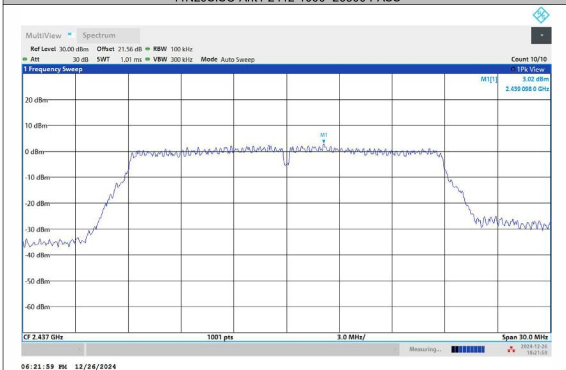
11N20SISO-Ant1-2437-0~Reference-PASS
