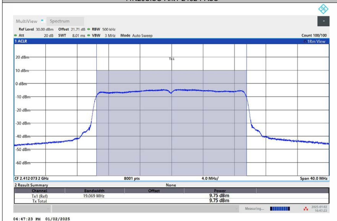
11AX20SISO-Ant1-2412-PASS
