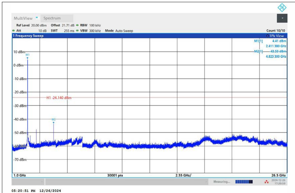
11B-Ant1-2412-1000~26500-PASS
