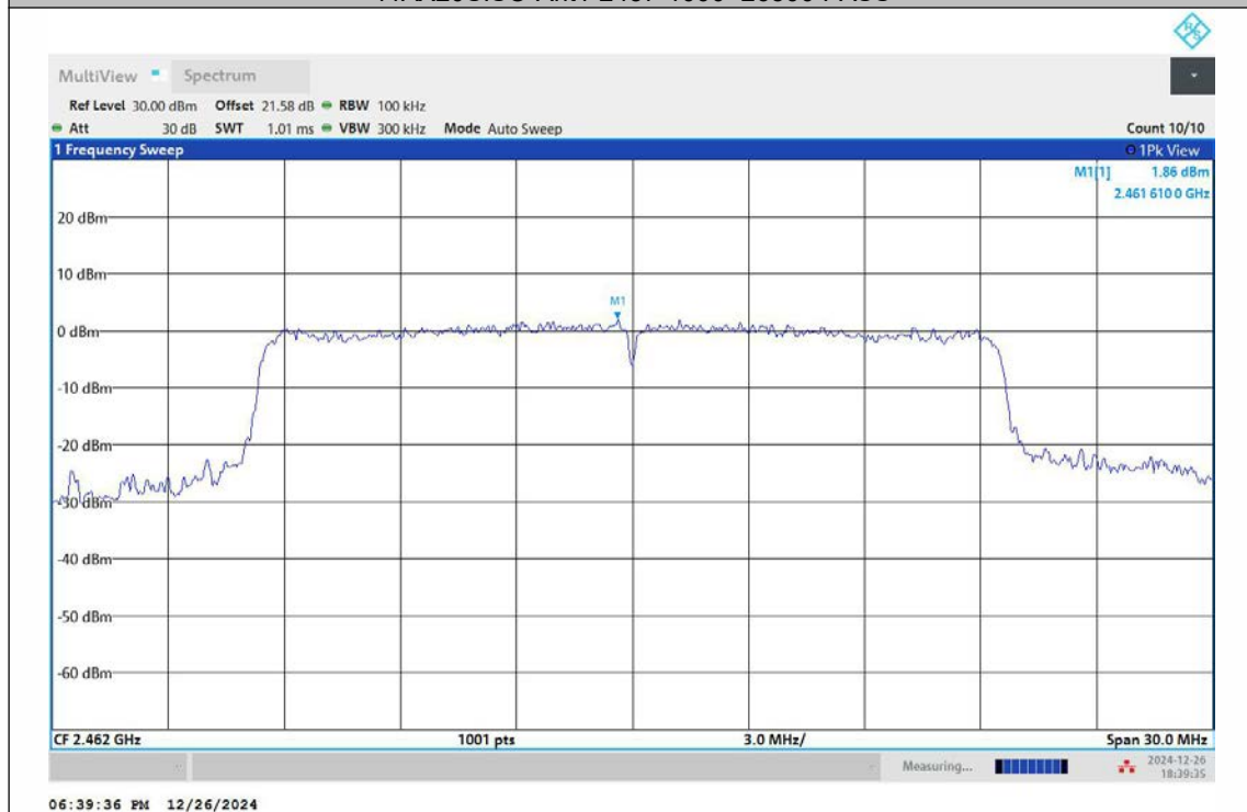
11AX20SISO-Ant1-2462-0~Reference-PASS
