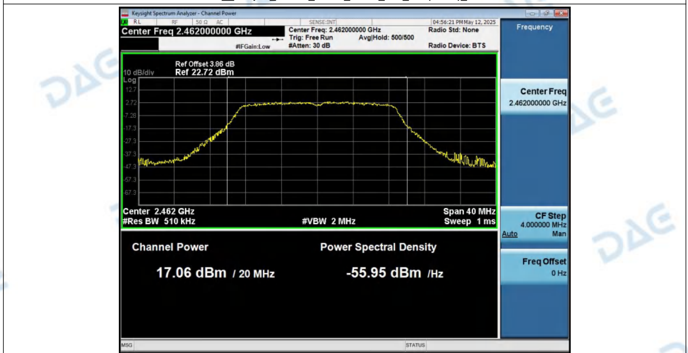
MAX__Output_Power_NVNT_ANT1_802_11n(HT20)_2462
