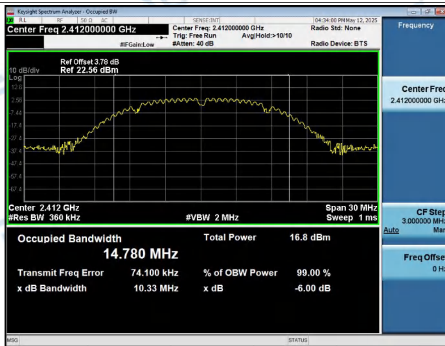
-6dB_Bandwidth_NVNT_ANT1_802_11b_2412
