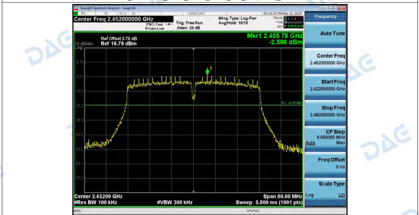
2_Bandedge_NVNT_ANT1_802_11n(HT40)_2452
