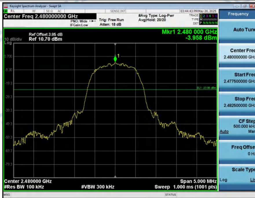
2_Spurious_Emissions_NVNT_ANT1_3-DH5_2480_00
