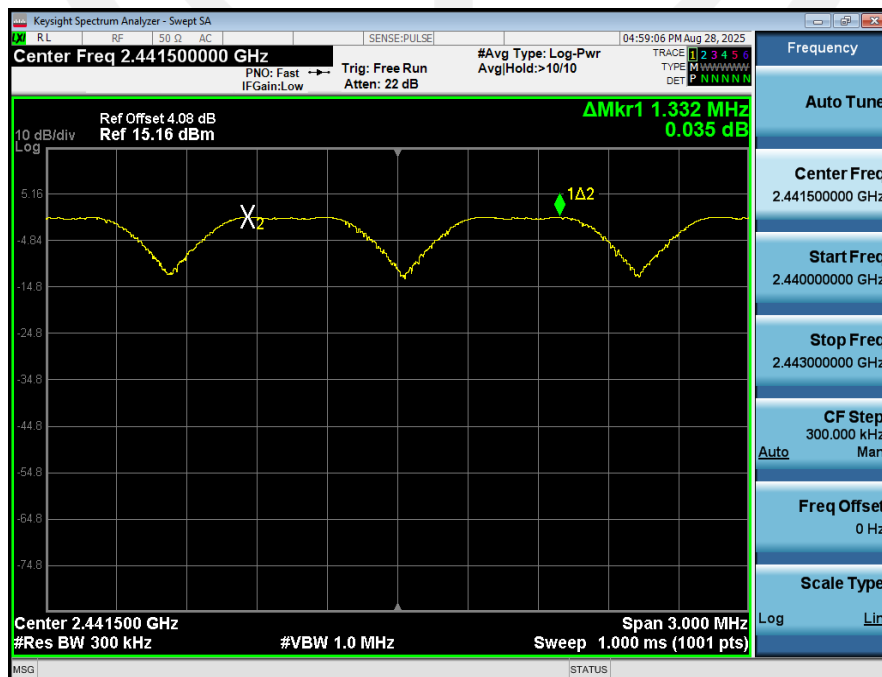
Carrier_Frequencies_Separation_(Hopping)_NVNT_ANT1_1-DH1_Hopping
