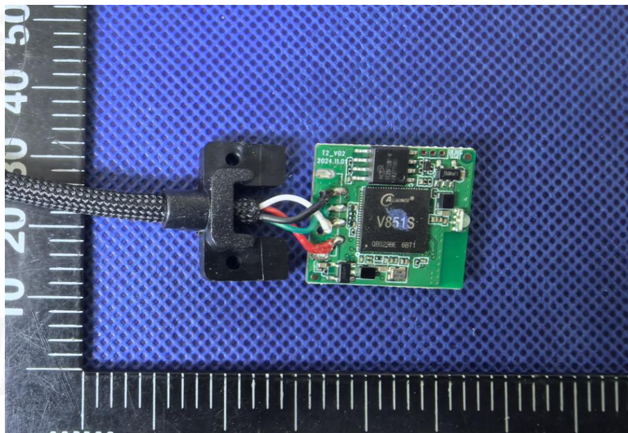
PCB view
