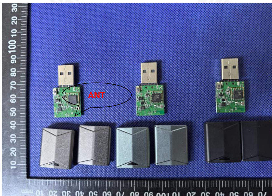
PCB view
