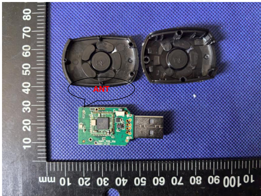
PCB view
