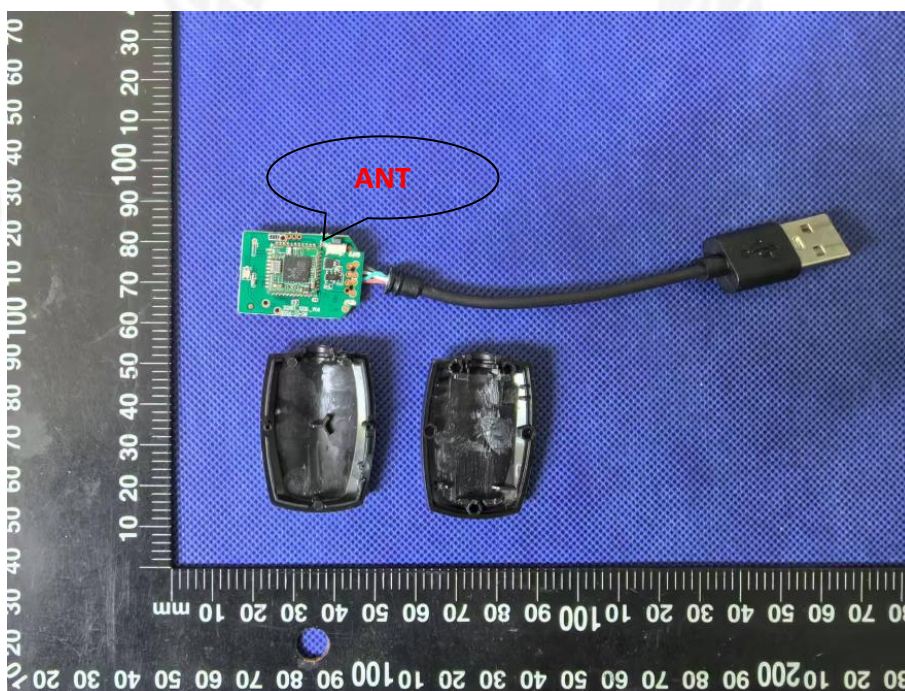
PCB view
