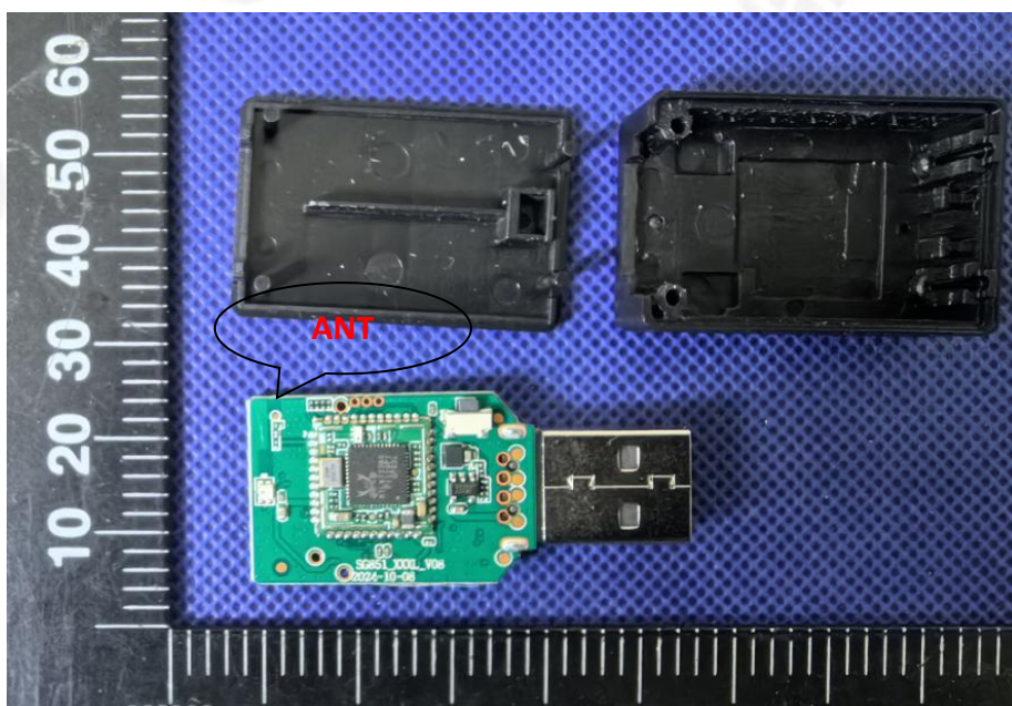
PCB view
