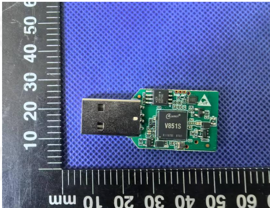
PCB view
