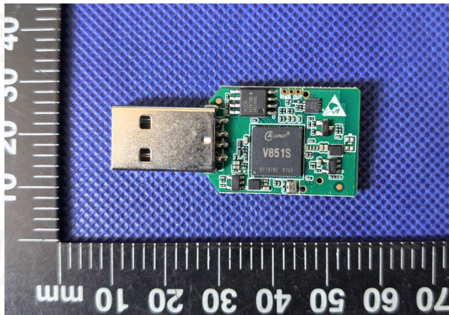
PCB view
