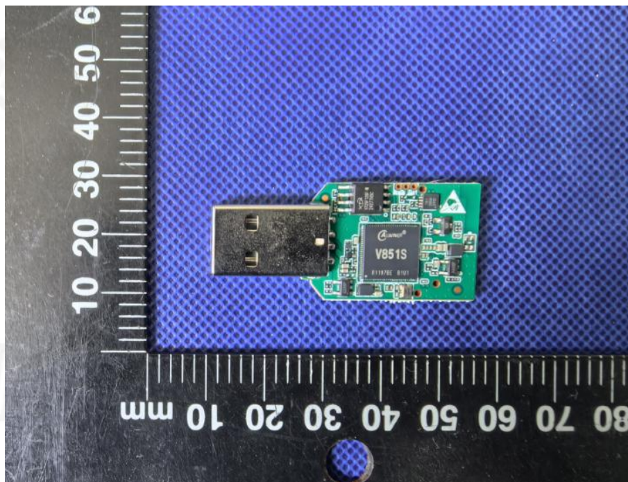
PCB view
