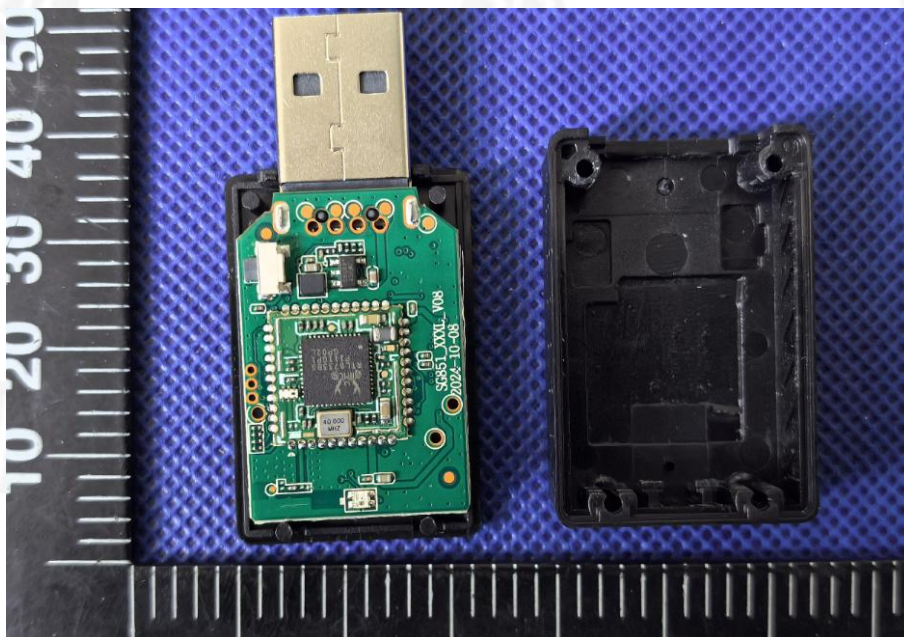
Internal view
