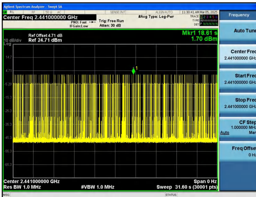
Dwell_Time_(Hopping)_NVNT_ANT1_3-DH3_2441_00_Accumulated
