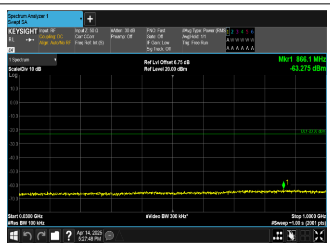
Band66-20MHz-QPSK-132572-1RB#99-30~1000-PASS
