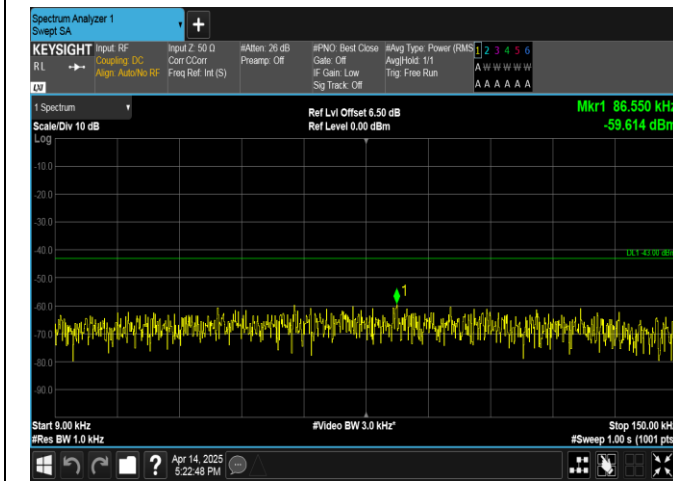
Band66-20MHz-QPSK-132322-1RB#99-0.009~0.15-PASS
