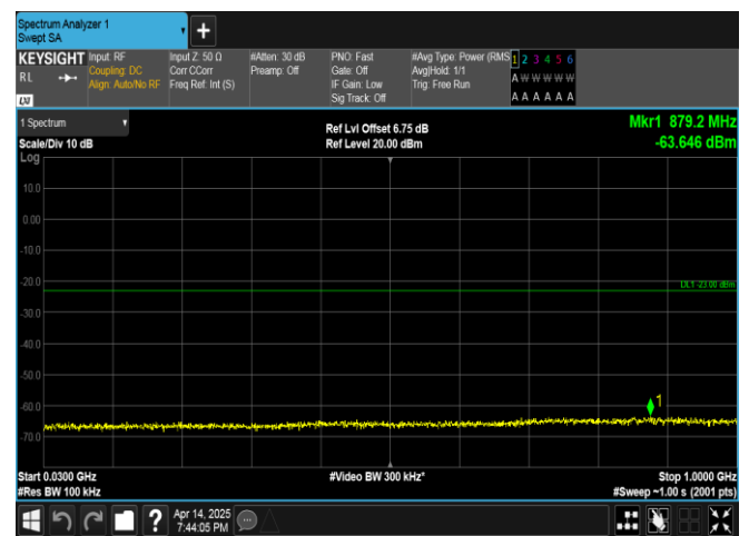
Band66-20MHz-QPSK-132322-100RB#0-30~1000-PASS
