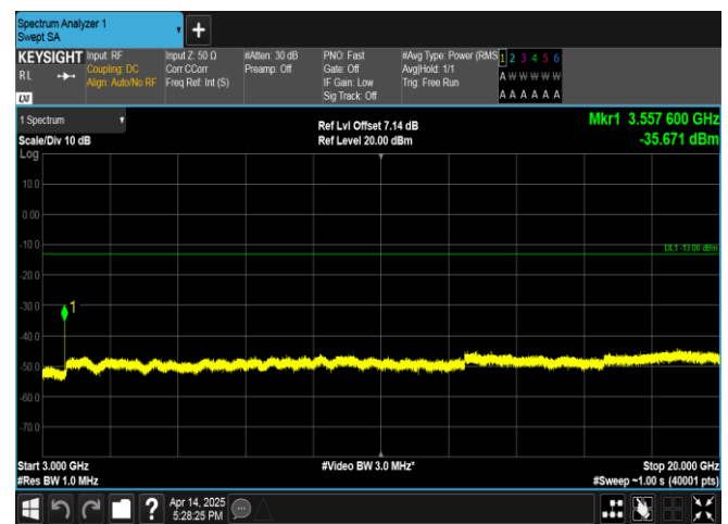
Band66-20MHz-QPSK-132572-1RB#99-3000~20000-PASS
