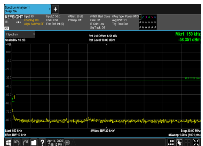
Band66-20MHz-QPSK-132572-100RB#0-0.15~30-PASS
