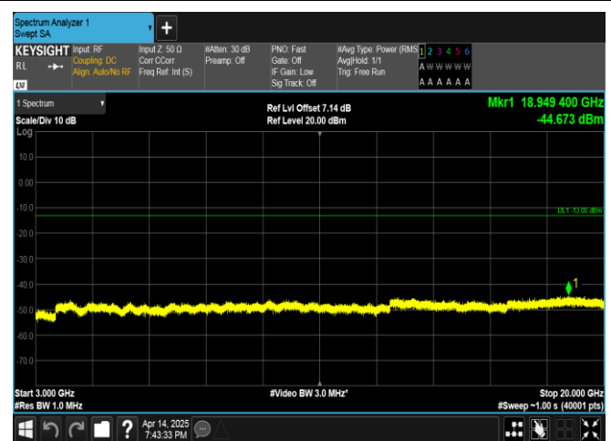
Band66-20MHz-16QAM-132072-100RB#0-3000~20000-PASS
