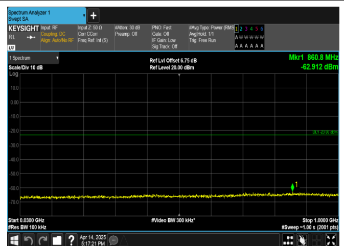
Band66-20MHz-16QAM-132072-1RB#0-30~1000-PASS
