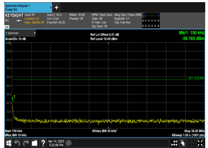
Band66-20MHz-QPSK-132322-1RB#99-0.15~30-PASS
