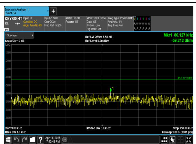
Band66-20MHz-QPSK-132322-100RB#0-0.009~0.15-PASS
