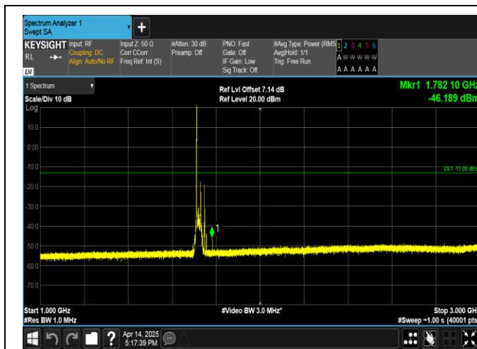
Band66-20MHz-16QAM-132072-1RB#0-1000~3000-PASS
