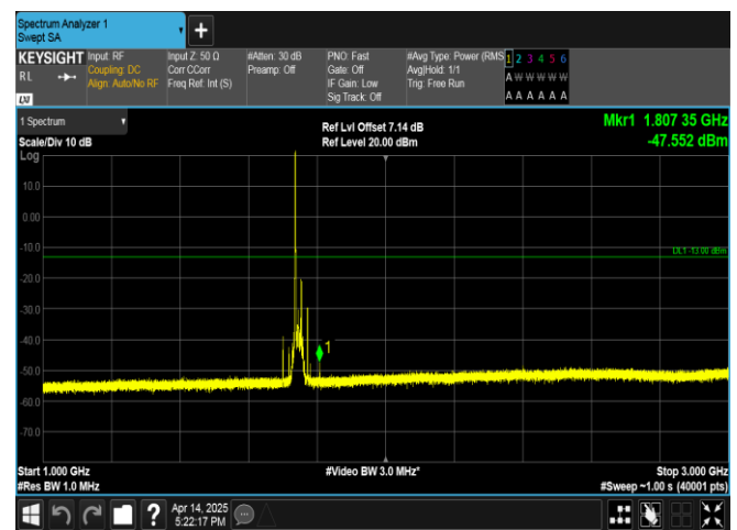
Band66-20MHz-16QAM-132322-1RB#0-1000~3000-PASS
