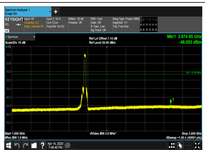
Band66-20MHz-QPSK-132572-100RB#0-1000~3000-PASS
