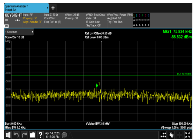
Band66-20MHz-16QAM-132072-1RB#0-0.009~0.15-PASS
