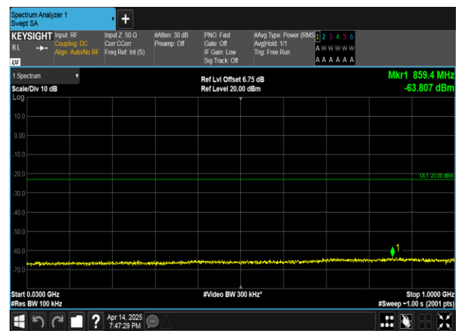
Band66-20MHz-16QAM-132572-100RB#0-30~1000-PASS
