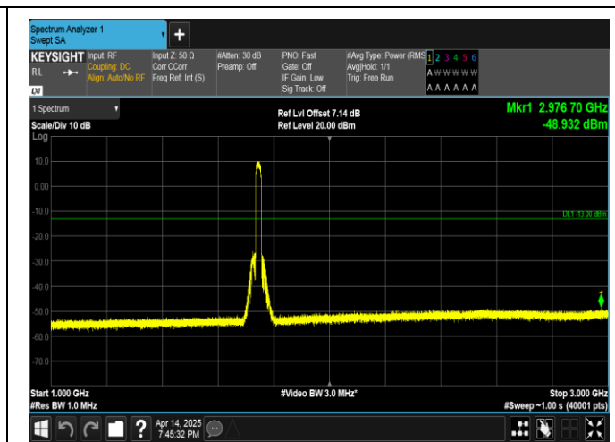
Band66-20MHz-16QAM-132322-100RB#0-1000~3000-PASS
