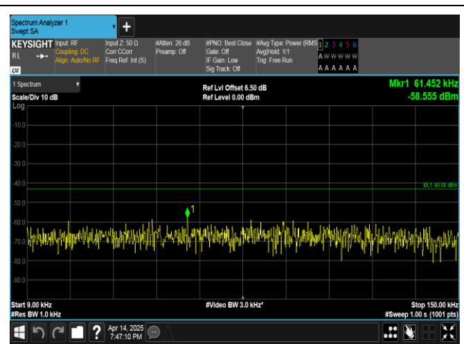
Band66-20MHz-16QAM-132572-100RB#0-0.009~0.15-PASS
