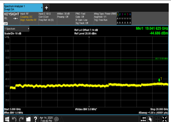
Band66-20MHz-QPSK-132322-100RB#0-3000~20000-PASS
