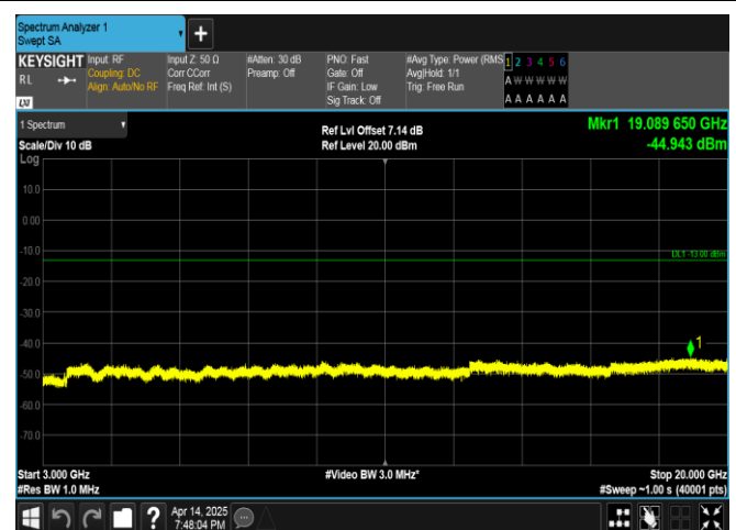
Band66-20MHz-16QAM-132572-100RB#0-3000~20000-PASS
