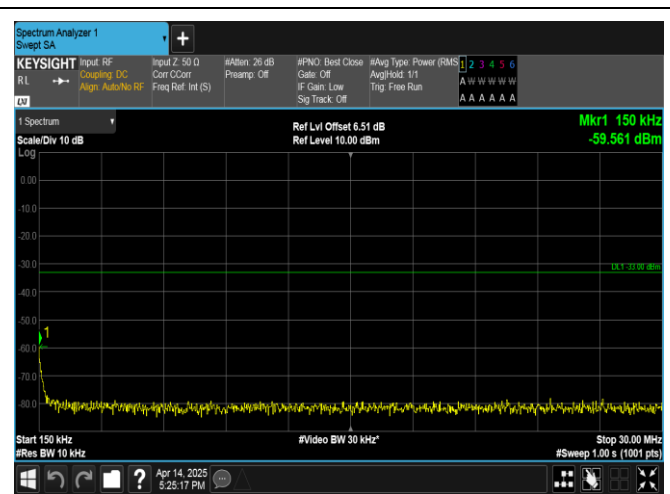
Band66-20MHz-QPSK-132572-1RB#0-0.15~30-PASS
