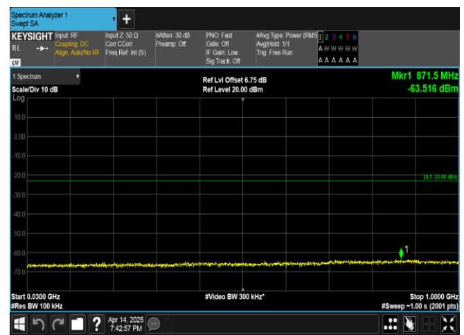
Band66-20MHz-16QAM-132072-100RB#0-30~1000-PASS
