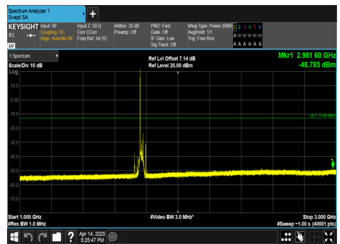
Band66-20MHz-QPSK-132572-1RB#0-1000~3000-PASS
