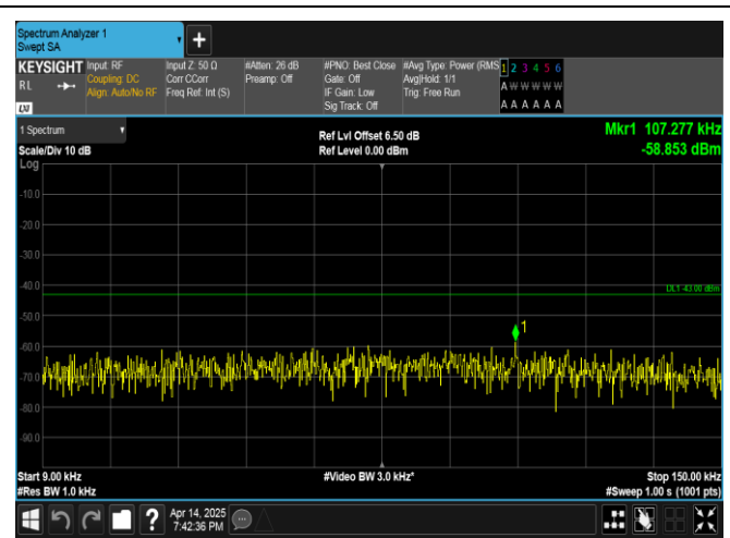
Band66-20MHz-16QAM-132072-100RB#0-0.009~0.15-PASS
