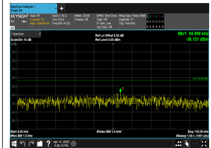
Band66-20MHz-16QAM-132572-1RB#0-0.009~0.15-PASS
