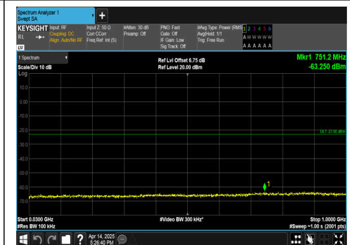
Band66-20MHz-16QAM-132572-1RB#0-30~1000-PASS
