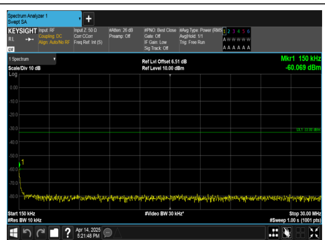
Band66-20MHz-16QAM-132322-1RB#0-0.15~30-PASS
