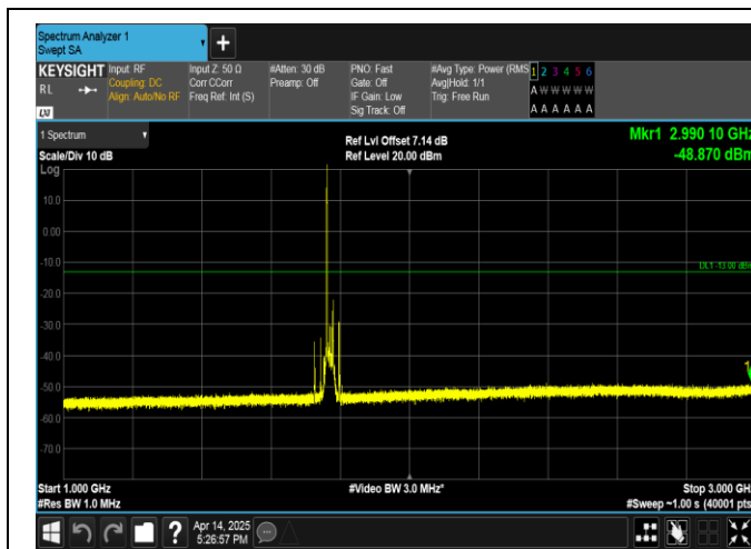
Band66-20MHz-16QAM-132572-1RB#0-1000~3000-PASS
