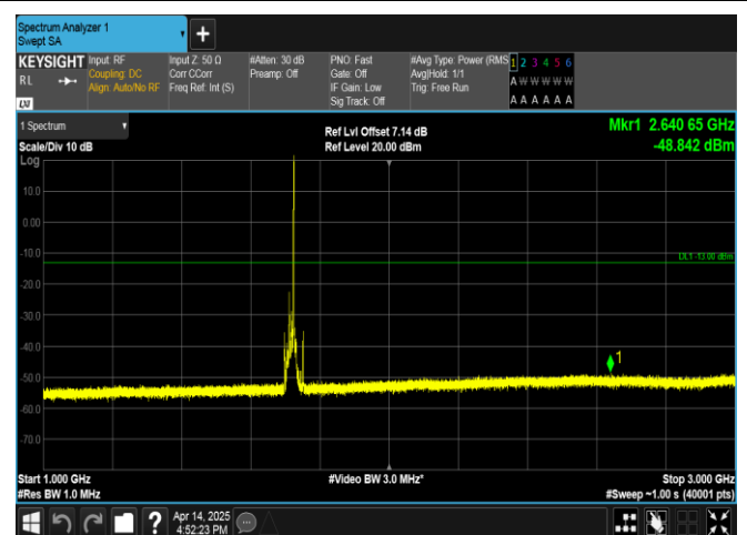
Band66-15MHz-16QAM-132047-1RB#74-1000~3000-PASS
