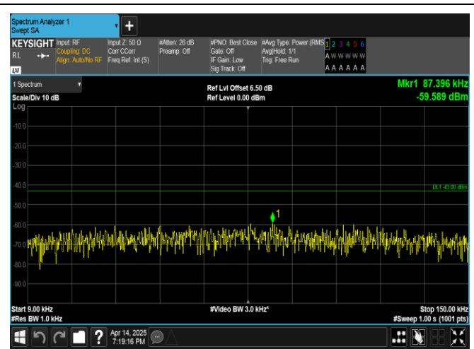
Band66-15MHz-QPSK-132322-75RB#0-0.009~0.15-PASS
