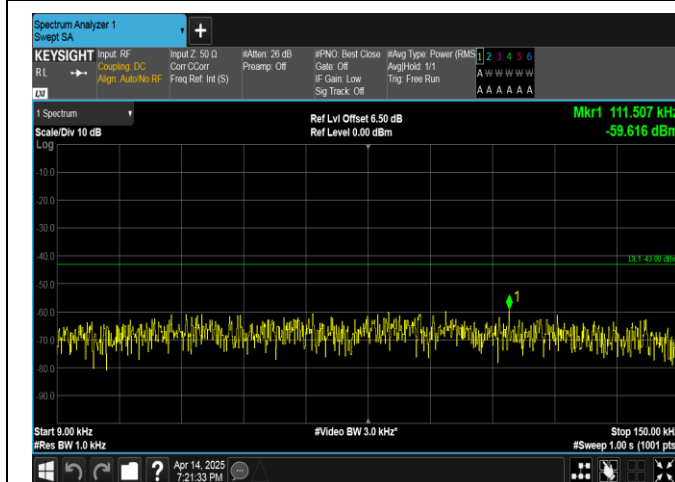
Band66-15MHz-QPSK-132597-75RB#0-0.009~0.15-PASS
