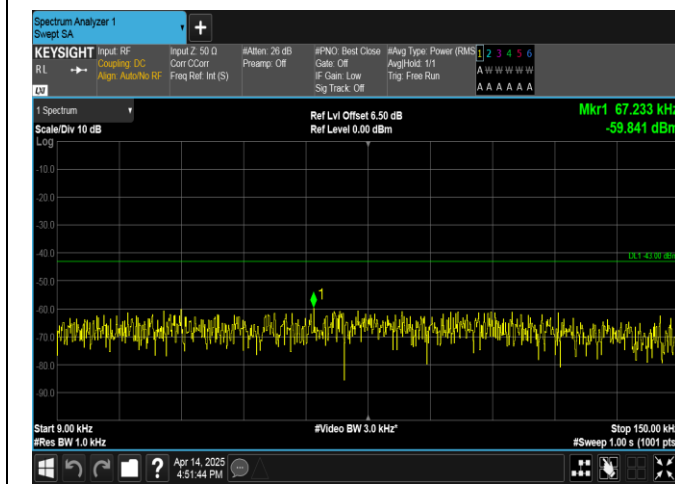
Band66-15MHz-16QAM-132047-1RB#74-0.009~0.15-PASS
