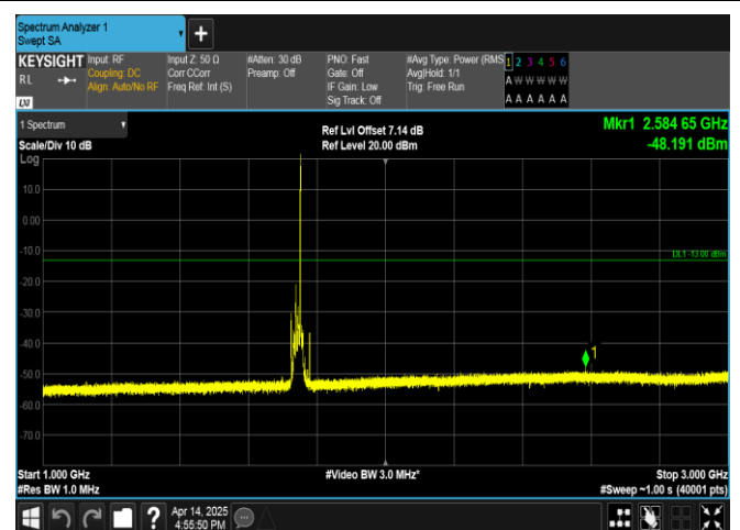
Band66-15MHz-QPSK-132322-1RB#74-1000~3000-PASS
