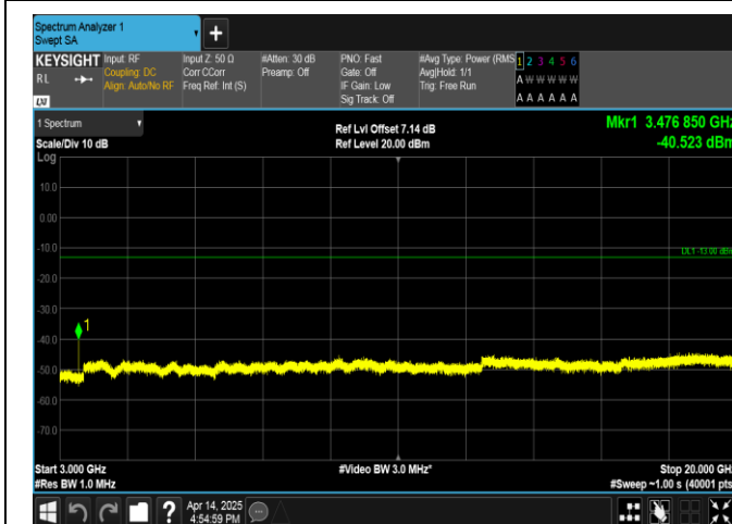
Band66-15MHz-16QAM-132322-1RB#0-3000~20000-PASS
