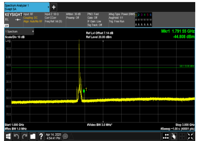
Band66-15MHz-16QAM-132322-1RB#0-1000~3000-PASS
