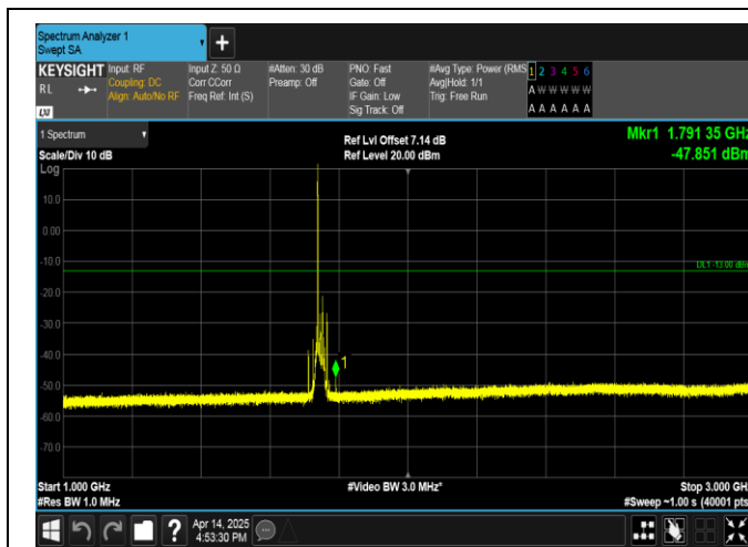
Band66-15MHz-QPSK-132322-1RB#0-1000~3000-PASS
