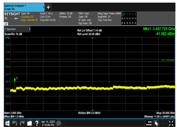
Band66-20MHz-QPSK-132072-1RB#99-3000~20000-PASS
