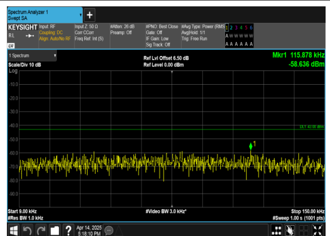
Band66-20MHz-QPSK-132072-1RB#99-0.009~0.15-PASS
