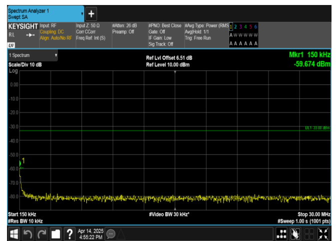
Band66-15MHz-QPSK-132322-1RB#74-0.15~30-PASS
