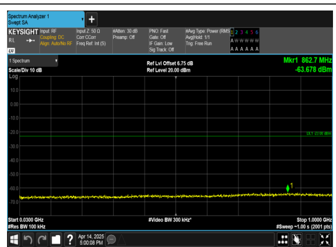
Band66-15MHz-QPSK-132597-1RB#74-30~1000-PASS
