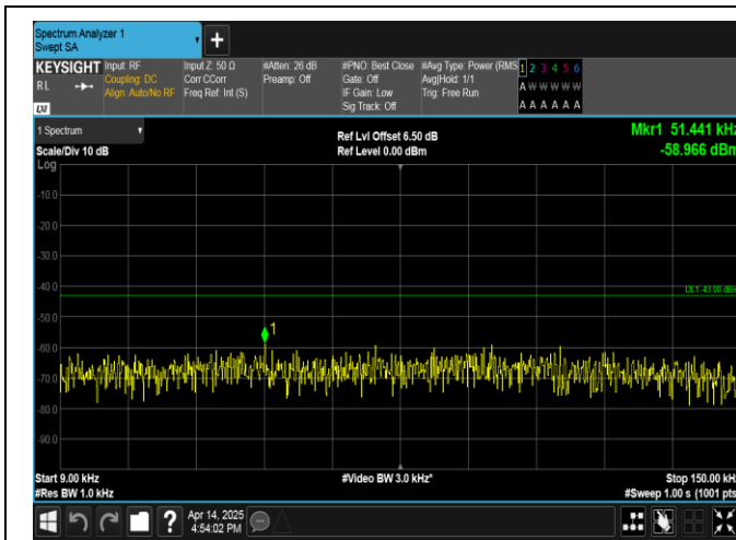
Band66-15MHz-16QAM-132322-1RB#0-0.009~0.15-PASS
