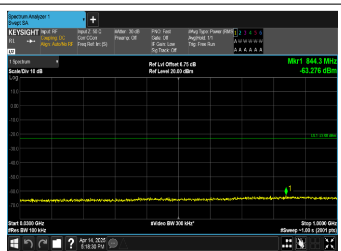
Band66-20MHz-QPSK-132072-1RB#99-30~1000-PASS
