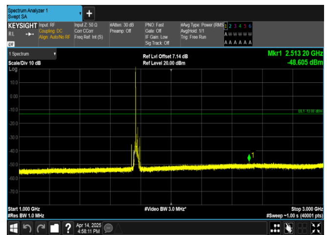
Band66-15MHz-QPSK-132597-1RB#0-1000~3000-PASS
