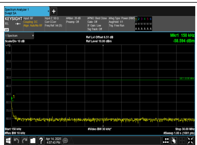
Band66-15MHz-QPSK-132597-1RB#0-0.15~30-PASS
