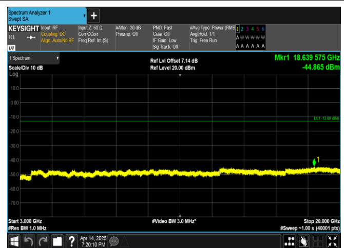
Band66-15MHz-QPSK-132322-75RB#0-3000~20000-PASS
