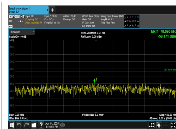
Band66-20MHz-QPSK-132072-1RB#0-0.009~0.15-PASS
