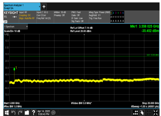
Band66-15MHz-QPSK-132597-1RB#74-3000~20000-PASS
