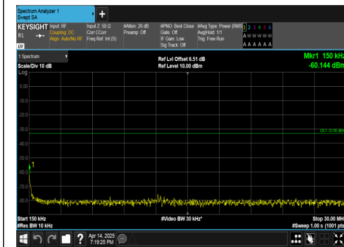
Band66-15MHz-QPSK-132322-75RB#0-0.15~30-PASS
