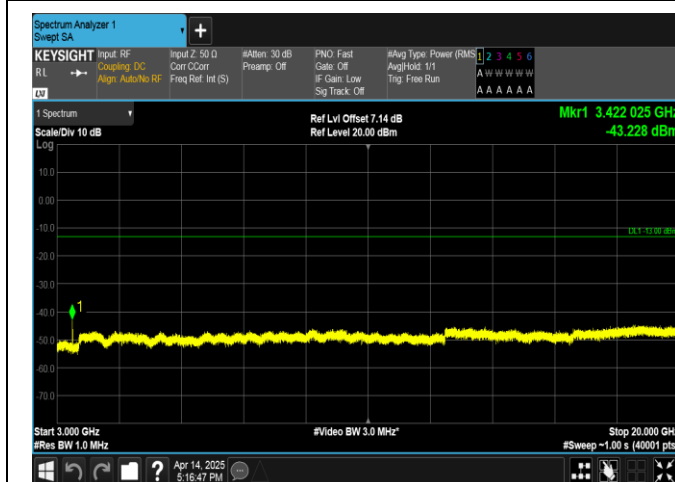
Band66-20MHz-QPSK-132072-1RB#0-3000~20000-PASS
