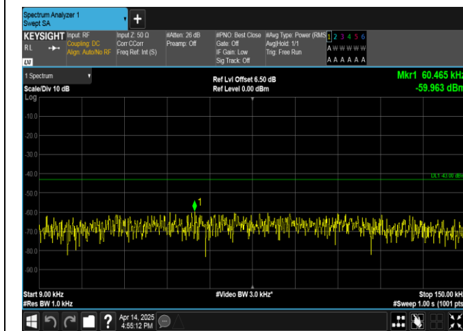
Band66-15MHz-QPSK-132322-1RB#74-0.009~0.15-PASS
