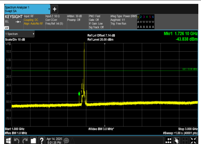
Band66-15MHz-16QAM-132597-1RB#74-1000~3000-PASS
