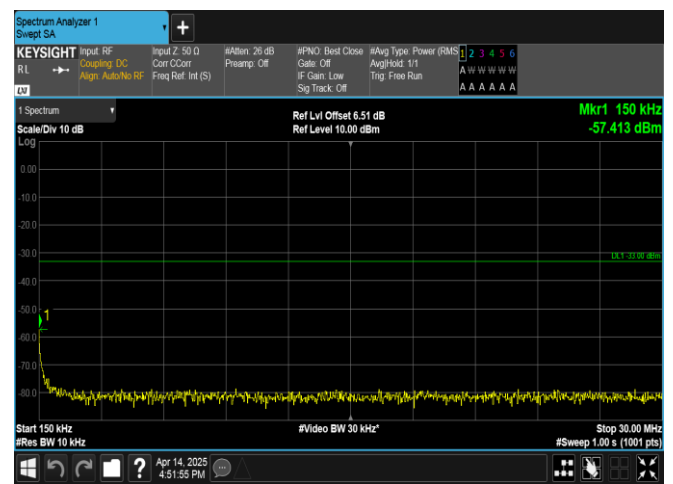
Band66-15MHz-16QAM-132047-1RB#74-0.15~30-PASS
