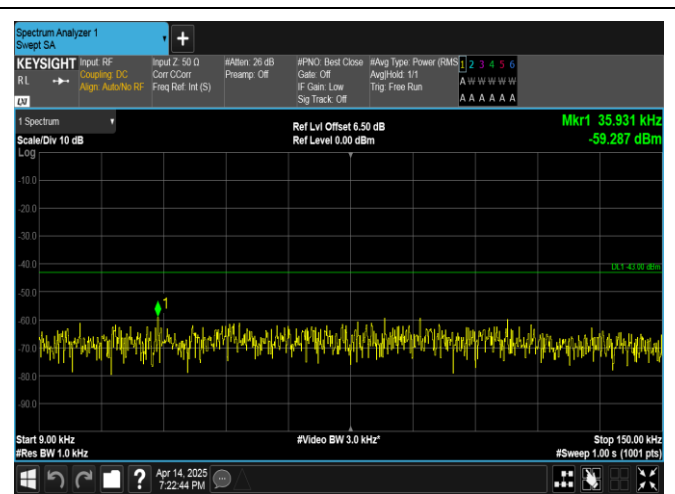
Band66-15MHz-16QAM-132597-75RB#0-0.009~0.15-PASS
