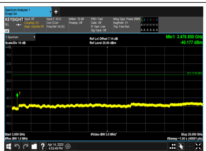
Band66-15MHz-QPSK-132322-1RB#0-3000~20000-PASS
