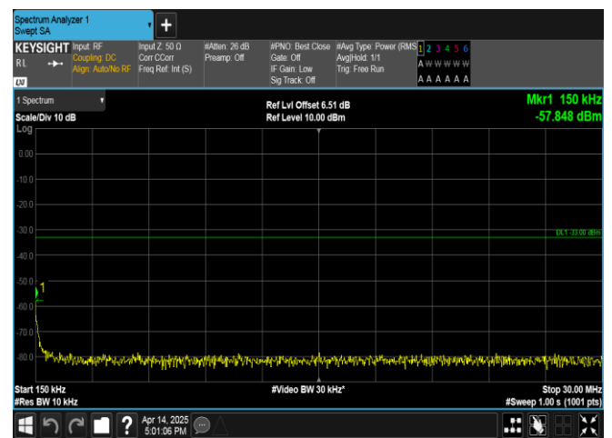
Band66-15MHz-16QAM-132597-1RB#74-0.15~30-PASS
