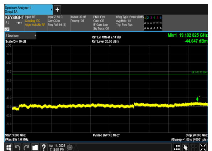
Band66-15MHz-16QAM-132047-75RB#0-3000~20000-PASS
