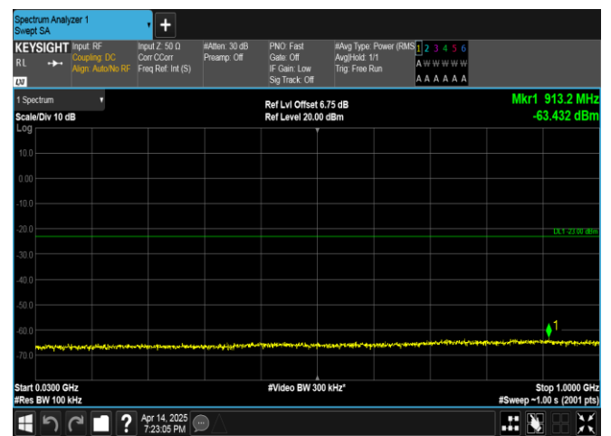
Band66-15MHz-16QAM-132597-75RB#0-30~1000-PASS
