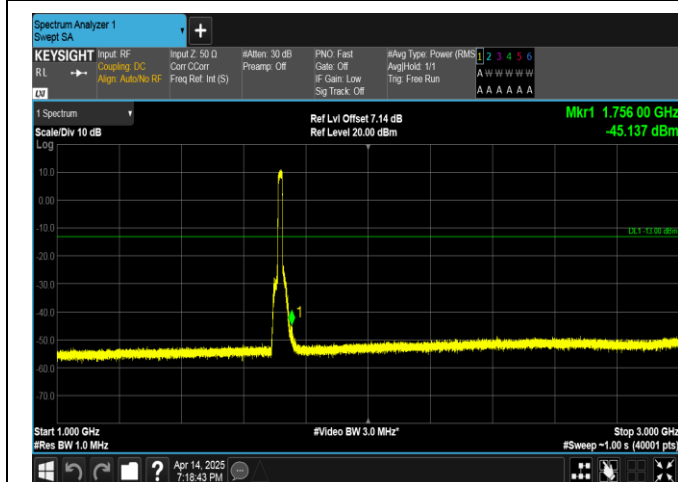
Band66-15MHz-16QAM-132047-75RB#0-1000~3000-PASS
