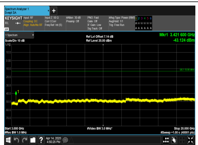
Band66-15MHz-16QAM-132047-1RB#0-3000~20000-PASS
