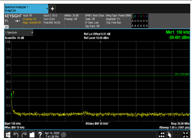
Band66-20MHz-QPSK-132072-100RB#0-0.15~30-PASS
