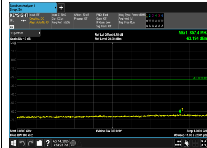
Band66-15MHz-16QAM-132322-1RB#0-30~1000-PASS
