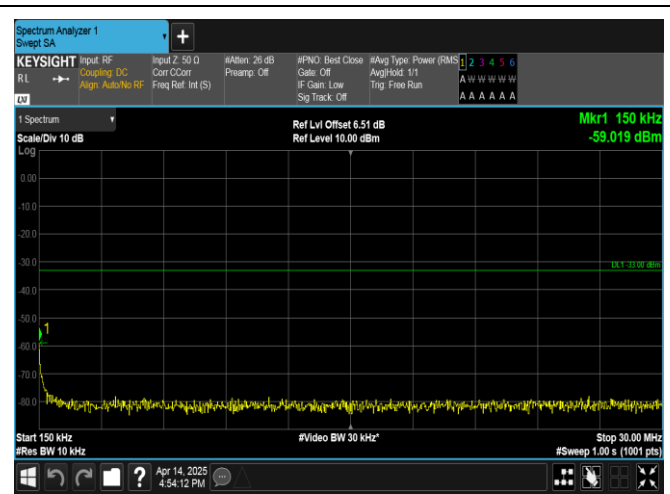
Band66-15MHz-16QAM-132322-1RB#0-0.15~30-PASS
