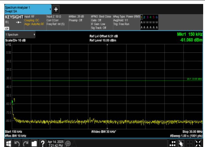
Band66-15MHz-QPSK-132597-75RB#0-0.15~30-PASS
