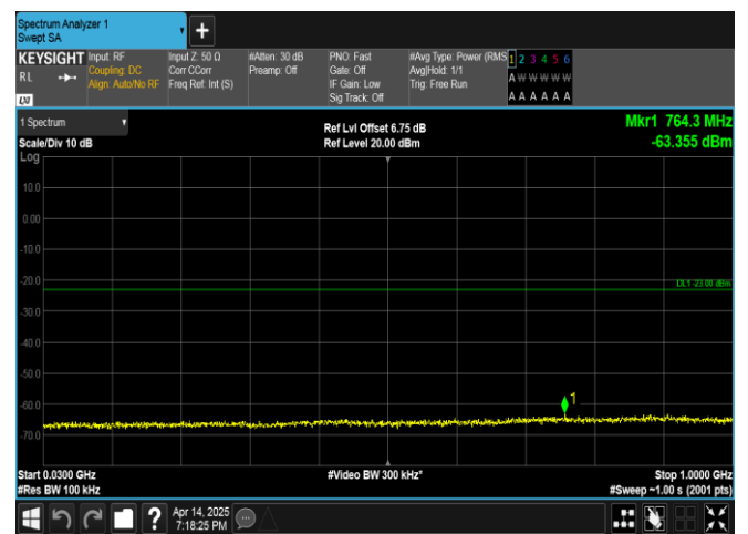
Band66-15MHz-16QAM-132047-75RB#0-30~1000-PASS
