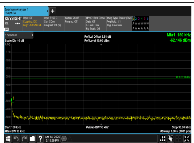
Band66-20MHz-QPSK-132072-1RB#0-0.15~30-PASS
