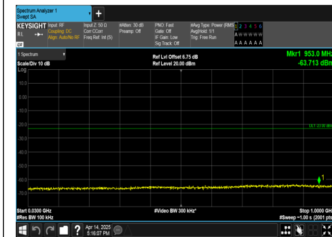
Band66-20MHz-QPSK-132072-1RB#0-30~1000-PASS
