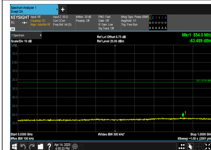
Band66-15MHz-QPSK-132322-1RB#74-30~1000-PASS
