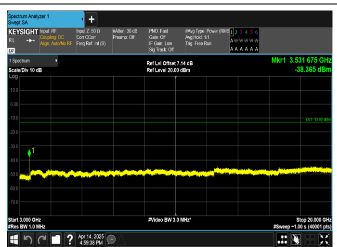
Band66-15MHz-16QAM-132597-1RB#0-3000~20000-PASS
