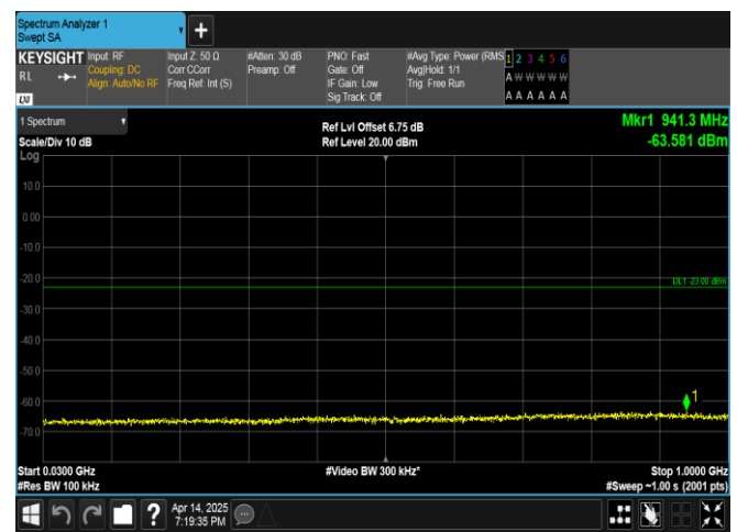
Band66-15MHz-QPSK-132322-75RB#0-30~1000-PASS
