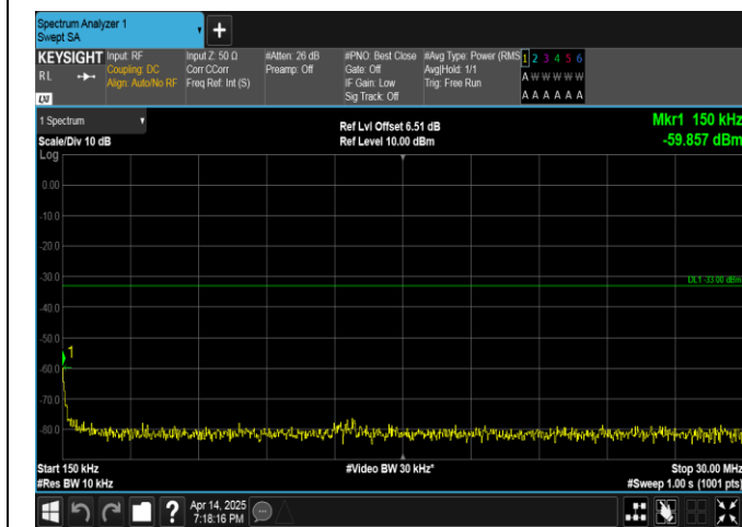
Band66-15MHz-16QAM-132047-75RB#0-0.15~30-PASS
