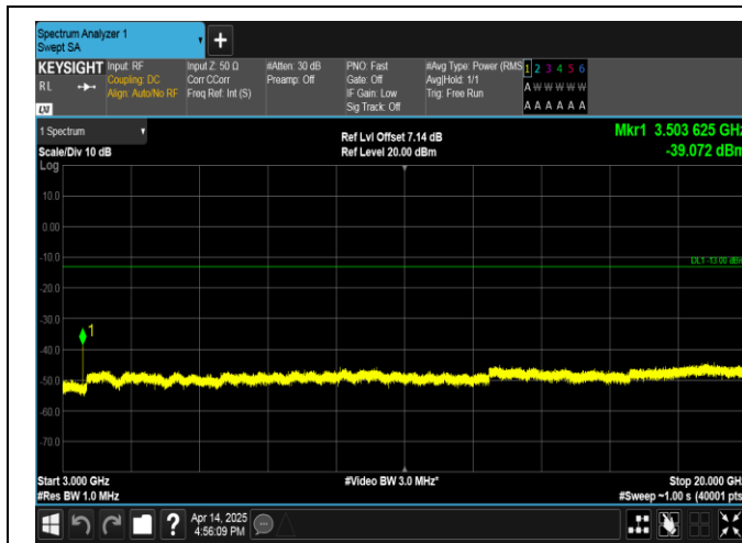
Band66-15MHz-QPSK-132322-1RB#74-3000~20000-PASS
