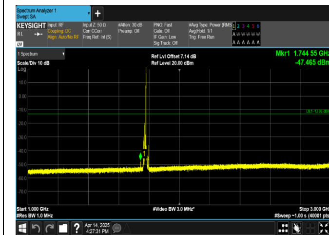
Band66-10MHz-QPSK-132622-1RB#49-1000~3000-PASS
