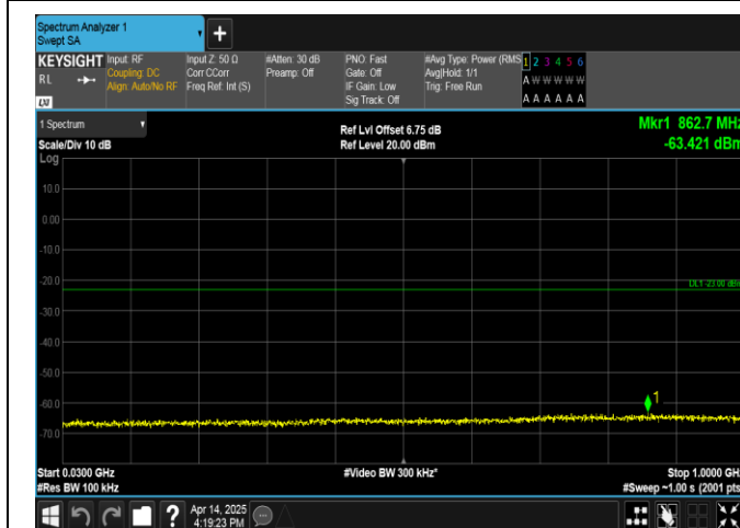
Band66-10MHz-16QAM-132022-1RB#49-30~1000-PASS
