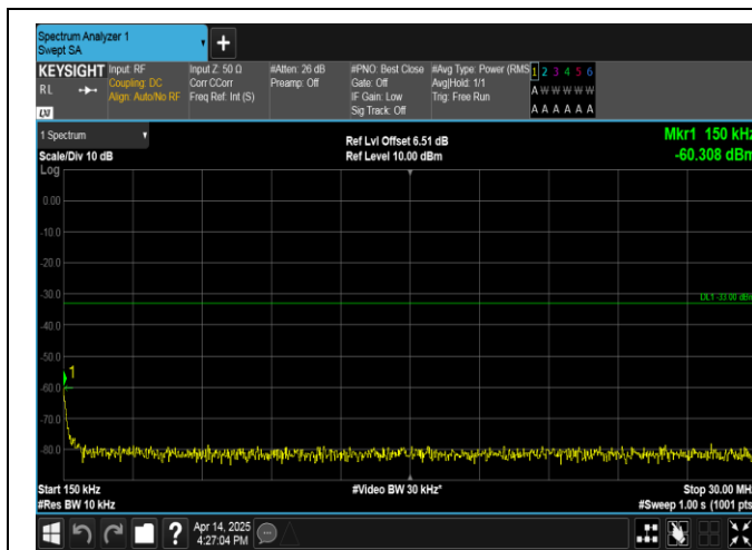
Band66-10MHz-QPSK-132622-1RB#49-0.15~30-PASS
