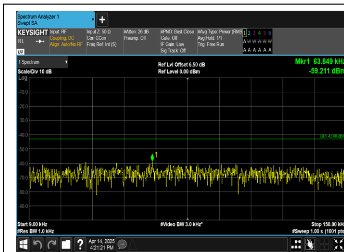
Band66-10MHz-16QAM-132322-1RB#0-0.009~0.15-PASS
