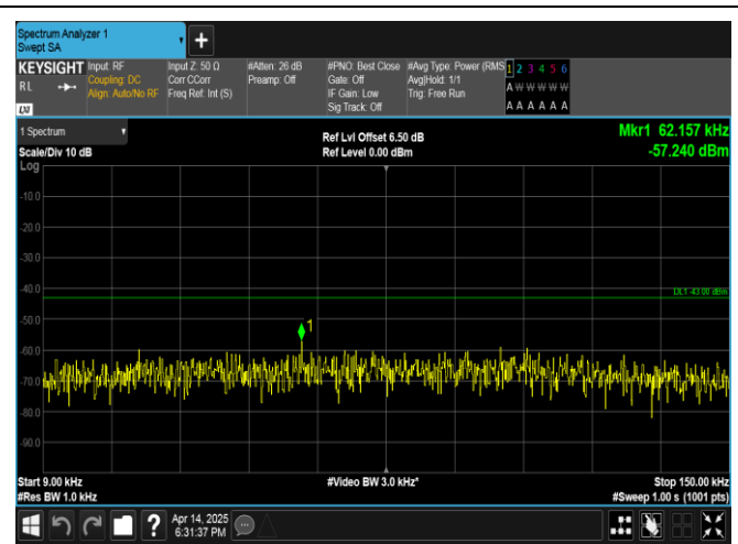
Band66-10MHz-QPSK-132322-50RB#0-0.009~0.15-PASS
