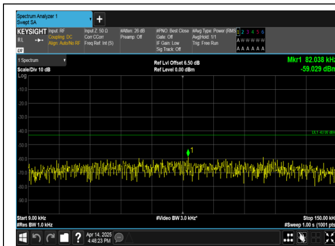
Band66-15MHz-QPSK-132047-1RB#0-0.009~0.15-PASS
