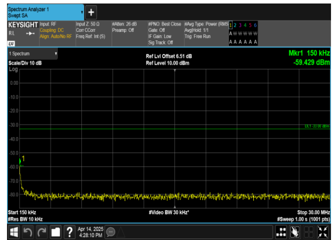
Band66-10MHz-16QAM-132622-1RB#49-0.15~30-PASS
