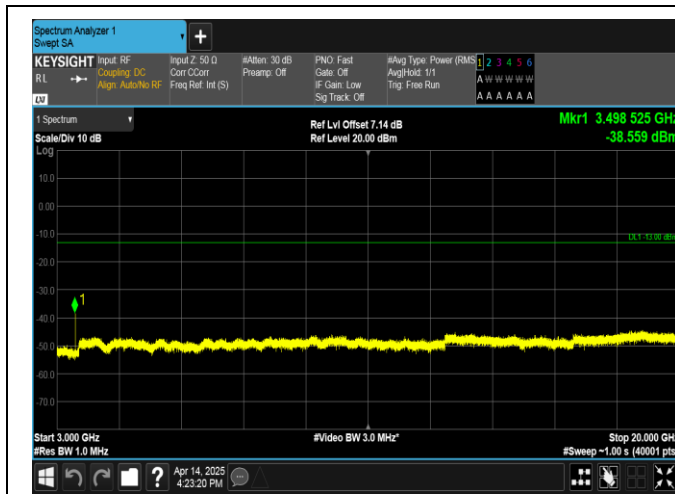
Band66-10MHz-QPSK-132322-1RB#49-3000~20000-PASS
