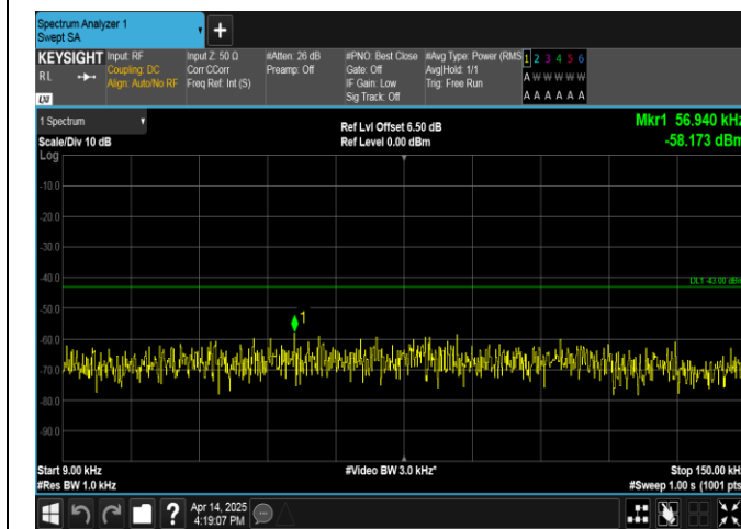
Band66-10MHz-16QAM-132022-1RB#49-0.009~0.15-PASS
