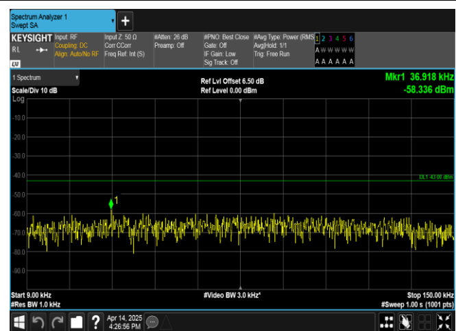
Band66-10MHz-QPSK-132622-1RB#49-0.009~0.15-PASS
