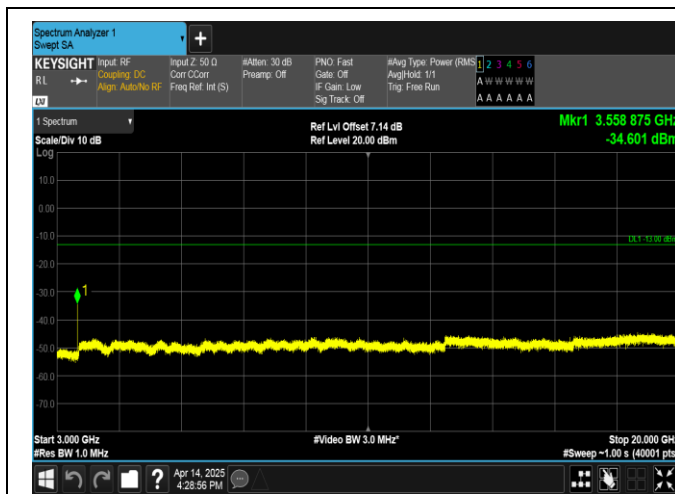
Band66-10MHz-16QAM-132622-1RB#49-3000~20000-PASS
