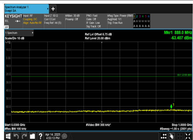
Band66-15MHz-QPSK-132322-1RB#0-30~1000-PASS
