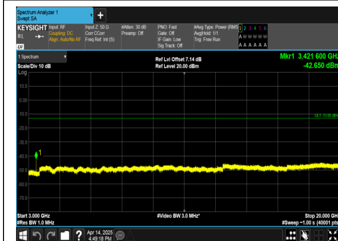
Band66-15MHz-QPSK-132047-1RB#0-3000~20000-PASS
