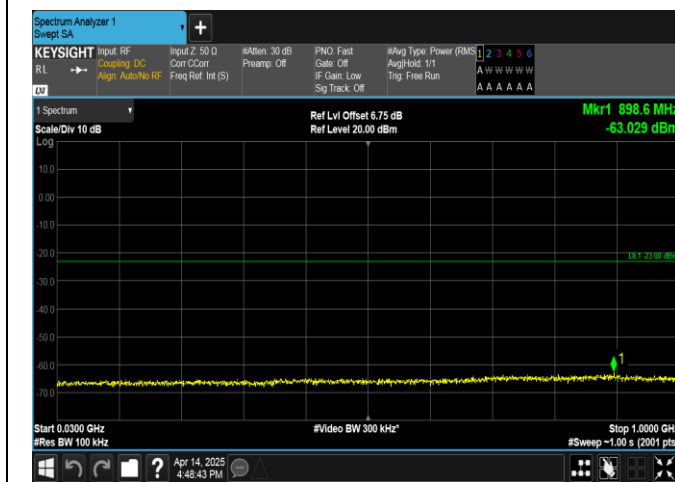
Band66-15MHz-QPSK-132047-1RB#0-30~1000-PASS
