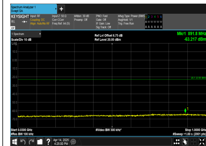
Band66-10MHz-QPSK-132622-1RB#0-30~1000-PASS
