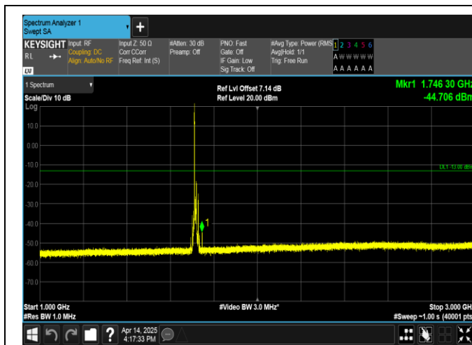
Band66-10MHz-16QAM-132022-1RB#0-1000~3000-PASS
