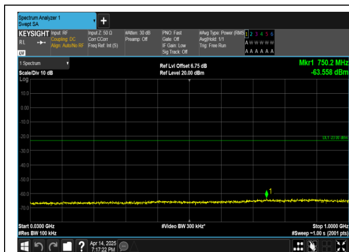
Band66-15MHz-QPSK-132047-75RB#0-30~1000-PASS
