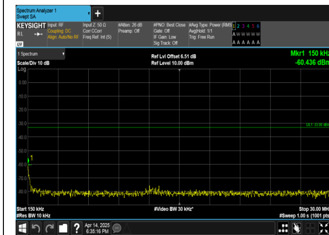
Band66-10MHz-16QAM-132622-50RB#0-0.15~30-PASS
