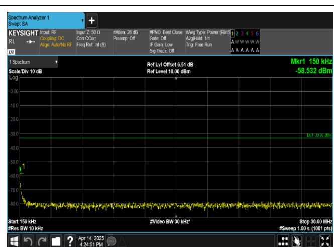
Band66-10MHz-QPSK-132622-1RB#0-0.15~30-PASS
