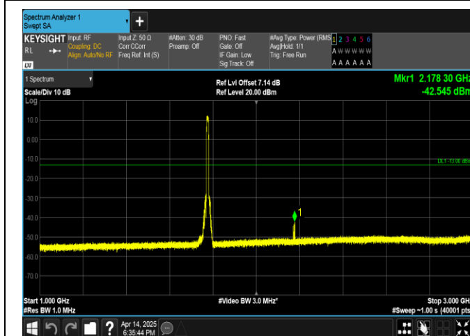
Band66-10MHz-16QAM-132622-50RB#0-1000~3000-PASS
