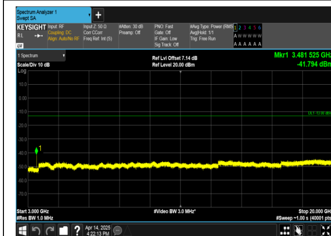
Band66-10MHz-16QAM-132322-1RB#0-3000~20000-PASS
