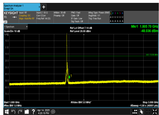
Band66-10MHz-QPSK-132622-1RB#0-1000~3000-PASS
