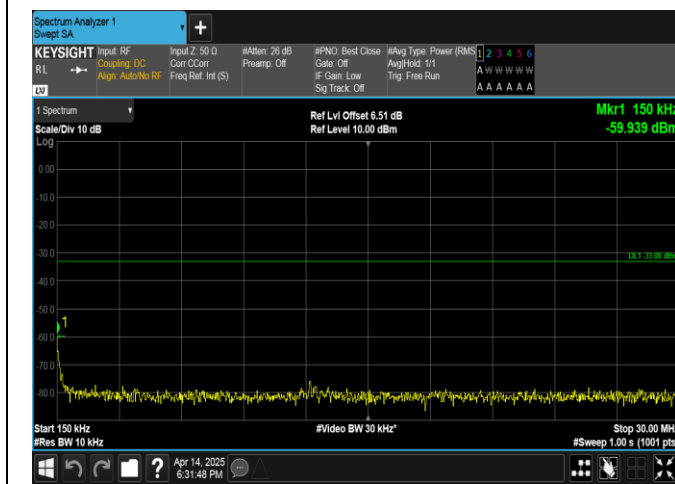
Band66-10MHz-QPSK-132322-50RB#0-0.15~30-PASS
