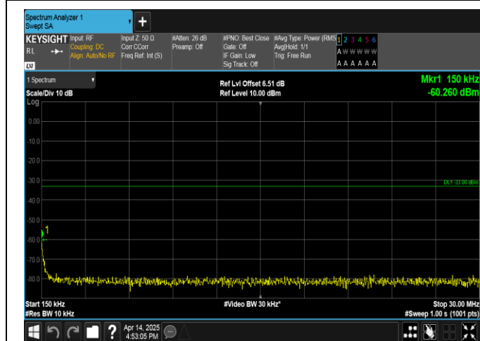
Band66-15MHz-QPSK-132322-1RB#0-0.15~30-PASS
