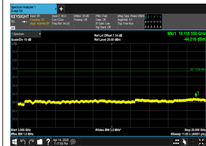
Band66-15MHz-QPSK-132047-75RB#0-3000~20000-PASS
