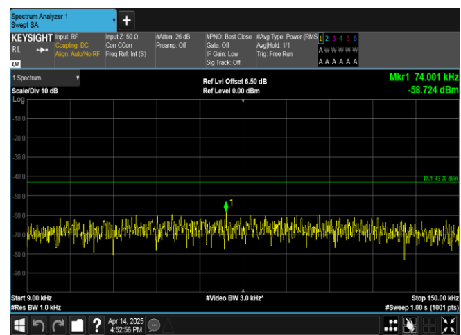
Band66-15MHz-QPSK-132322-1RB#0-0.009~0.15-PASS
