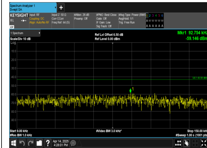
Band66-10MHz-16QAM-132622-1RB#49-0.009~0.15-PASS
