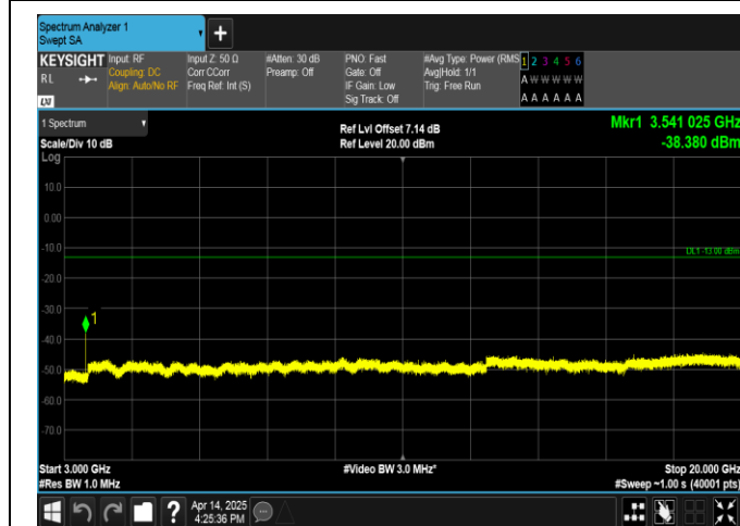
Band66-10MHz-QPSK-132622-1RB#0-3000~20000-PASS
