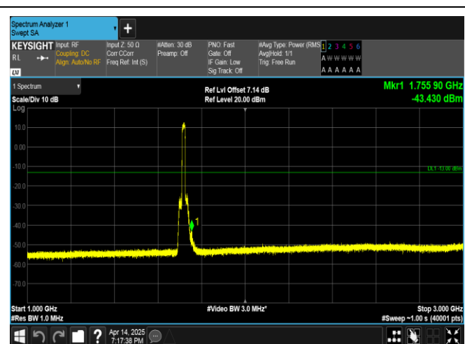
Band66-15MHz-QPSK-132047-75RB#0-1000~3000-PASS
