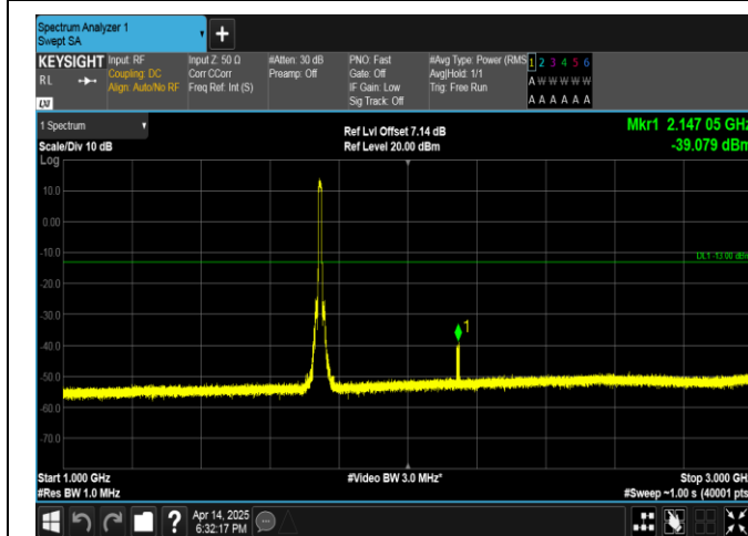
Band66-10MHz-QPSK-132322-50RB#0-1000~3000-PASS
