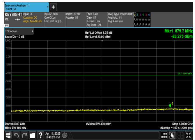
Band66-5MHz-16QAM-132647-25RB#0-30~1000-PASS
