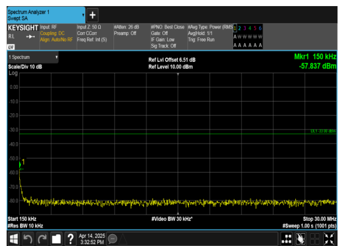
Band66-5MHz-16QAM-131997-1RB#24-0.15~30-PASS
