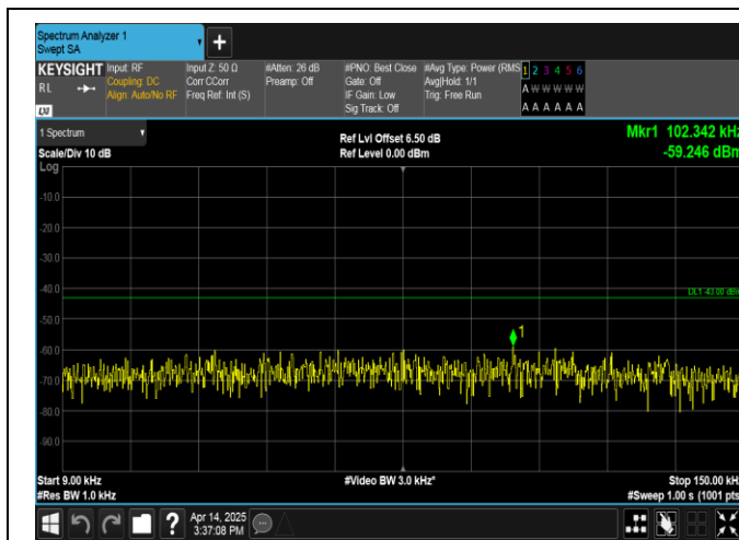
Band66-5MHz-16QAM-132322-1RB#0-0.009~0.15-PASS
