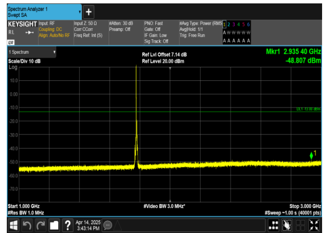
Band66-5MHz-QPSK-132647-1RB#0-1000~3000-PASS
