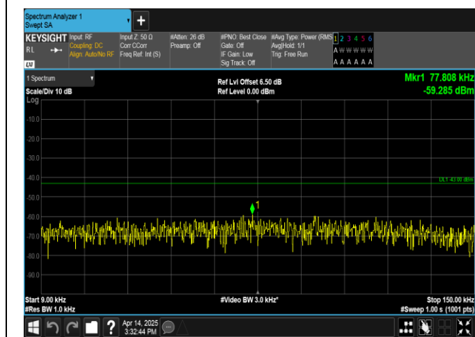
Band66-5MHz-16QAM-131997-1RB#24-0.009~0.15-PASS
