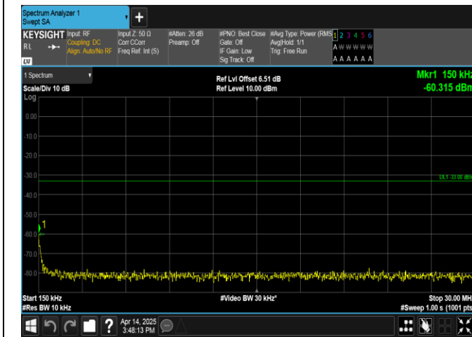
Band66-5MHz-16QAM-132647-25RB#0-0.15~30-PASS
