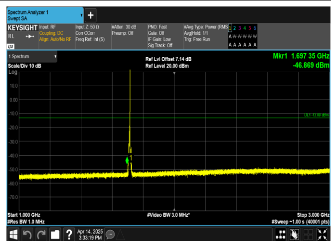
Band66-5MHz-16QAM-131997-1RB#24-1000~3000-PASS
