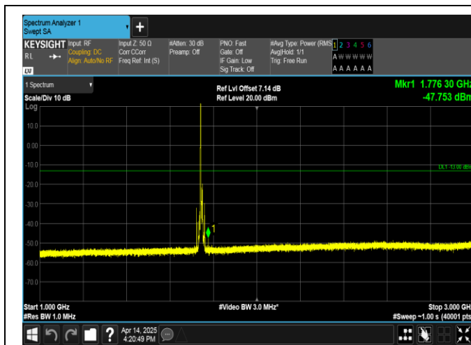
Band66-10MHz-QPSK-132322-1RB#0-1000~3000-PASS
