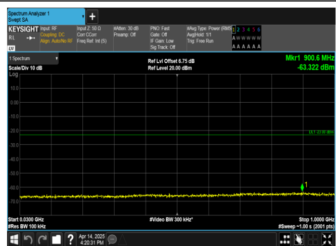
Band66-10MHz-QPSK-132322-1RB#0-30~1000-PASS
