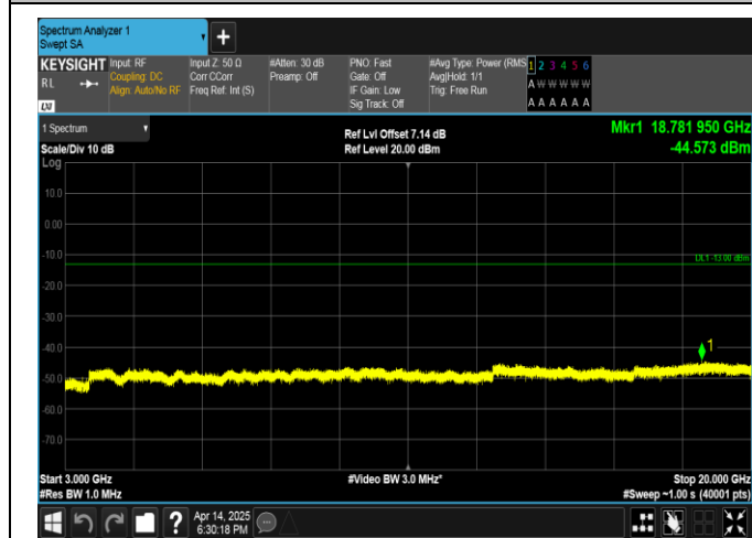
Band66-10MHz-QPSK-132022-50RB#0-3000~20000-PASS
