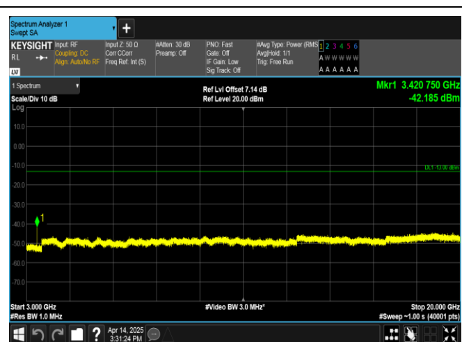
Band66-5MHz-16QAM-131997-1RB#0-3000~20000-PASS
