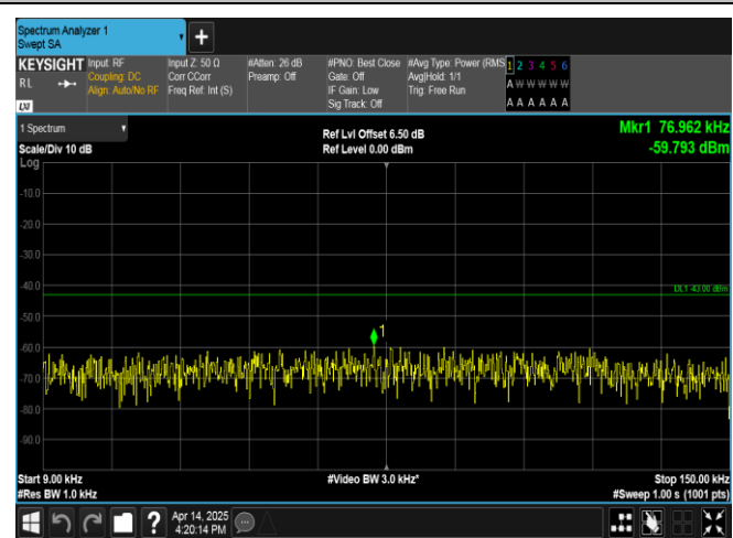
Band66-10MHz-QPSK-132322-1RB#0-0.009~0.15-PASS
