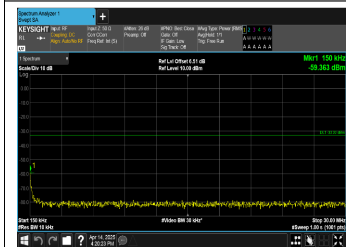
Band66-10MHz-QPSK-132322-1RB#0-0.15~30-PASS
