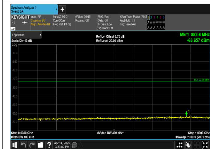
Band66-5MHz-16QAM-131997-1RB#24-30~1000-PASS
