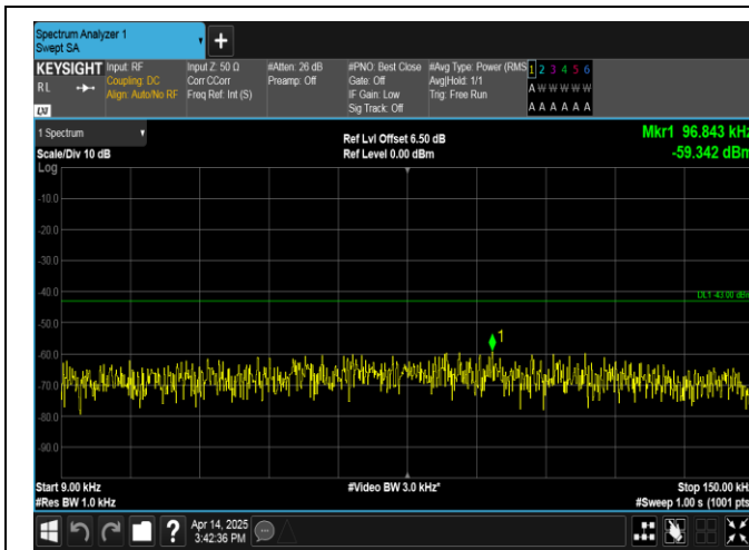
Band66-5MHz-QPSK-132647-1RB#0-0.009~0.15-PASS
