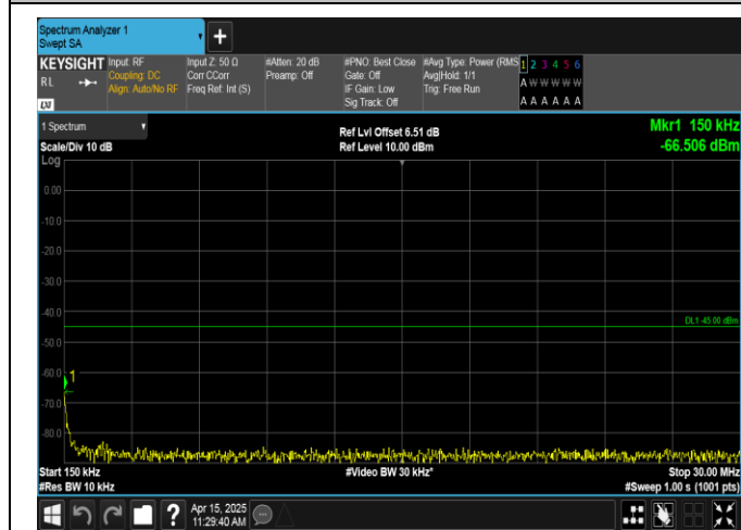
Band41-20MHz-16OAM-39750-1RB#0-0.15~30-PASS
