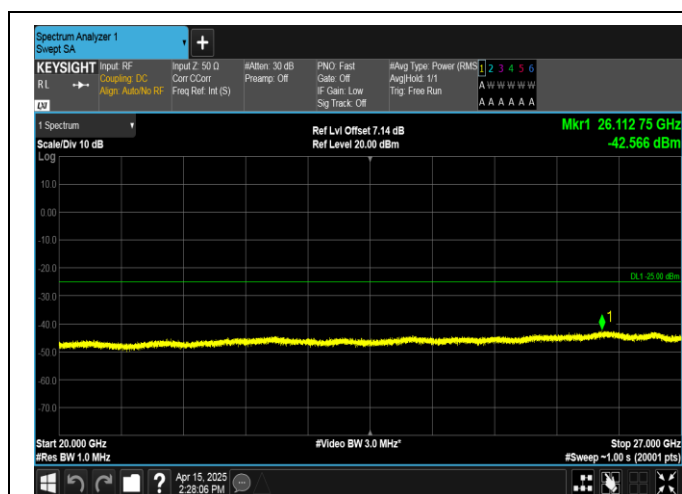
Band41-20MHz-OPSK-41490-100RB#0-20000~27000-PASS
