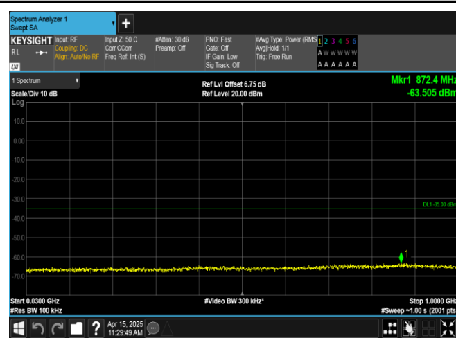
Band41-20MHz-16OAM-39750-1RB#0-30~1000-PASS
