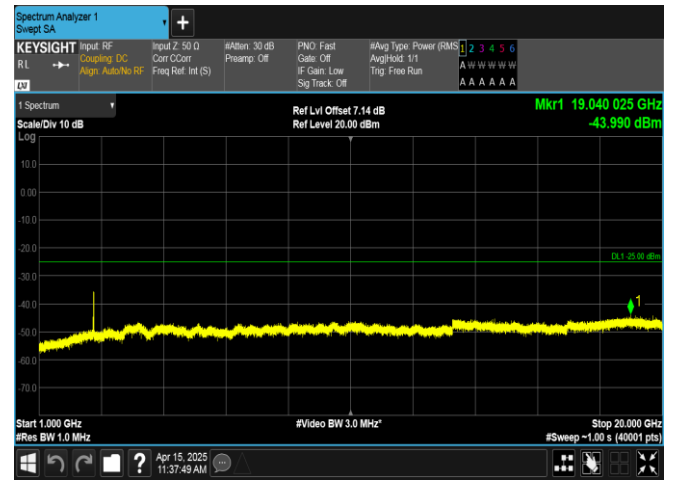
Band41-20MHz-QPSK-41490-1RB#0-1000~20000-PASS
