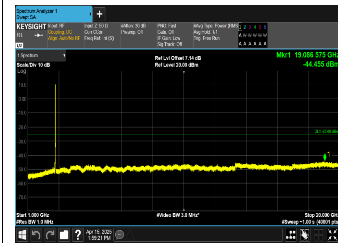
Band41-15MHz-16QAM-41515-75RB#0-1000~20000-PASS
