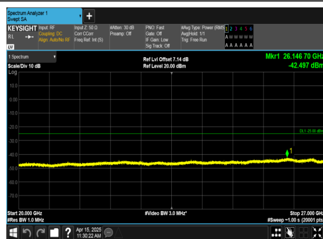
Band41-20MHz-16QAM-39750-1RB#0-20000~27000-PASS
