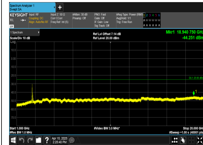
Band41-20MHz-QPSK-40620-100RB#0-1000~20000-PASS
