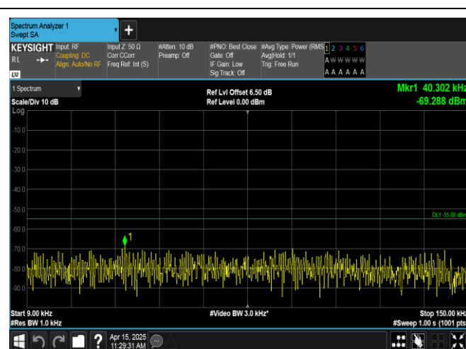
Band41-20MHz-16OAM-39750-1RB#0-0.009~0.15-PASS
