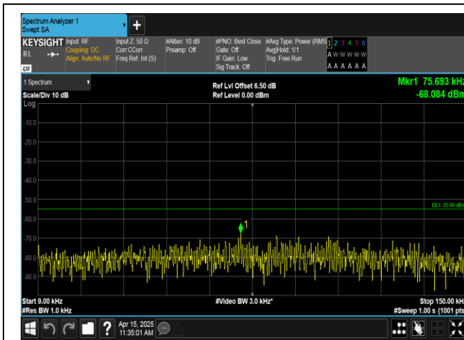
Band41-20MHz-QPSK-40620-1RB#99-0.009~0.15-PASS
