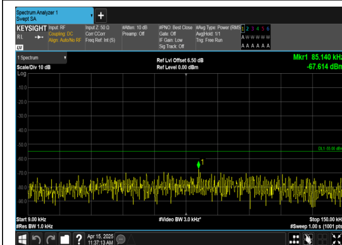
Band41-20MHz-QPSK-41490-1RB#0-0.009~0.15-PASS
