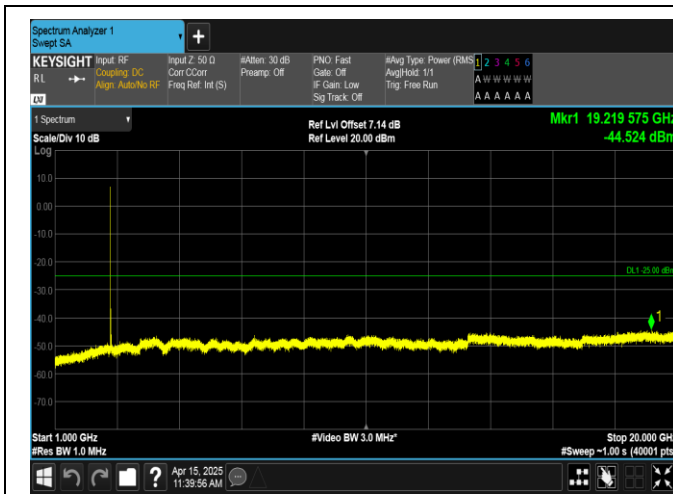
Band41-20MHz-QPSK-41490-1RB#99-1000~20000-PASS
