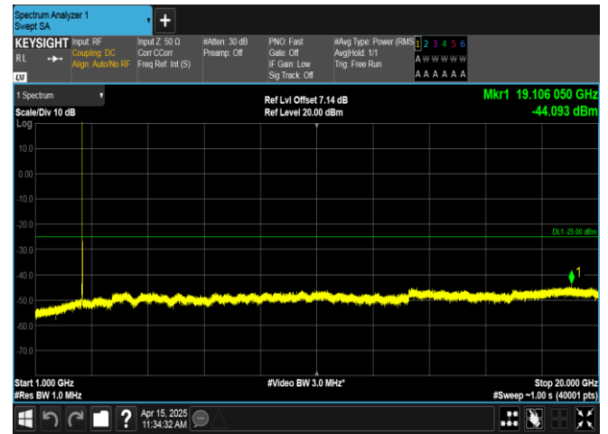
Band41-20MHz-16QAM-40620-1RB#0-1000~20000-PASS
