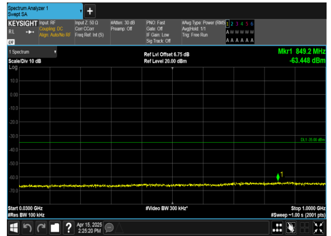
Band41-20MHz-QPSK-40620-100RB#0-30~1000-PASS
