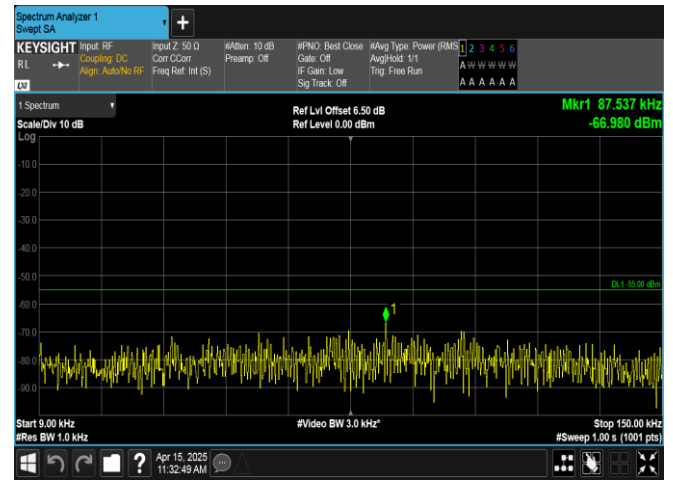
Band41-20MHz-QPSK-40620-1RB#0-0.009~0.15-PASS
