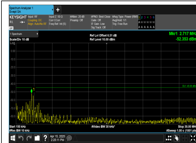
Band41-20MHz-QPSK-40620-100RB#0-0.15~30-PASS
