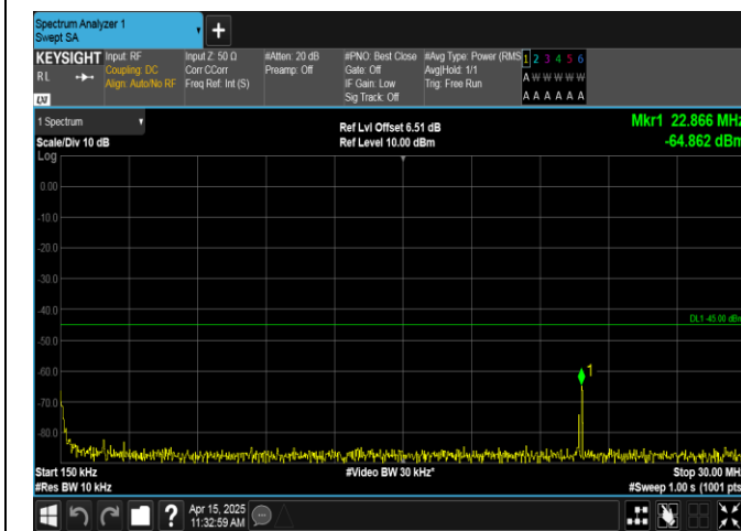
Band41-20MHz-QPSK-40620-1RB#0-0.15~30-PASS
