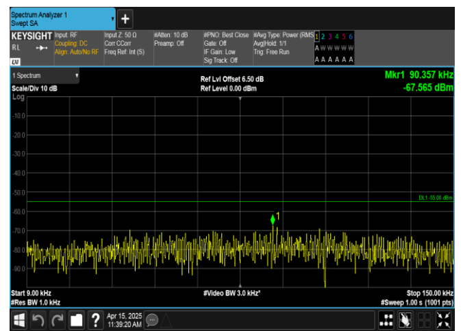
Band41-20MHz-QPSK-41490-1RB#99-0.009~0.15-PASS
