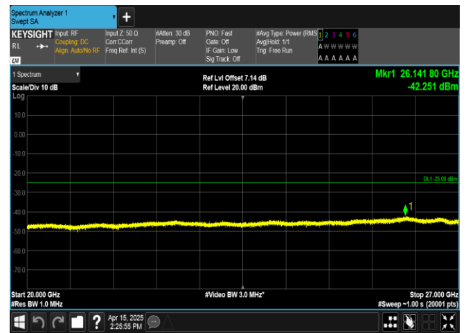
Band41-20MHz-QPSK-40620-100RB#0-20000~27000-PASS
