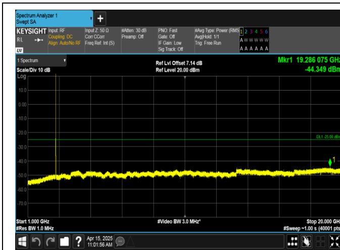
Band41-15MHz-QPSK-41515-1RB#74-1000~20000-PASS
