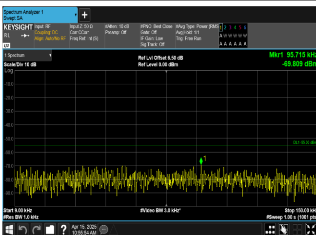
Band41-15MHz-16QAM-40620-1RB#0-0.009~0.15-PASS
