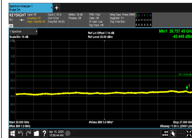
Band41-15MHz-16QAM-40620-1RB#0-20000~27000-PASS
