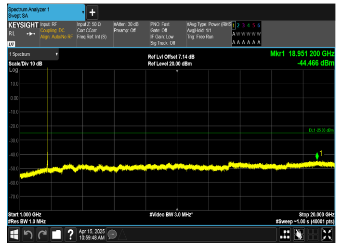
Band41-15MHz-QPSK-41515-1RB#0-1000~20000-PASS
