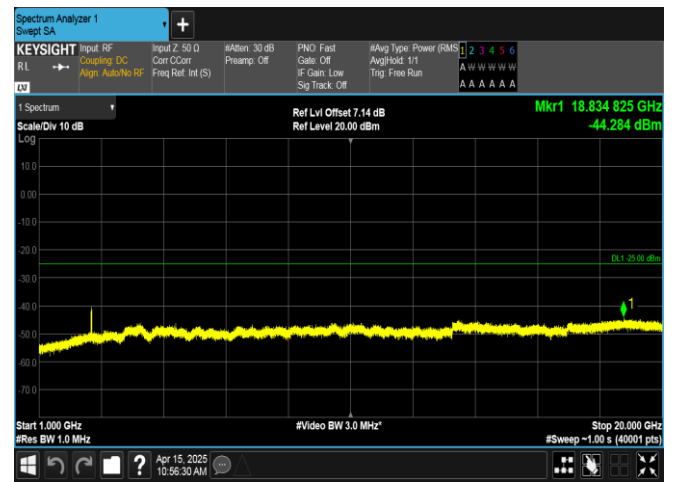
Band41-15MHz-16QAM-40620-1RB#0-1000~20000-PASS
