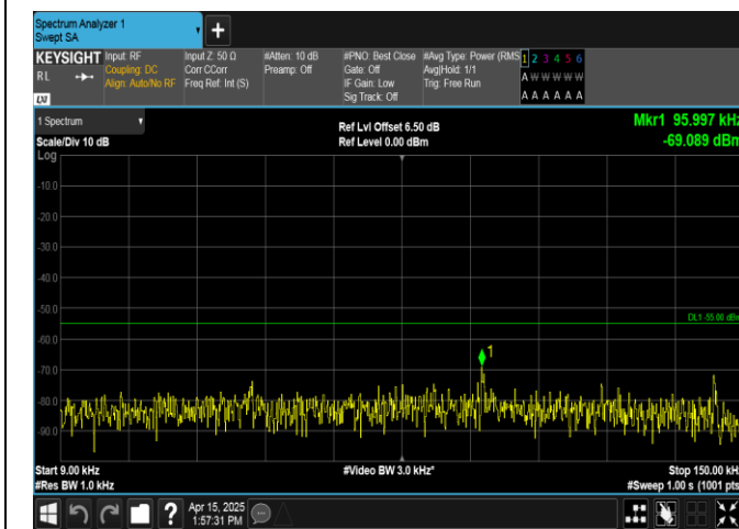
Band41-15MHz-QPSK-41515-75RB#0-0.009~0.15-PASS
