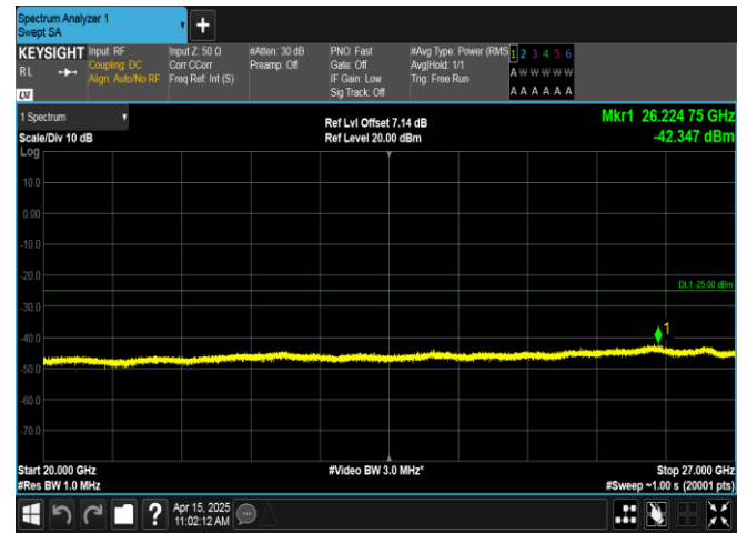
Band41-15MHz-QPSK-41515-1RB#74-20000~27000-PASS
