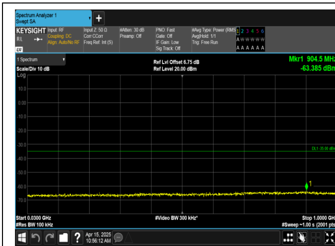
Band41-15MHz-16QAM-40620-1RB#0-30~1000-PASS
