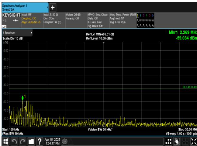
Band41-15MHz-16QAM-39725-75RB#0-0.15~30-PASS
