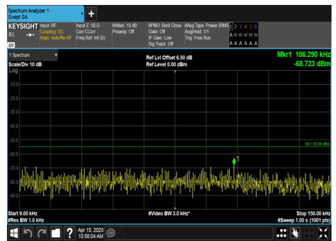
Band41-15MHz-16QAM-40620-1RB#74-0.009~0.15-PASS
