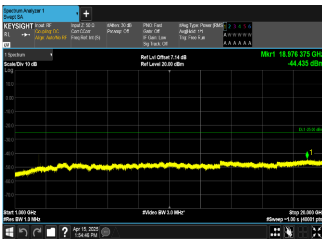
Band41-15MHz-16QAM-39725-75RB#0-1000~20000-PASS
