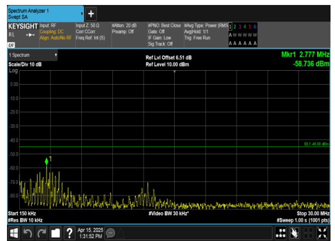
Band41-10MHz-QPSK-41540-50RB#0-0.15~30-PASS
