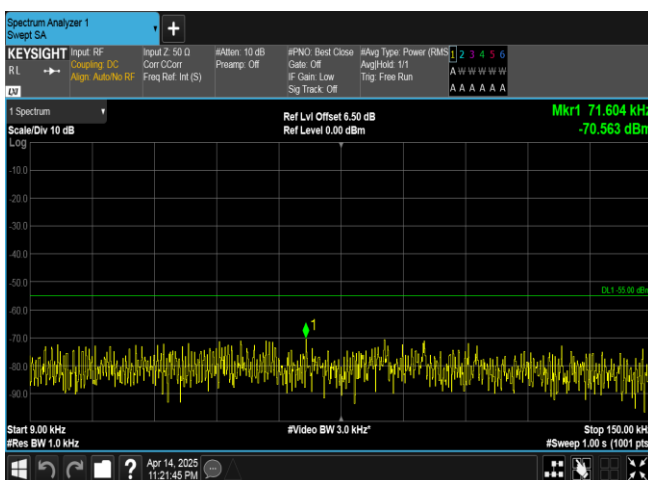
Band41-10MHz-16QAM-40620-1RB#0-0.009~0.15-PASS
