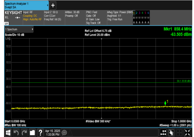
Band41-10MHz-16QAM-41540-50RB#0-30~1000-PASS
