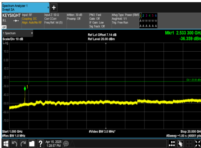
Band41-10MHz-16QAM-39700-50RB#0-1000~20000-PASS
