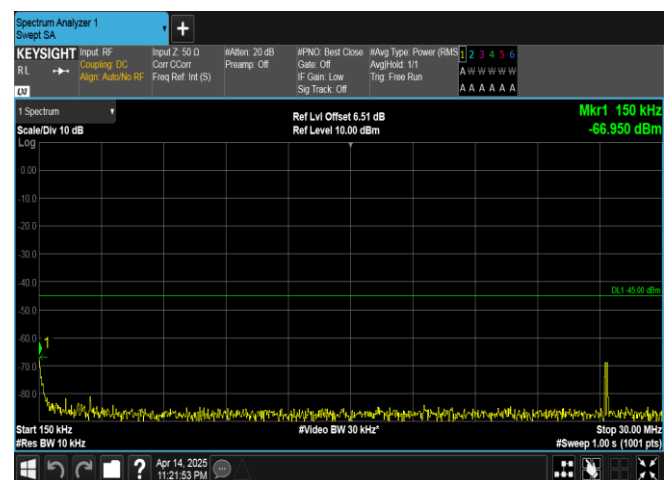
Band41-10MHz-16QAM-40620-1RB#0-0.15~30-PASS
