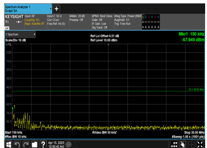
Band41-15MHz-QPSK-39725-1RB#0-0.15~30-PASS
