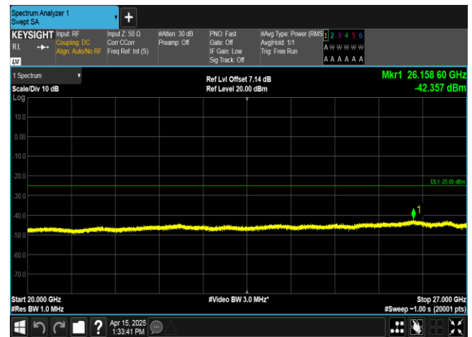
Band41-10MHz-16QAM-41540-50RB#0-20000~27000-PASS
