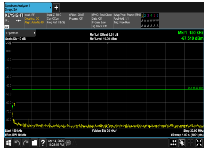
Band41-10MHz-16QAM-41540-1RB#49-0.15~30-PASS
