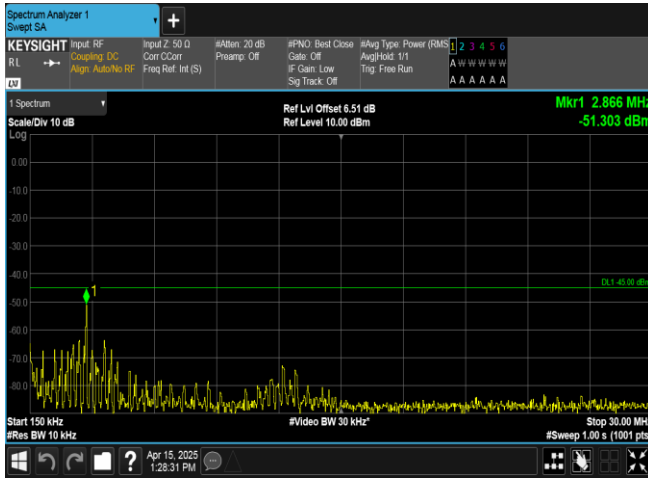
Band41-10MHz-16QAM-39700-50RB#0-0.15~30-PASS
