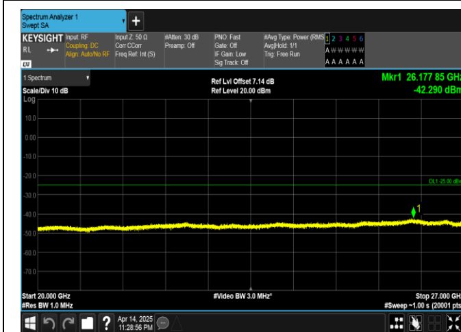
Band41-10MHz-16QAM-41540-1RB#49-20000~27000-PASS
