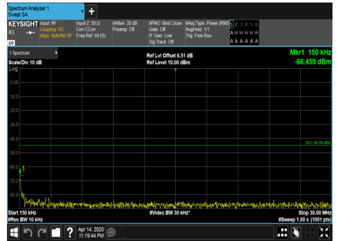
Band41-10MHz-16QAM-39700-1RB#49-0.15~30-PASS
