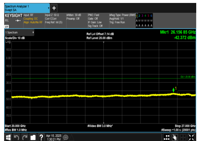
Band41-10MHz-QPSK-40620-50RB#0-20000~27000-PASS
