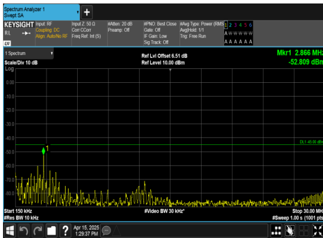
Band41-10MHz-QPSK-40620-50RB#0-0.15~30-PASS
