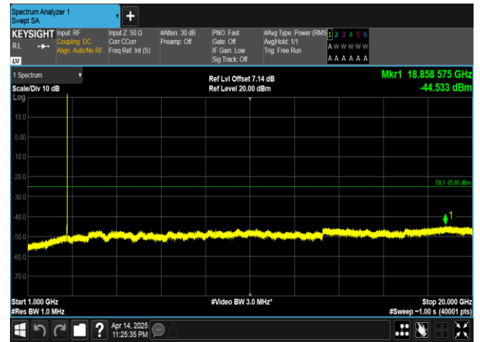
Band41-10MHz-QPSK-41540-1RB#0-1000~20000-PASS
