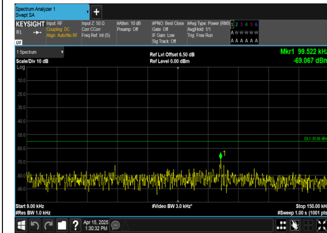
Band41-10MHz-16QAM-40620-50RB#0-0.009~0.15-PASS
