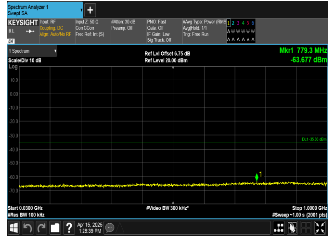
Band41-10MHz-16QAM-39700-50RB#0-30~1000-PASS
