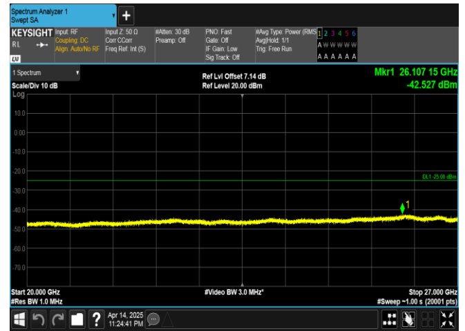
Band41-10MHz-16QAM-40620-1RB#49-20000~27000-PASS
