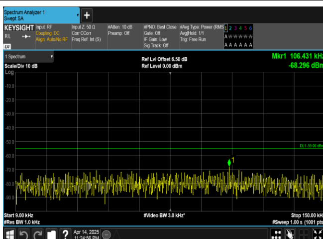
Band41-10MHz-QPSK-41540-1RB#0-0.009~0.15-PASS
