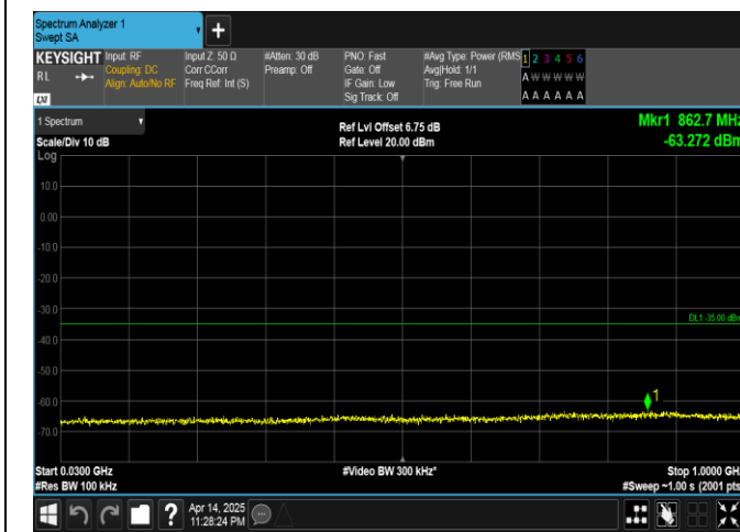
Band41-10MHz-16QAM-41540-1RB#49-30~1000-PASS
