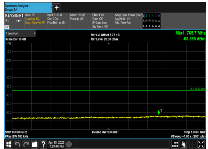
Band41-10MHz-QPSK-40620-50RB#0-30~1000-PASS
