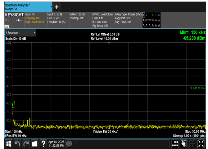
Band41-10MHz-QPSK-40620-1RB#49-0.15~30-PASS
