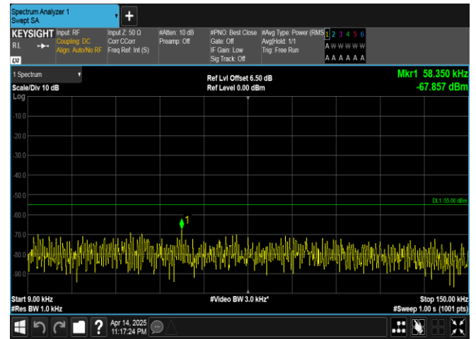
Band41-10MHz-16QAM-39700-1RB#0-0.009~0.15-PASS
