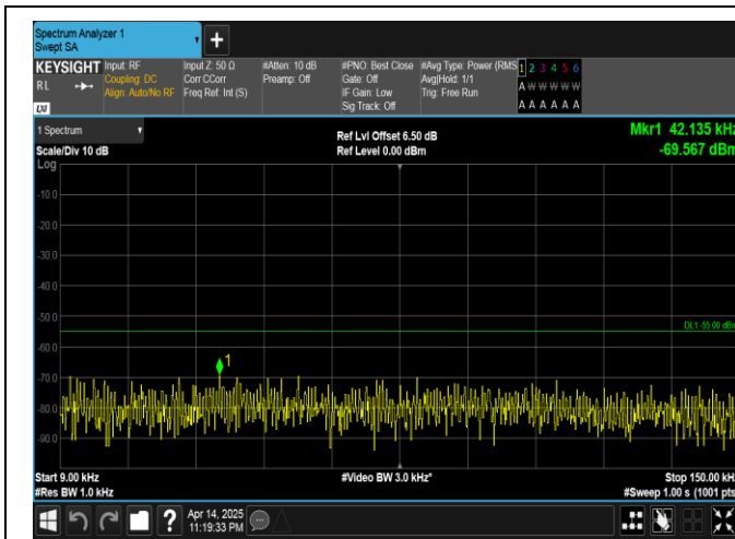
Band41-10MHz-16QAM-39700-1RB#49-0.009~0.15-PASS
