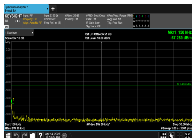
Band41-10MHz-QPSK-41540-1RB#0-0.15~30-PASS
