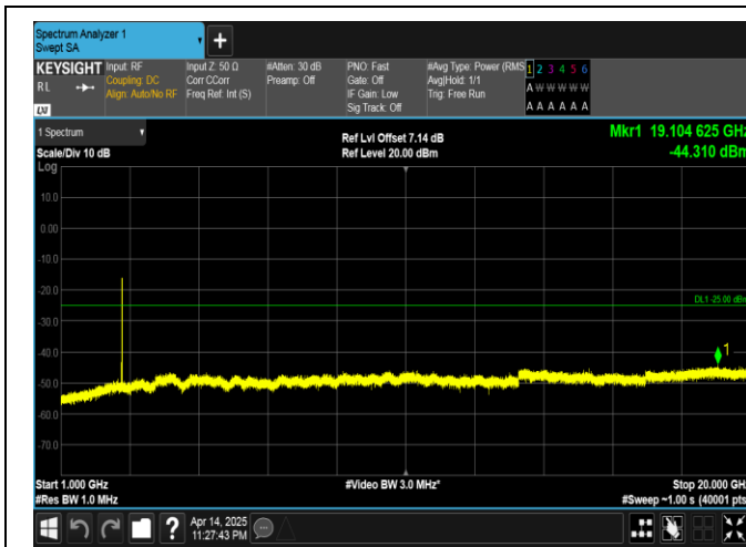
Band41-10MHz-QPSK-41540-1RB#49-1000~20000-PASS
