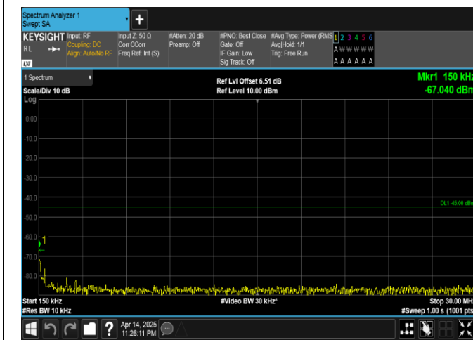
Band41-10MHz-16QAM-41540-1RB#0-0.15~30-PASS
