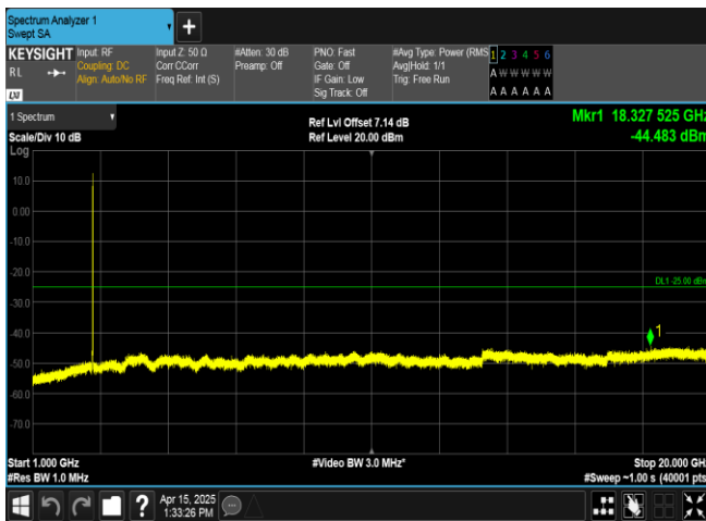
Band41-10MHz-16QAM-41540-50RB#0-1000~20000-PASS
