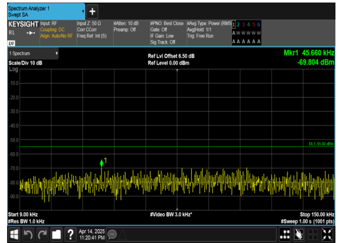
Band41-10MHz-QPSK-40620-1RB#0-0.009~0.15-PASS
