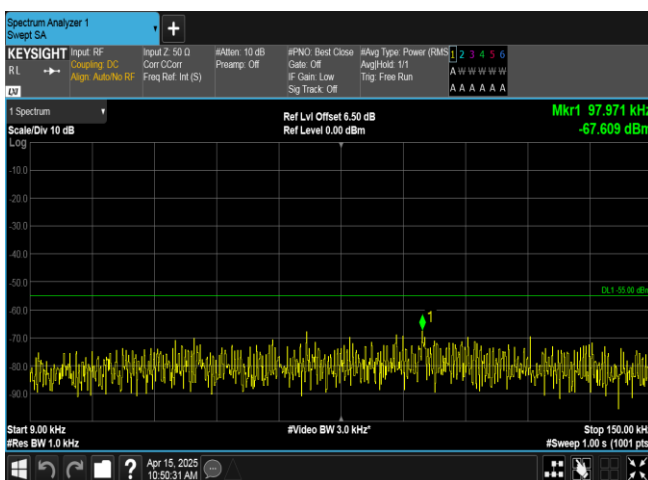
Band41-15MHz-QPSK-39725-1RB#0-0.009~0.15-PASS
