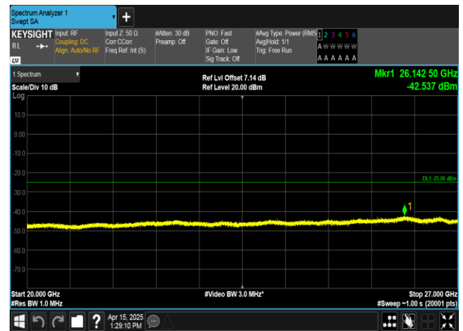
Band41-10MHz-16QAM-39700-50RB#0-20000~27000-PASS
