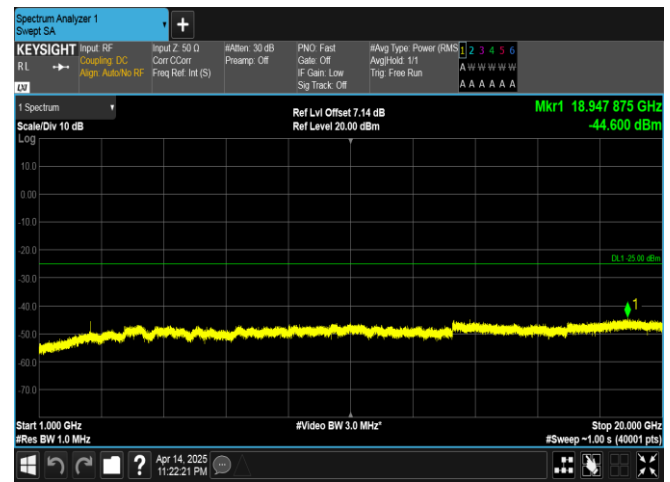
Band41-10MHz-16QAM-40620-1RB#0-1000~20000-PASS
