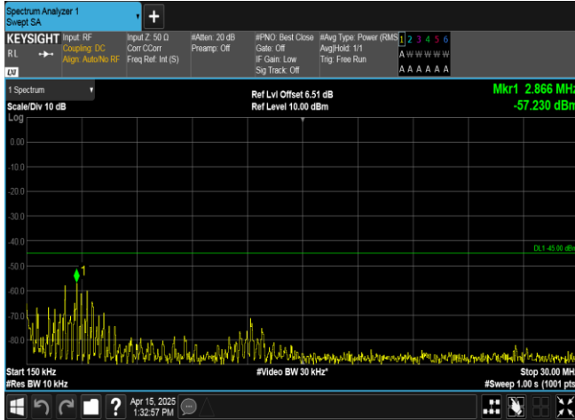
Band41-10MHz-16QAM-41540-50RB#0-0.15~30-PASS
