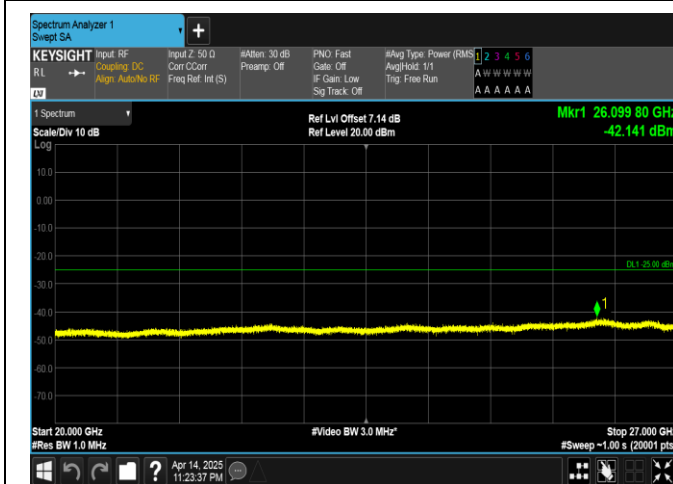
Band41-10MHz-QPSK-40620-1RB#49-20000~27000-PASS
