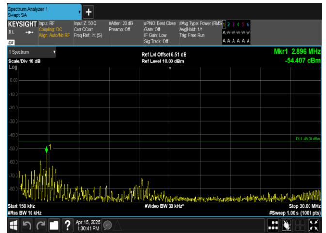
Band41-10MHz-16QAM-40620-50RB#0-0.15~30-PASS
