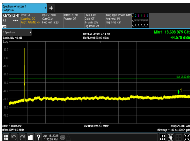
Band41-10MHz-QPSK-40620-50RB#0-1000~20000-PASS
