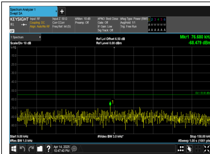
Band41-5MHz-16QAM-41565-1RB#24-0.009~0.15-PASS
