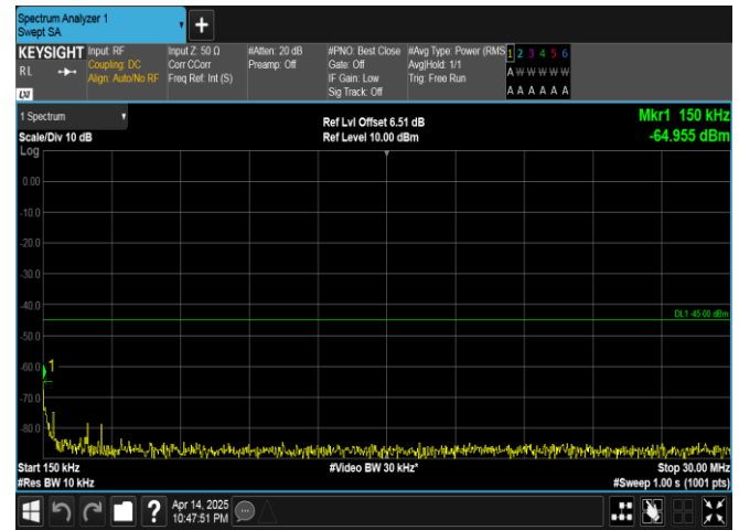
Band41-5MHz-16QAM-41565-1RB#24-0.15~30-PASS
