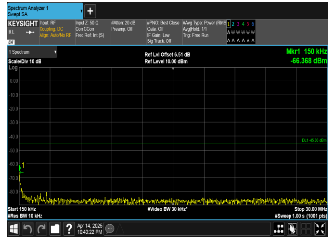
Band41-5MHz-QPSK-40620-1RB#24-0.15~30-PASS
