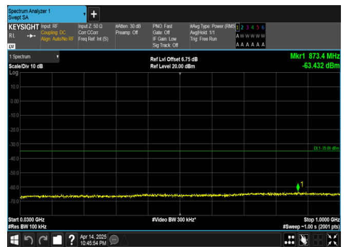
Band41-5MHz-16QAM-41565-1RB#0-30~1000-PASS
