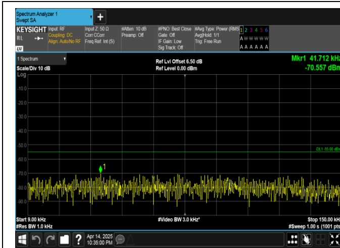
Band41-5MHz-16QAM-39675-1RB#24-0.009~0.15-PASS
