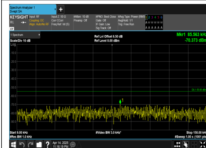
Band41-10MHz-QPSK-39700-1RB#0-0.009~0.15-PASS
