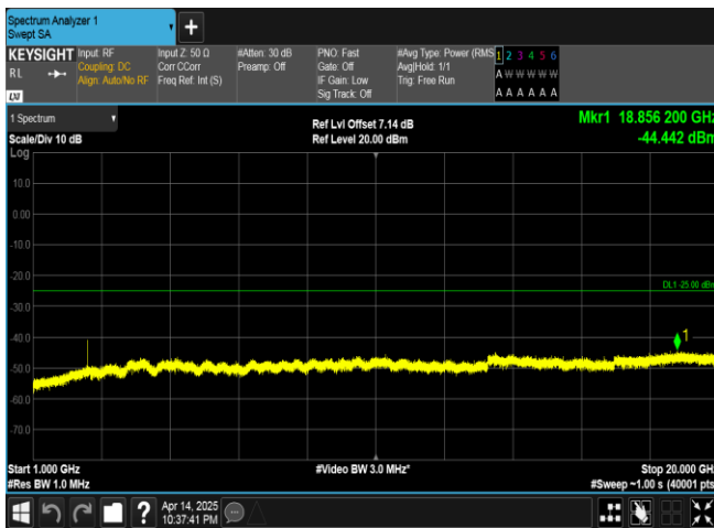
Band41-5MHz-16QAM-39675-25RB#0-1000~20000-PASS
