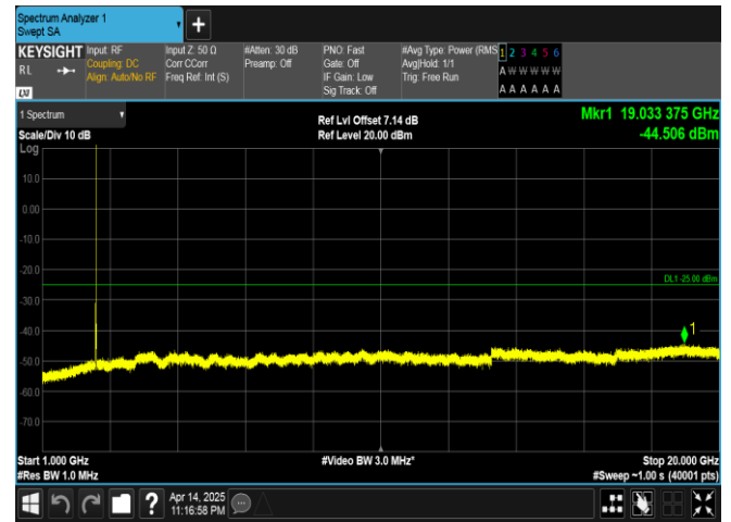
Band41-10MHz-QPSK-39700-1RB#0-1000~20000-PASS
