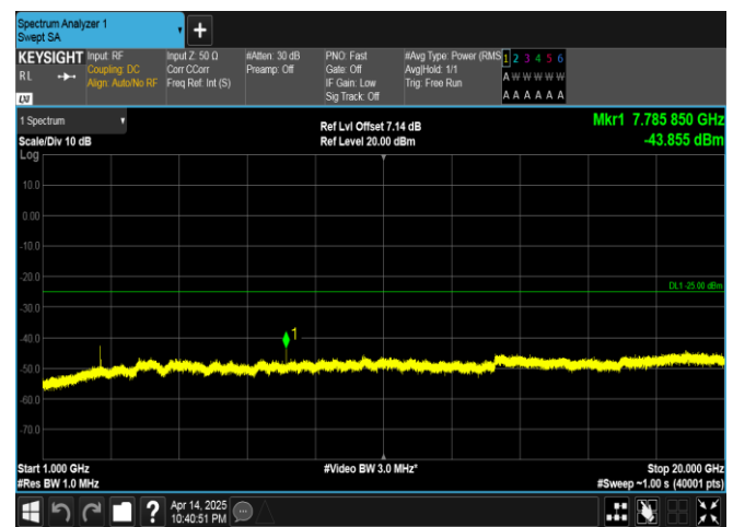
Band41-5MHz-QPSK-40620-1RB#24-1000~20000-PASS
