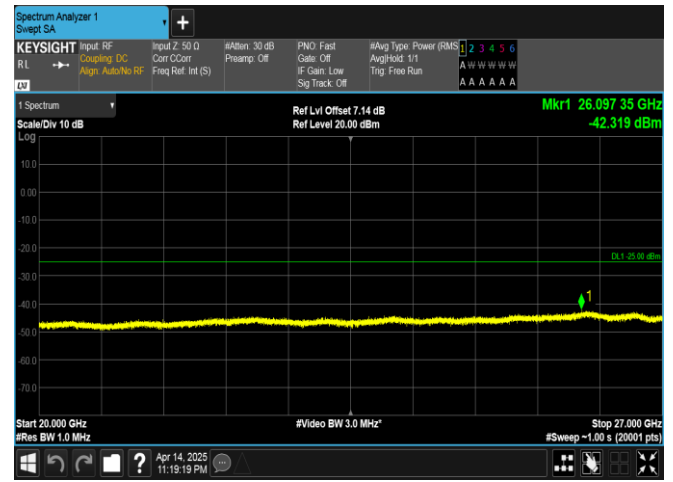
Band41-10MHz-QPSK-39700-1RB#49-20000~27000-PASS
