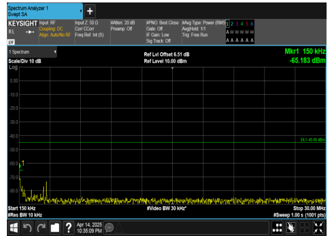
Band41-5MHz-16QAM-39675-1RB#24-0.15~30-PASS
