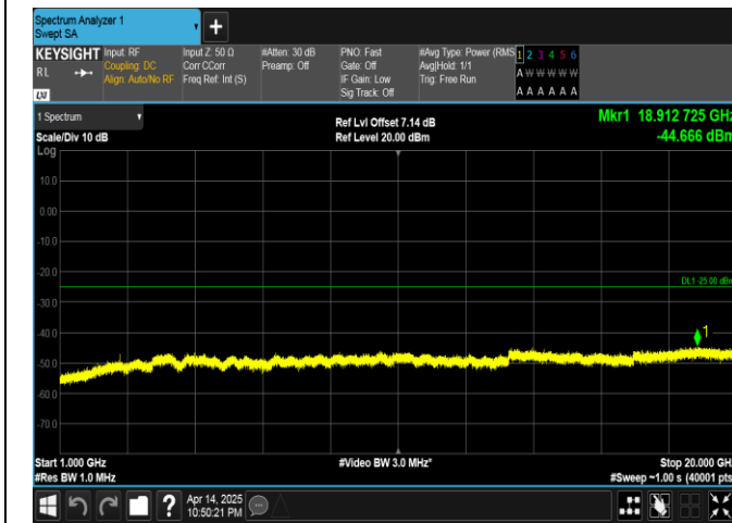
Band41-5MHz-16QAM-41565-25RB#0-1000~20000-PASS
