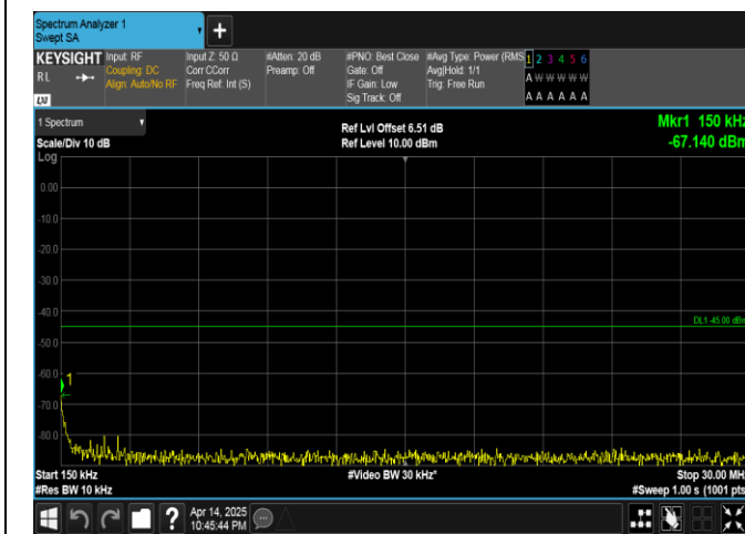
Band41-5MHz-16QAM-41565-1RB#0-0.15~30-PASS
