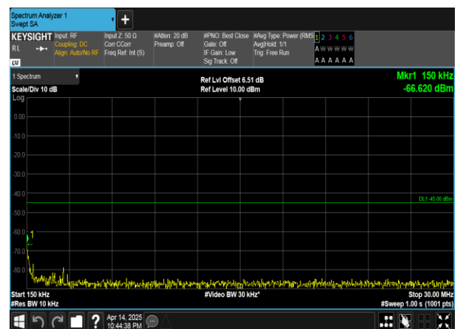
Band41-5MHz-QPSK-41565-1RB#0-0.15~30-PASS
