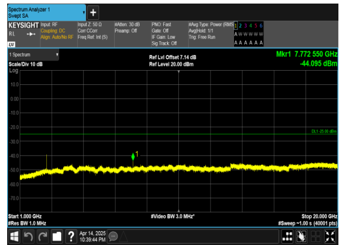
Band41-5MHz-16QAM-40620-1RB#0-1000~20000-PASS
