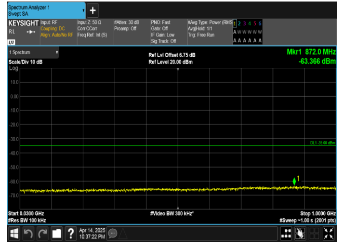
Band41-5MHz-16QAM-39675-25RB#0-30~1000-PASS
