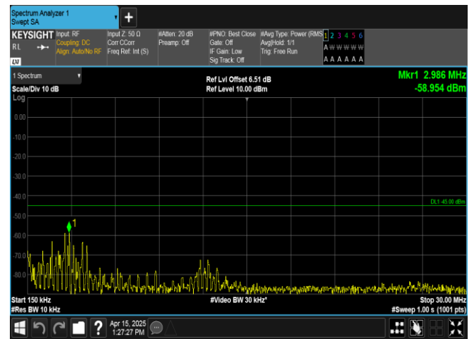
Band41-10MHz-QPSK-39700-50RB#0-0.15~30-PASS
