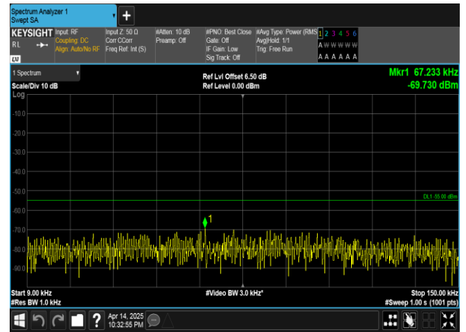
Band41-5MHz-16QAM-39675-1RB#0-0.009~0.15-PASS
