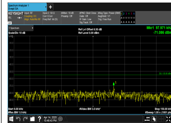
Band41-5MHz-QPSK-41565-25RB#0-0.009~0.15-PASS
