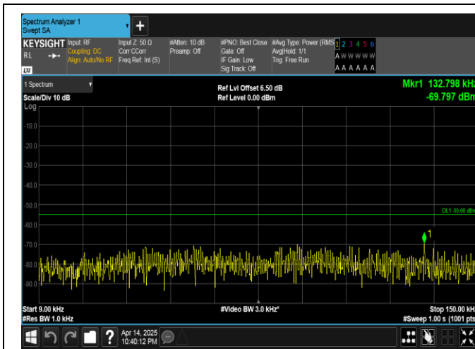
Band41-5MHz-QPSK-40620-1RB#24-0.009~0.15-PASS
