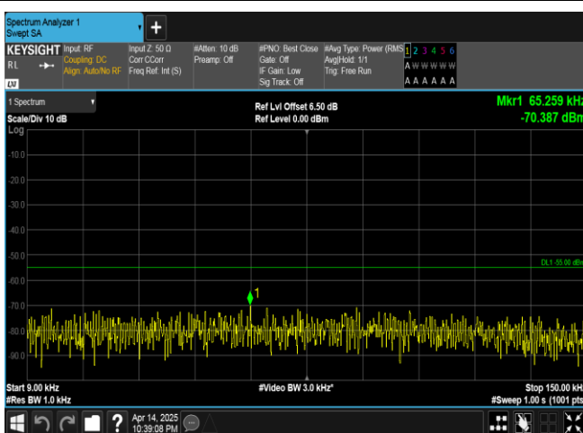
Band41-5MHz-16QAM-40620-1RB#0-0.009~0.15-PASS
