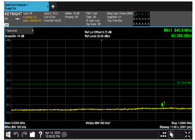
Band41-5MHz-16QAM-41565-25RB#0-30~1000-PASS
