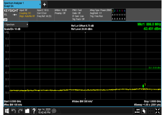
Band41-5MHz-QPSK-40620-25RB#0-30~1000-PASS
