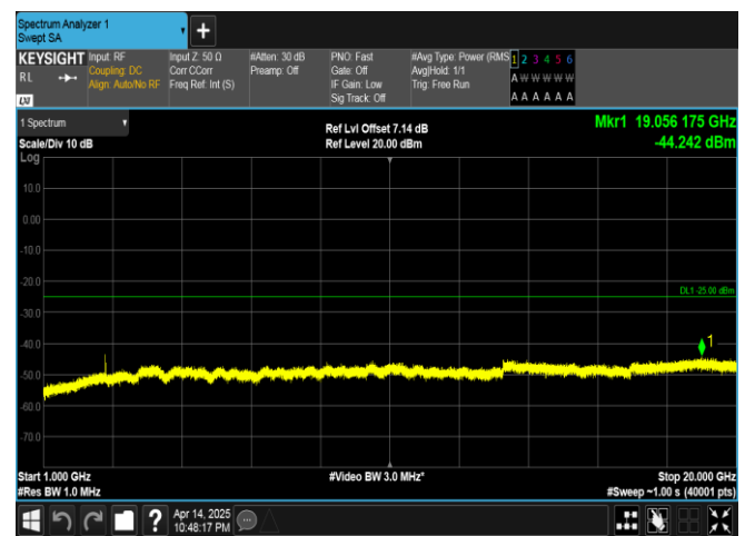
Band41-5MHz-16QAM-41565-1RB#24-1000~20000-PASS
