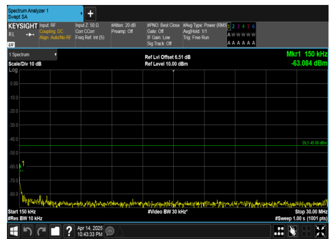
Band41-5MHz-16QAM-40620-25RB#0-0.15~30-PASS
