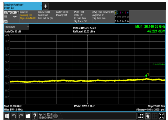
Band41-5MHz-16QAM-41565-25RB#0-20000~27000-PASS
