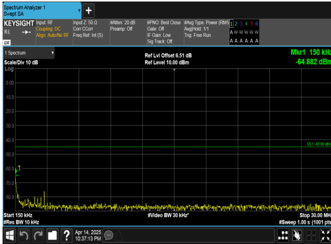
Band41-5MHz-16QAM-39675-25RB#0-0.15~30-PASS
