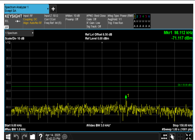
Band41-5MHz-QPSK-40620-25RB#0-0.009~0.15-PASS
