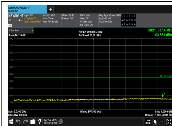
Band41-5MHz-16QAM-40620-1RB#0-30~1000-PASS
