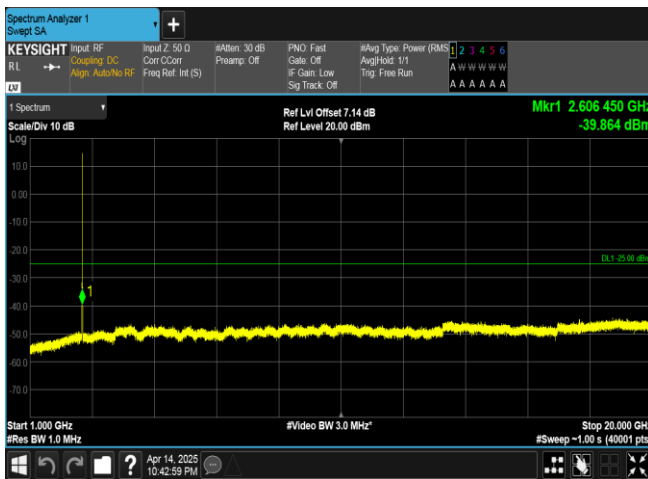
Band41-5MHz-QPSK-40620-25RB#0-1000~20000-PASS
