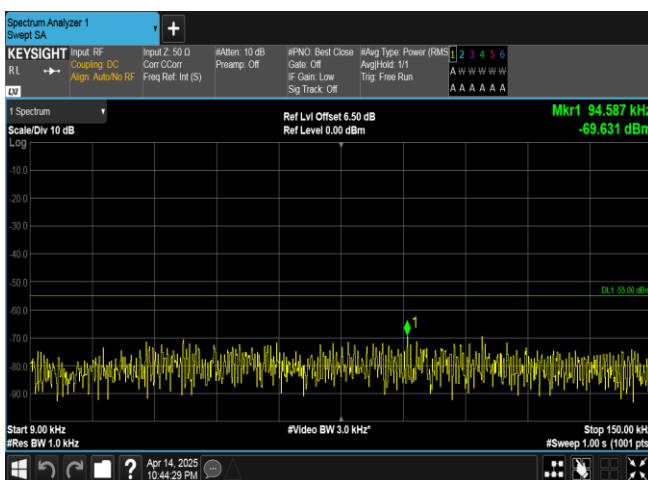
Band41-5MHz-QPSK-41565-1RB#0-0.009~0.15-PASS
