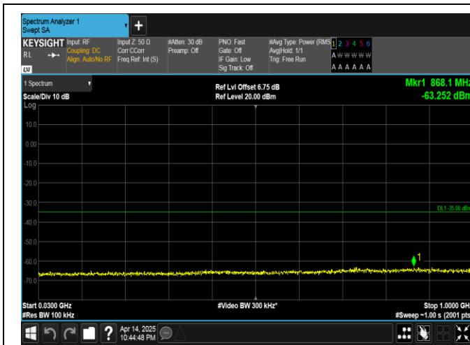
Band41-5MHz-QPSK-41565-1RB#0-30~1000-PASS
