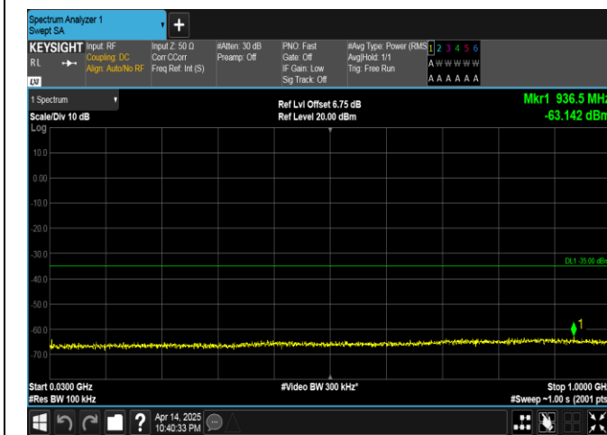
Band41-5MHz-QPSK-40620-1RB#24-30~1000-PASS
