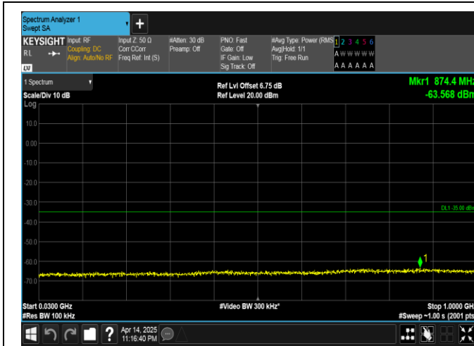
Band41-10MHz-QPSK-39700-1RB#0-30~1000-PASS
