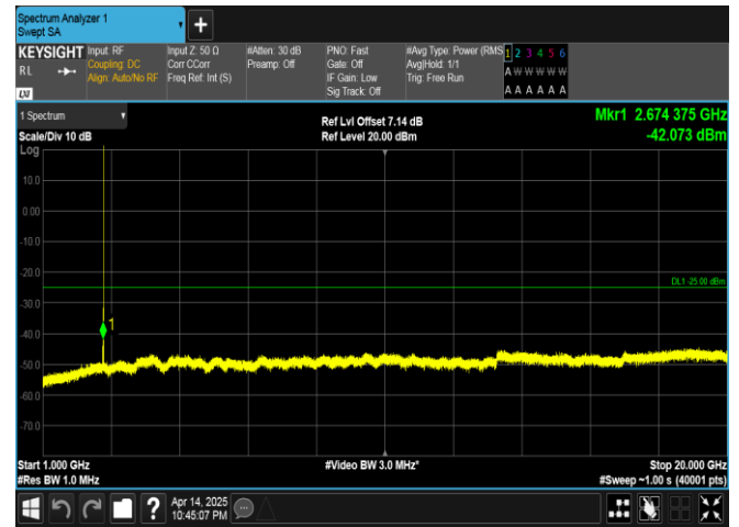
Band41-5MHz-QPSK-41565-1RB#0-1000~20000-PASS
