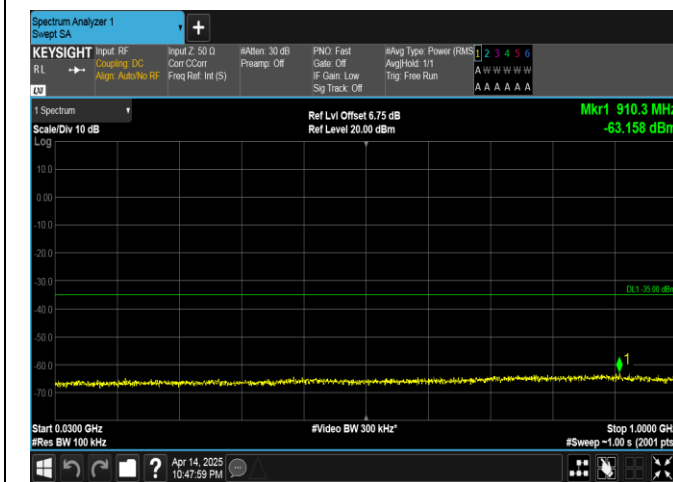
Band41-5MHz-16QAM-41565-1RB#24-30~1000-PASS
