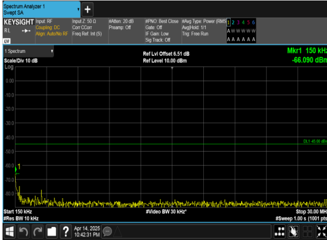
Band41-5MHz-QPSK-40620-25RB#0-0.15~30-PASS
