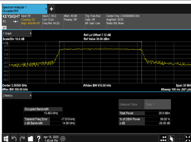
Band41-15MHz-16QAM-40620-75RB#0-PASS
