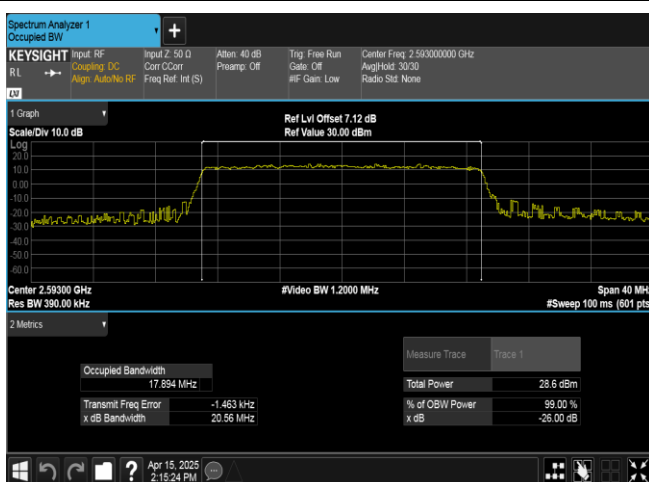
Band41-20MHz-16QAM-40620-100RB#0-PASS
