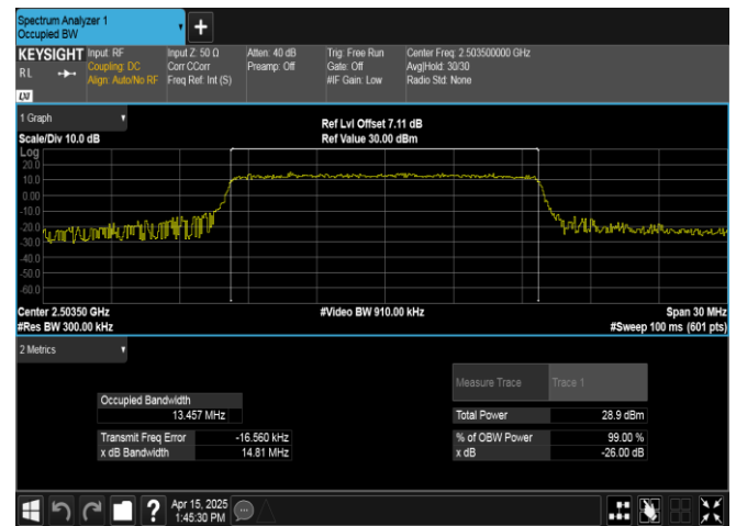
Band41-15MHz-16QAM-39725-75RB#0-PASS
