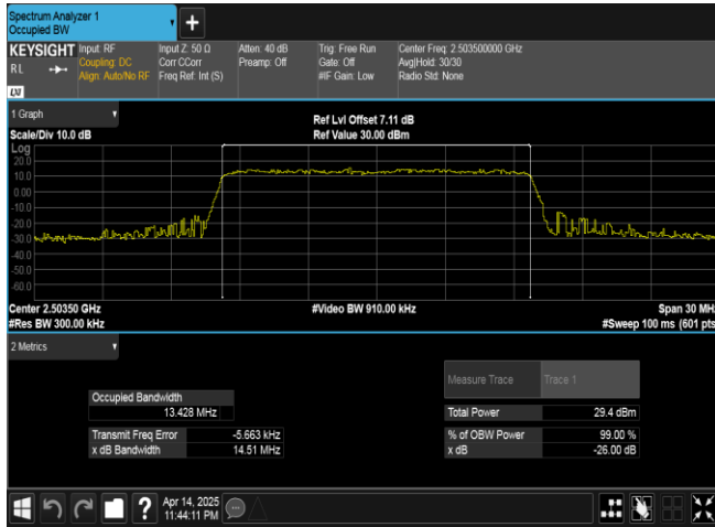
Band41-15MHz-QPSK-39725-75RB#0-PASS
