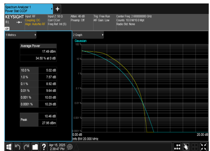
Band41-20MHz-QPSK-41490-100RB#0-PASS
