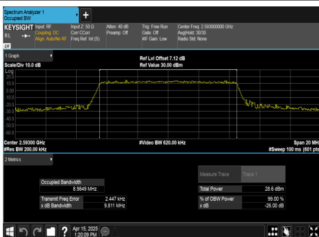
Band41-10MHz-16QAM-40620-50RB#0-PASS
