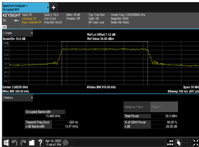
Band41-15MHz-QPSK-41515-75RB#0-PASS
