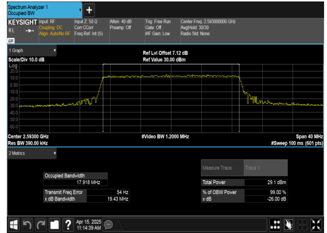
Band41-20MHz-QPSK-40620-100RB#0-PASS
