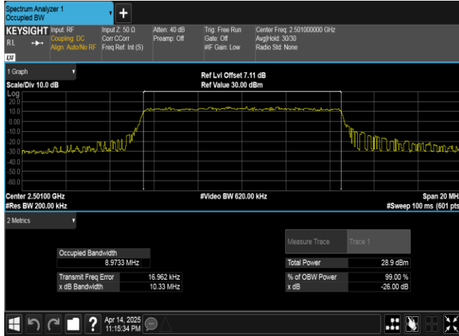
Band41-10MHz-QPSK-39700-50RB#0-PASS
