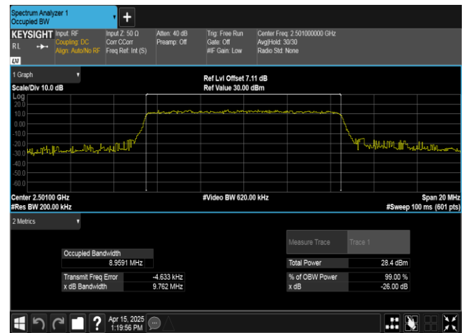
Band41-10MHz-16QAM-39700-50RB#0-PASS
