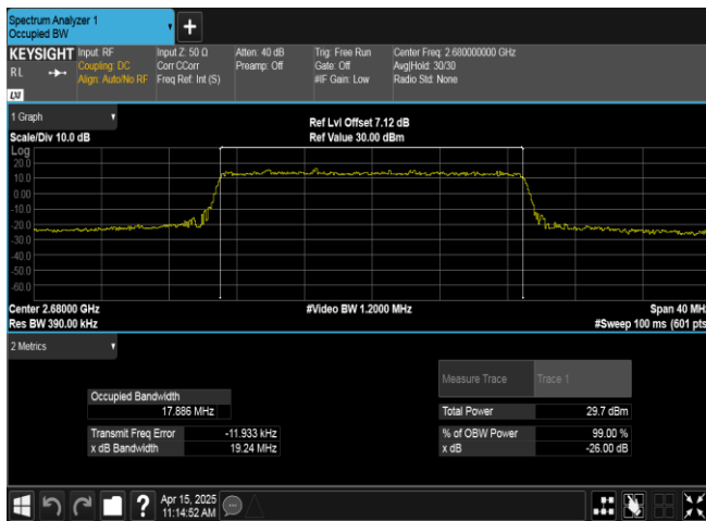
Band41-20MHz-QPSK-41490-100RB#0-PASS
