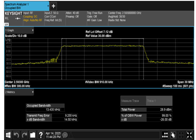
Band41-15MHz-QPSK-40620-75RB#0-PASS
