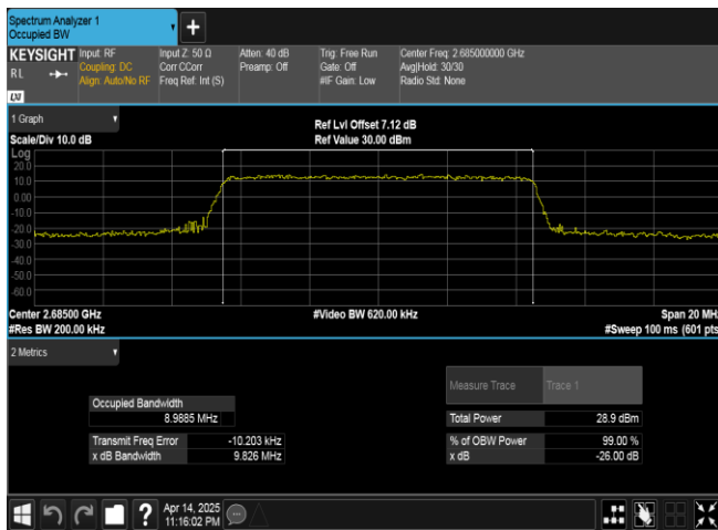
Band41-10MHz-QPSK-41540-50RB#0-PASS
