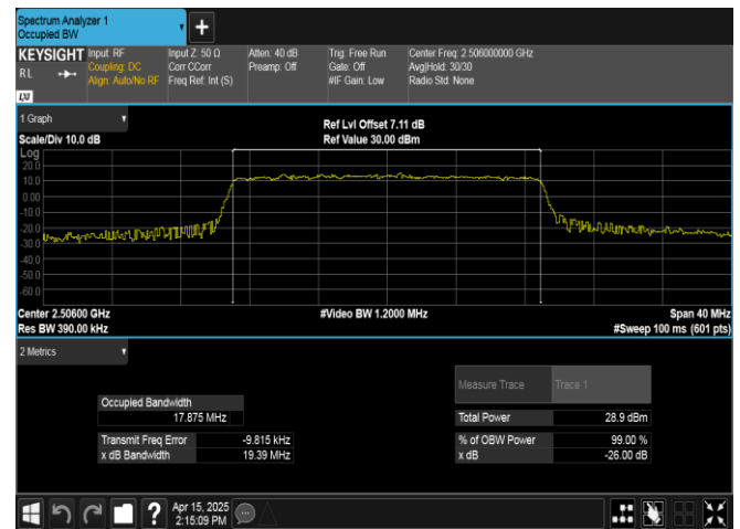
Band41-20MHz-16QAM-39750-100RB#0-PASS
