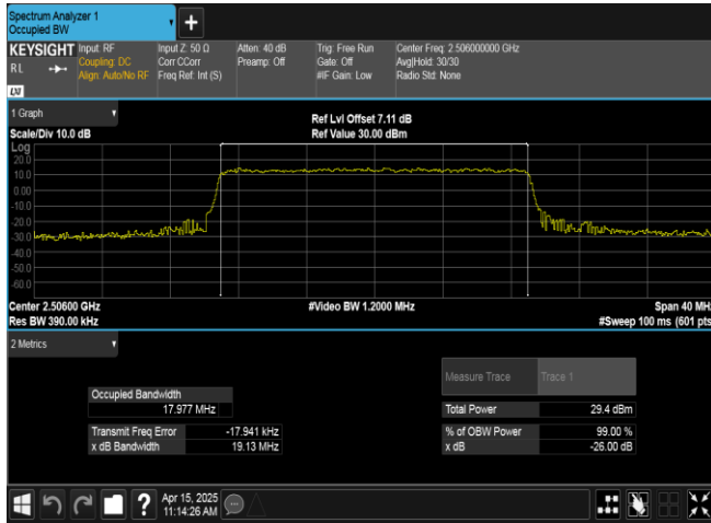
Band41-20MHz-QPSK-39750-100RB#0-PASS
