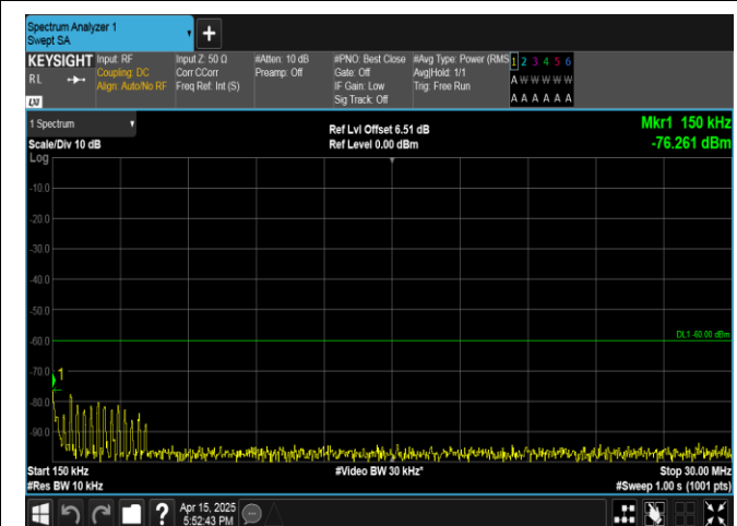
Band40(2350-2360)-5MHz-QPSK-39175-25RB#0-0.15~30-PASS
