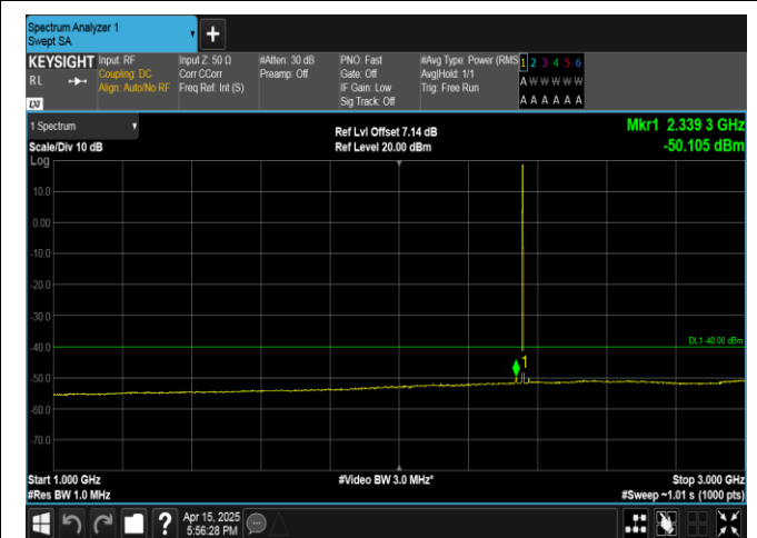
Band40(2350-2360)-5MHz-QPSK-39200-1RB#24-1000-3000-PASS
