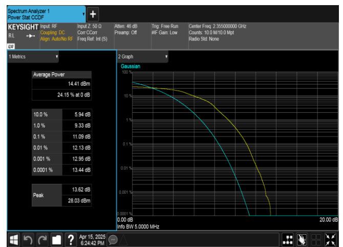
Band40(2350-2360)-5MHz-16QAM-39200-25RB#0-PASS
