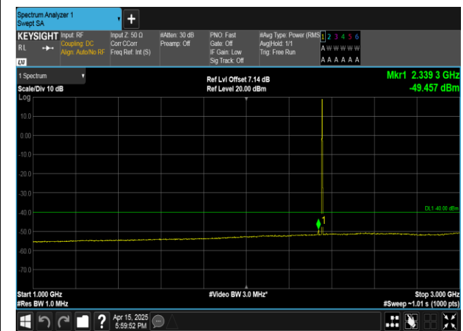
Band40(2350-2360)-5MHz-QPSK-39225-1RB#0-1000~3000-PASS
