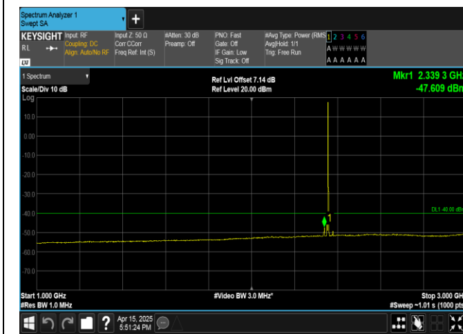
Band40(2350-2360)-5MHz-QPSK-39175-1RB#24-1000~3000-PASS
