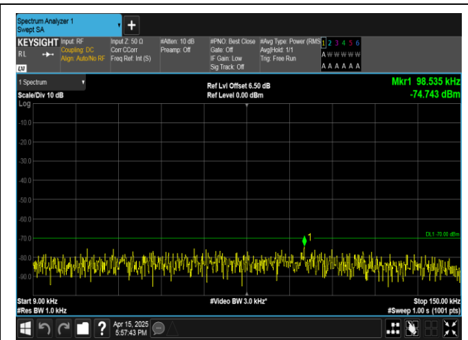
Band40(2350-2360)-5MHz-QPSK-39200-25RB#0-0.009-0.15-PASS
