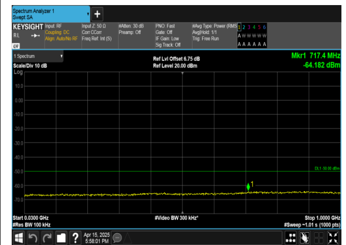
Band40(2350-2360)-5MHz-QPSK-39200-25RB#0-30-1000-PASS
