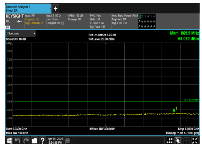
Band40(2350-2360)-5MHz-QPSK-39200-1RB#0-30~1000-PASS
