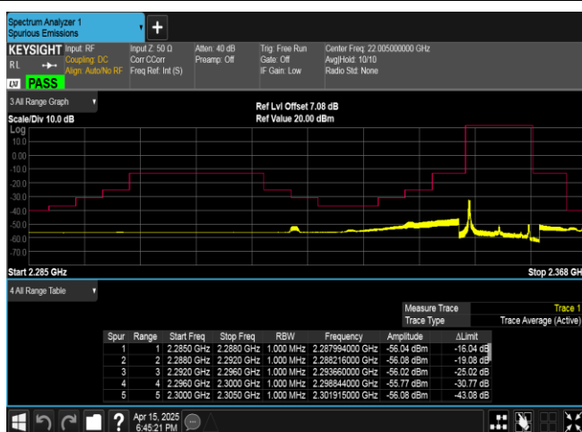
Band40(2350-2360)-10MHz-QPSK-39200-1RB#0-PASS
