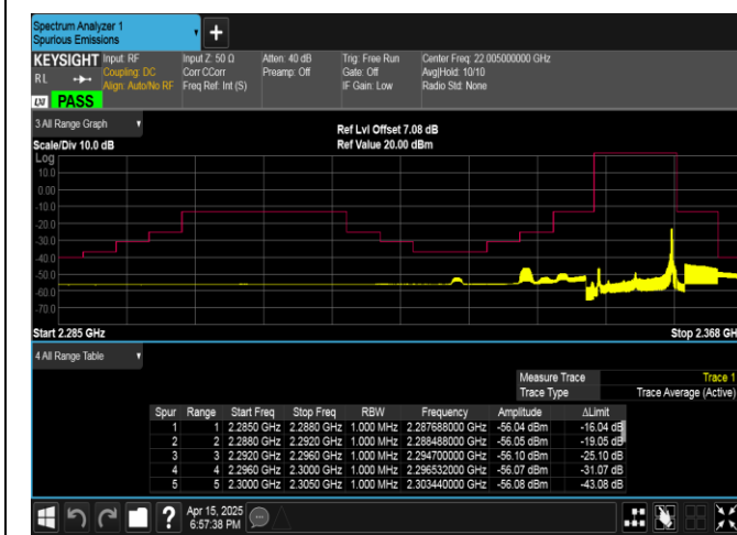
Band40(2350-2360)-10MHz-16QAM-39200-1RB#49-PASS
