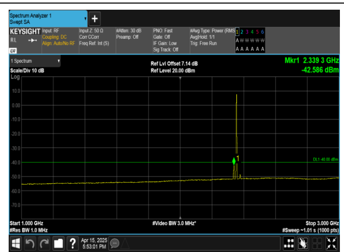
Band40(2350-2360)-5MHz-QPSK-39175-25RB#0-1000~3000-PASS
