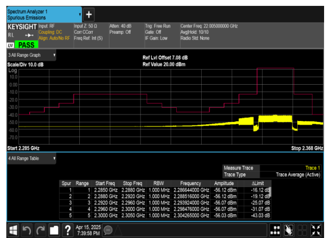
Band40(2350-2360)-10MHz-16QAM-39200-50RB#0-PASS
