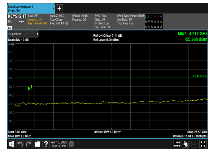
Band40(2350-2360)-5MHz-QPSK-39175-1RB#24-3000~26500-PASS
