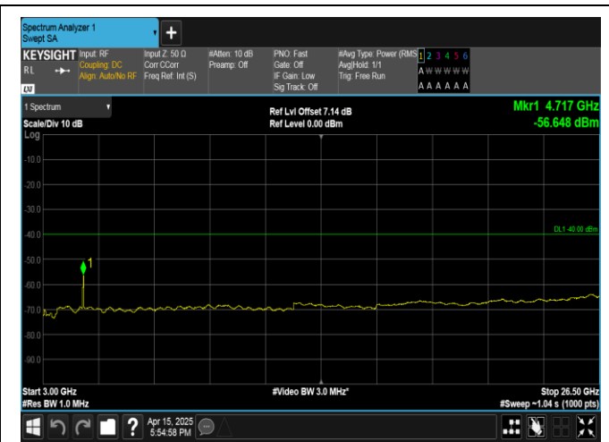
Band40(2350-2360)-5MHz-QPSK-39200-1RB#0-3000-26500-PASS
