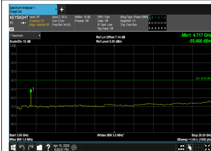
Band40(2350-2360)-5MHz-QPSK-39225-1RB#0-3000~26500-PASS
