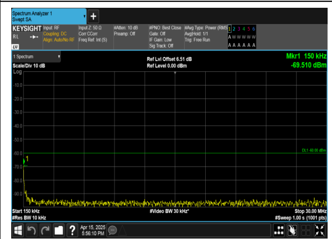
Band40(2350-2360)-5MHz-QPSK-39200-1RB#24-0.15-30-PASS
