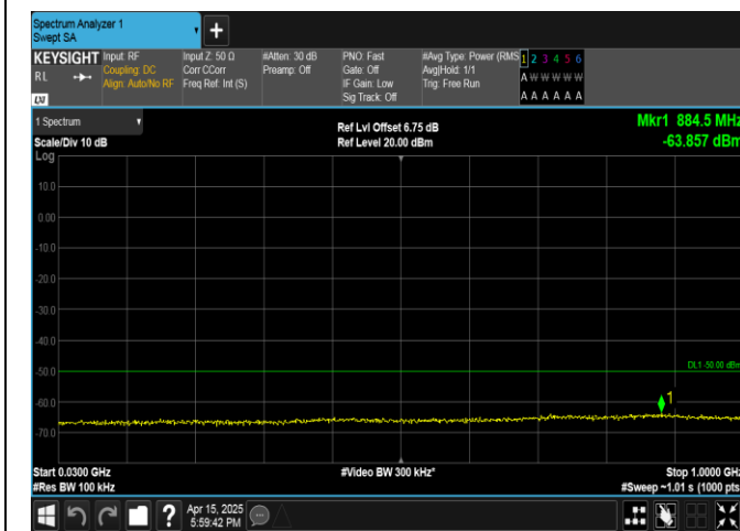
Band40(2350-2360)-5MHz-QPSK-39225-1RB#0-30~1000-PASS
