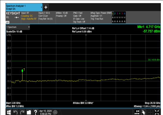
Band40(2350-2360)-5MHz-QPSK-39200-25RB#0-3000-26500-PASS
