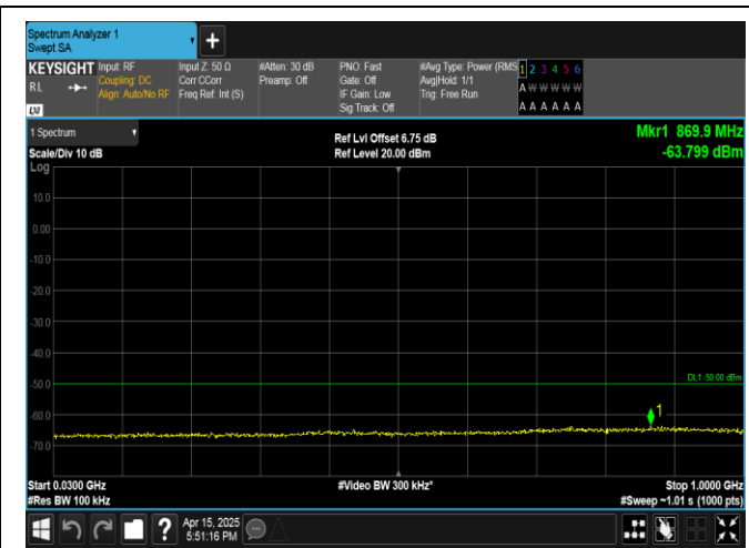
Band40(2350-2360)-5MHz-QPSK-39175-1RB#24-30~1000-PASS
