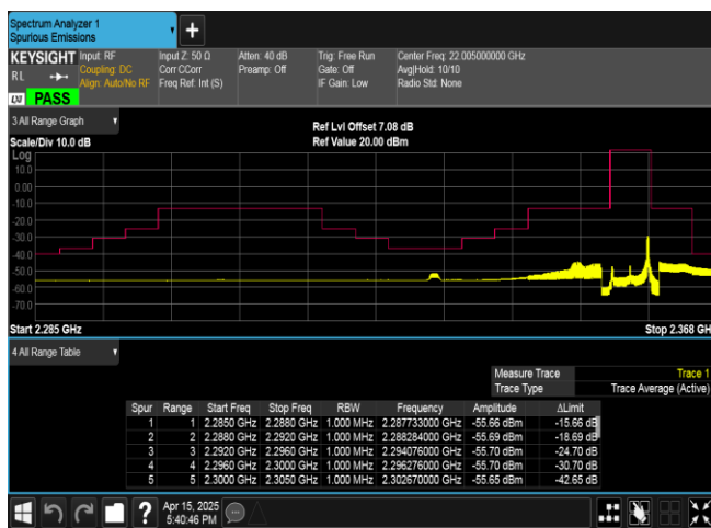
Band40(2350-2360)-5MHz-16QAM-39225-1RB#24-PASS
