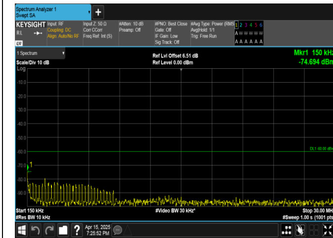
Band40(2305-2315)-10MHz-16QAM-38750-50RB#0-0.15~30-PASS
