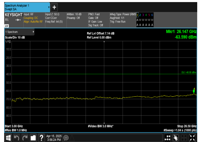
Band40(2305-2315)-5MHz-QPSK-38775-1RB#24-3000~26500-PASS
