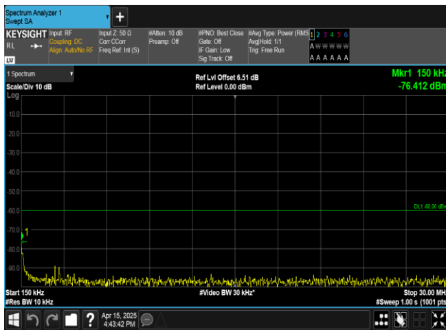
Band40(2305-2315)-10MHz-QPSK-38750-1RB#49-0.15~30-PASS
