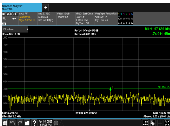
Band40(2305-2315)-5MHz-QPSK-38775-25RB#0-0.009~0.15-PASS
