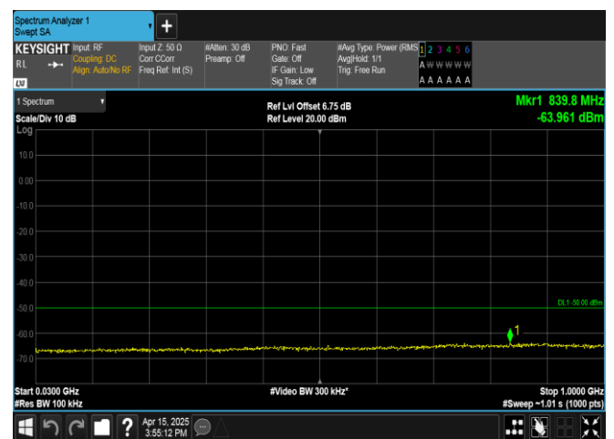
Band40(2305-2315)-5MHz-16QAM-38775-1RB#0-0-30~1000-PASS
