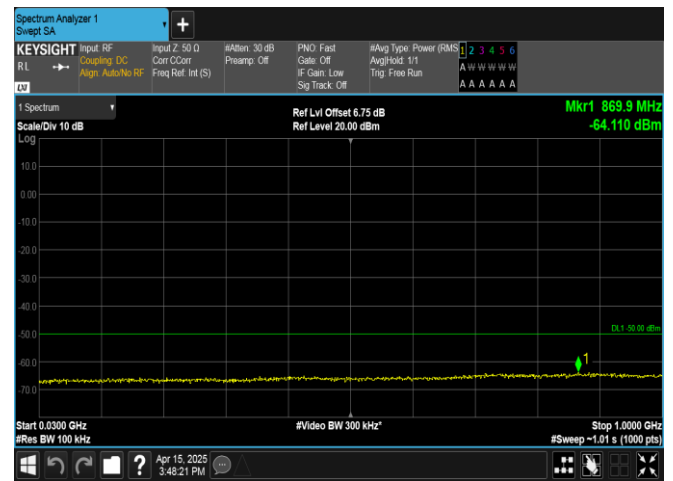
Band40(2305-2315)-5MHz-16QAM-38725-25RB#0-30-1000-PASS
