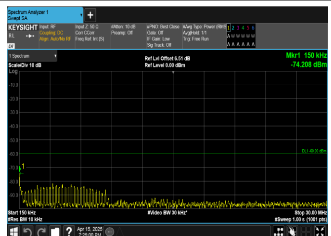
Band40(2305-2315)-10MHz-QPSK-38750-50RB#0-0.15~30-PASS
