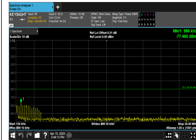
Band40(2305-2315)-5MHz-16QAM-38725-25RB#0-0.15-30-PASS
