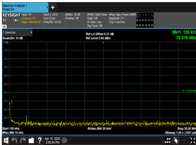
Band40(2305-2315)-5MHz-QPSK-38775-1RB#24-0.15~30-PASS
