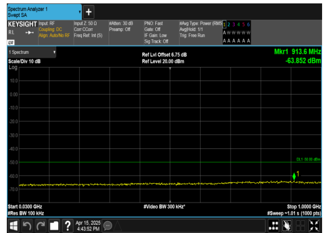
Band40(2305-2315)-10MHz-QPSK-38750-1RB#49-30~1000-PASS
