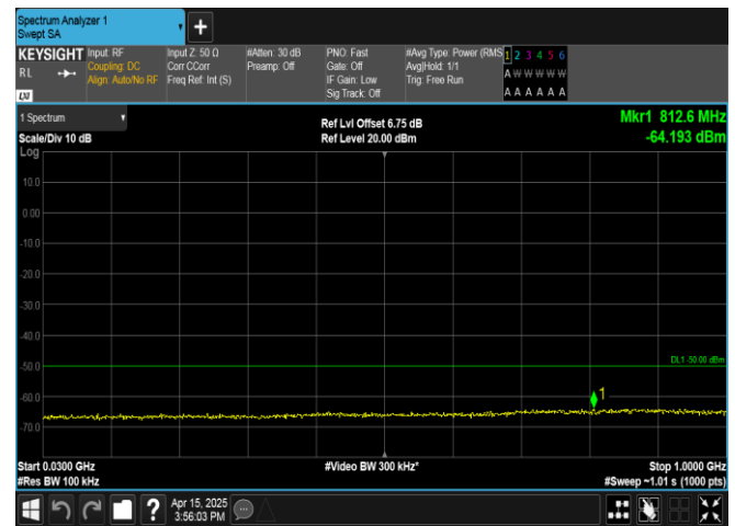
Band40(2305-2315)-5MHz-QPSK-38775-1RB#24-30~1000-PASS
