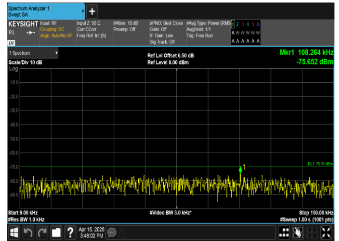
Band40(2305-2315)-5MHz-16QAM-38725-25RB#0-0.009-0.15-PASS
