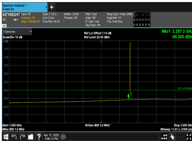
Band40(2305-2315)-5MHz-QPSK-38775-1RB#24-1000~3000-PASS
