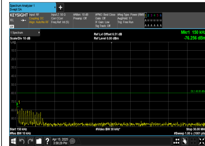
Band40(2305-2315)-5MHz-16QAM-38775-25RB#0-0.15-30-PASS
