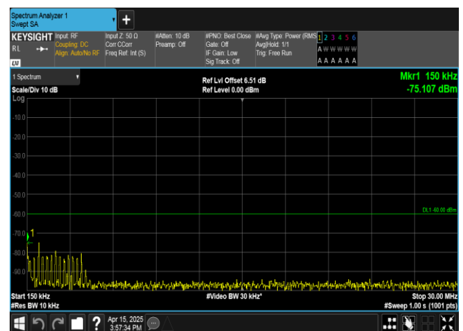
Band40(2305-2315)-5MHz-QPSK-38775-25RB#0-0.15~30-PASS
