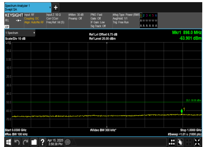
Band40(2305-2315)-5MHz-16QAM-38775-25RB#0-30-1000-PASS
