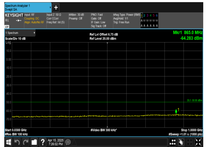
Band40(2305-2315)-10MHz-16QAM-38750-50RB#0-30~1000-PASS
