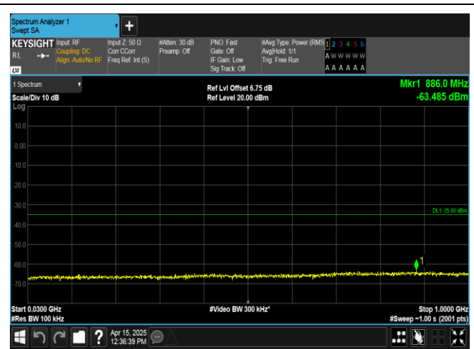
Band38-15MHz-16QAM-38175-75RB#0-30~1000-PASS
