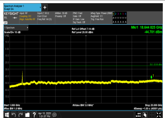
Band38-20MHz-QPSK-37850-100RB#0-1000~20000-PASS
