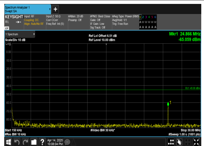
Band38-20MHz-16QAM-38000-1RB#0-0.15~30-PASS
