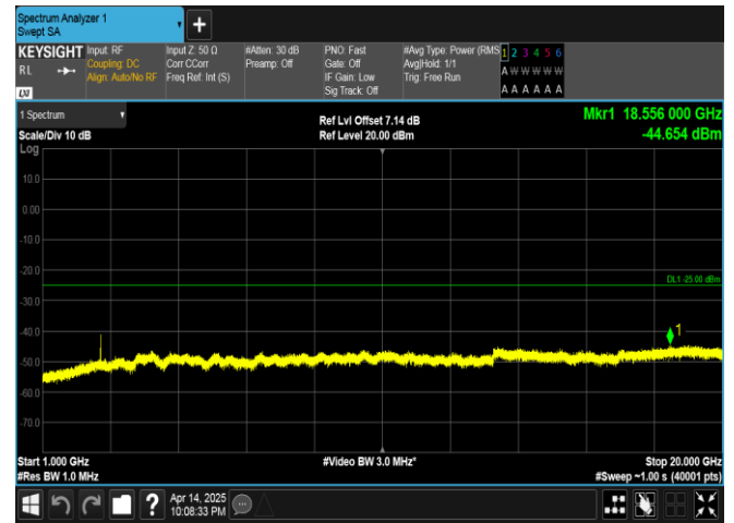
Band38-20MHz-16QAM-38000-1RB#0-1000~20000-PASS
