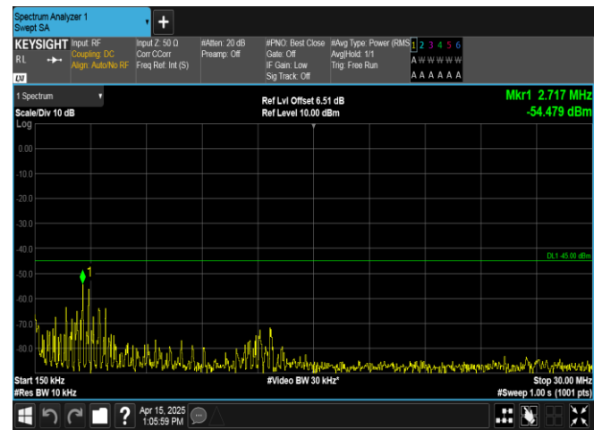
Band38-20MHz-QPSK-38150-100RB#0-0.15~30-PASS
