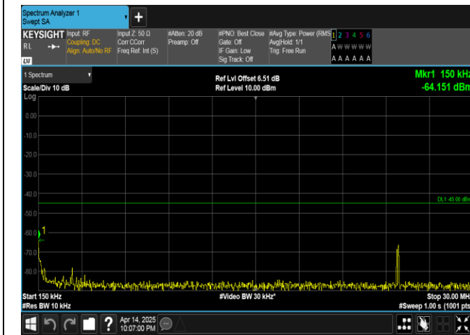
Band38-20MHz-QPSK-38000-1RB#0-0.15~30-PASS
