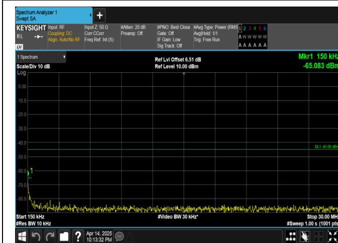
Band38-20MHz-QPSK-38150-1RB#99-0.15~30-PASS
