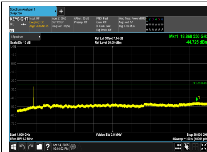
Band38-20MHz-QPSK-38150-1RB#99-1000~20000-PASS
