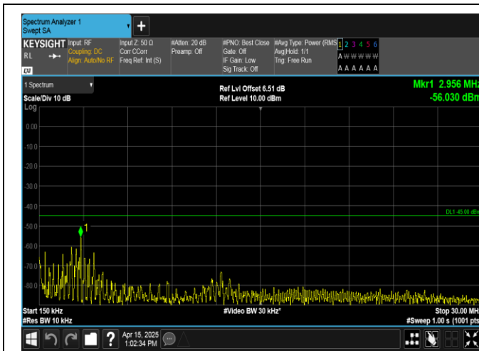
Band38-20MHz-16QAM-37850-100RB#0-0.15~30-PASS
