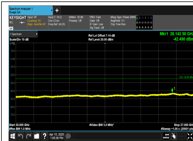
Band38-20MHz-16QAM-38000-100RB#0-20000~27000-PASS
