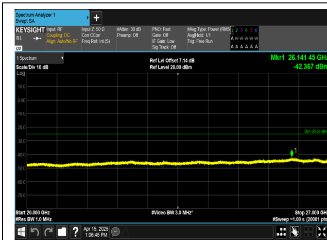
Band38-20MHz-QPSK-38150-100RB#0-20000~27000-PASS
