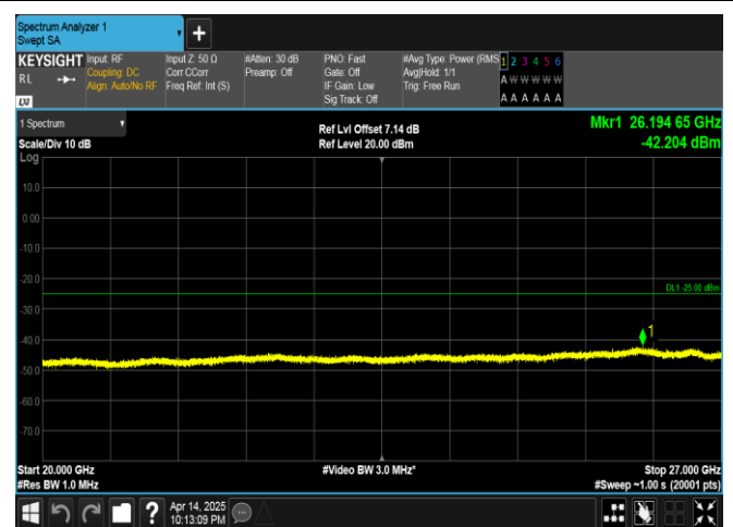
Band38-20MHz-16QAM-38150-1RB#0-20000~27000-PASS
