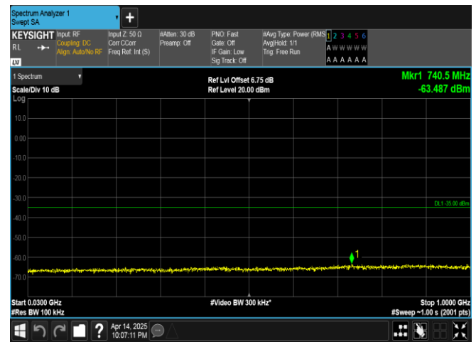
Band38-20MHz-QPSK-38000-1RB#0-30~1000-PASS
