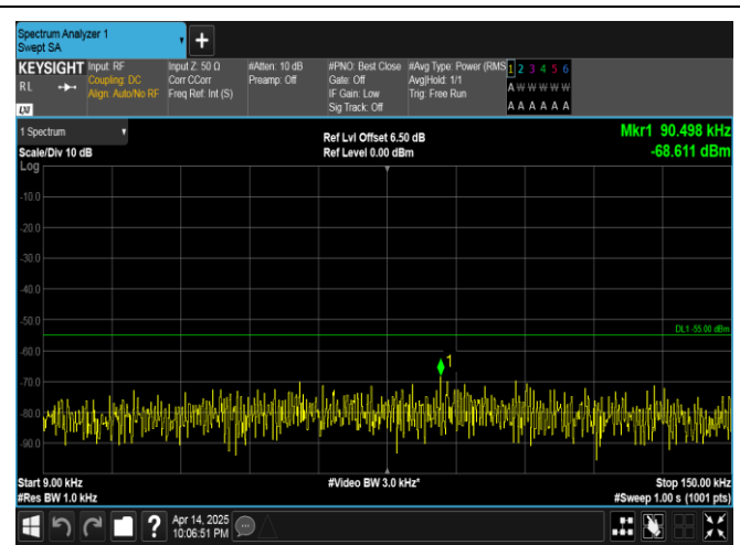
Band38-20MHz-QPSK-38000-1RB#0-0.009~0.15-PASS
