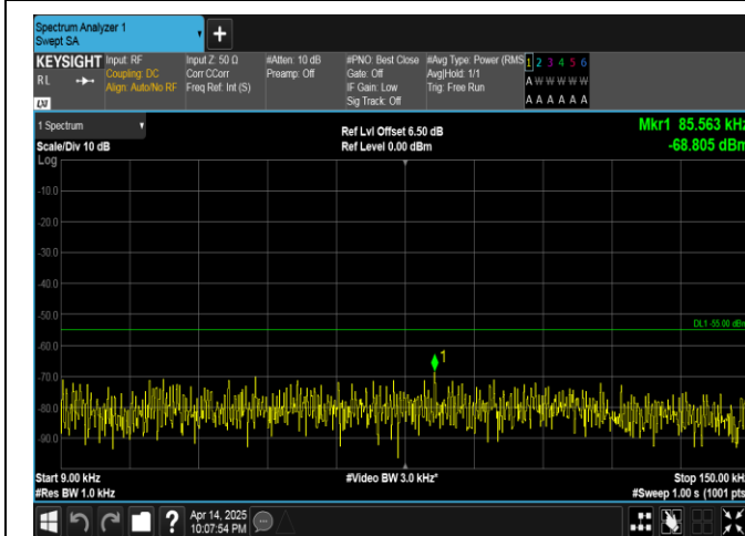
Band38-20MHz-16QAM-38000-1RB#0-0.009~0.15-PASS
