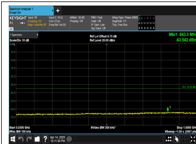
Band38-20MHz-QPSK-38150-1RB#0-30~1000-PASS
