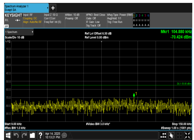
Band38-20MHz-QPSK-38150-1RB#99-0.009~0.15-PASS
