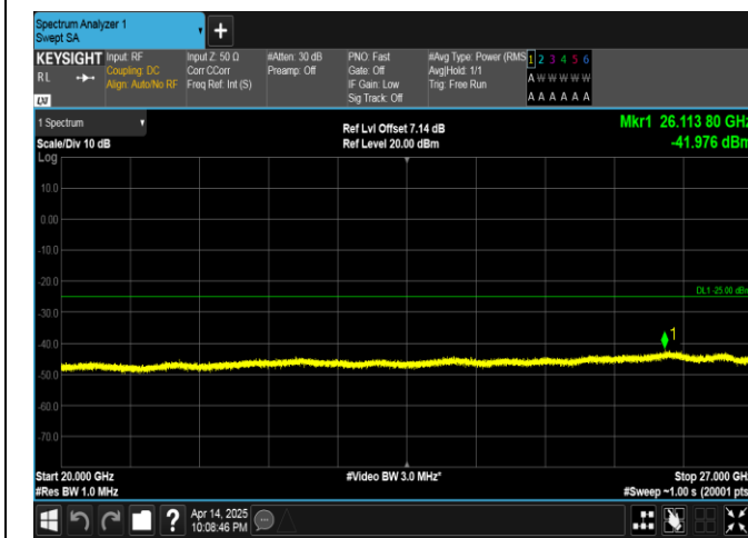
Band38-20MHz-16QAM-38000-1RB#0-20000~27000-PASS
