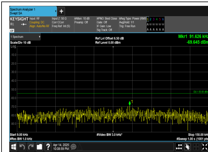
Band38-20MHz-QPSK-38000-1RB#99-0.009~0.15-PASS
