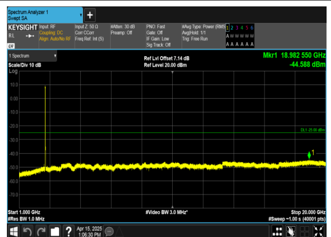
Band38-20MHz-QPSK-38150-100RB#0-1000~20000-PASS
