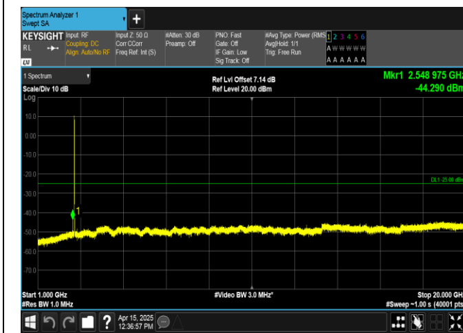
Band38-15MHz-16QAM-38175-75RB#0-1000~20000-PASS
