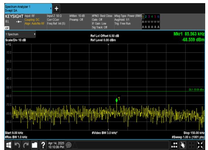
Band38-20MHz-16QAM-38000-1RB#99-0.009~0.15-PASS
