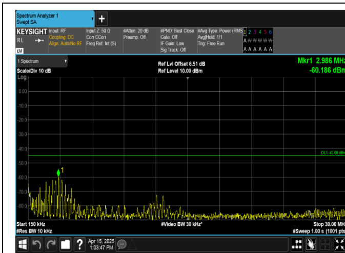
Band38-20MHz-QPSK-38000-100RB#0-0.15~30-PASS
