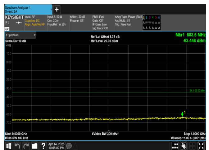
Band38-20MHz-QPSK-37850-1RB#99-30~1000-PASS
