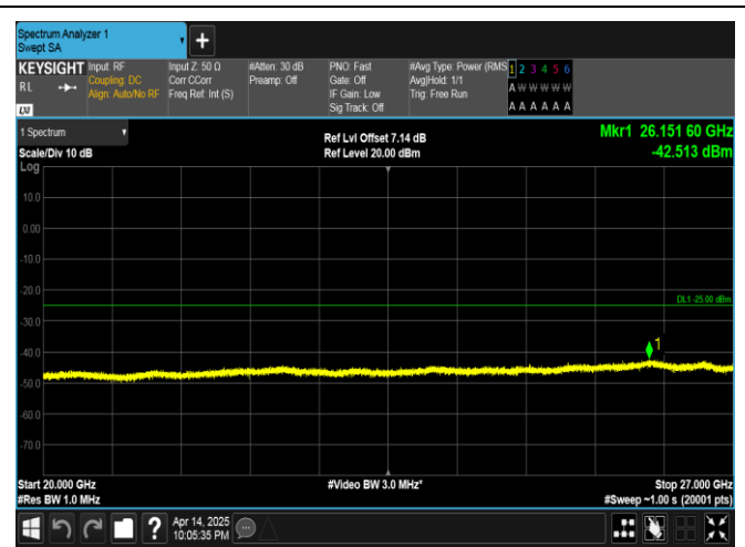
Band38-20MHz-QPSK-37850-1RB#99-20000~27000-PASS
