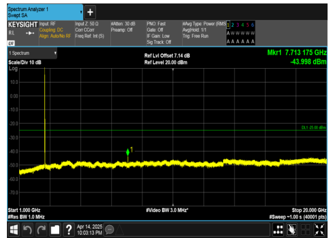
Band38-20MHz-QPSK-37850-1RB#0-1000~20000-PASS
