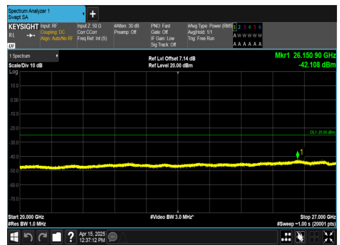
Band38-15MHz-16QAM-38175-75RB#0-20000~27000-PASS
