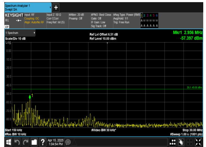
Band38-20MHz-16QAM-38000-100RB#0-0.15~30-PASS
