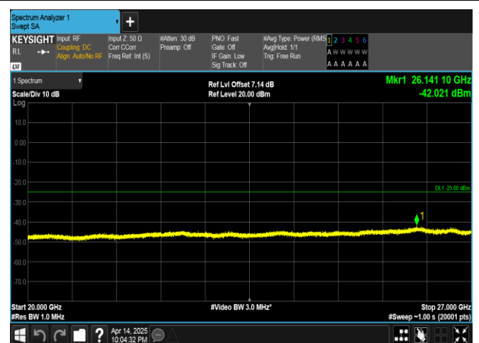
Band38-20MHz-16QAM-37850-1RB#0-20000~27000-PASS
