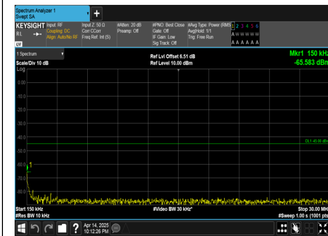
Band38-20MHz-16QAM-38150-1RB#0-0.15~30-PASS
