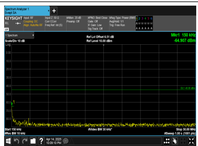
Band38-20MHz-QPSK-38000-1RB#99-0.15~30-PASS
