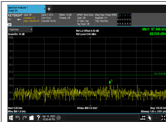
Band38-20MHz-16QAM-37850-1RB#99-0.009~0.15-PASS
