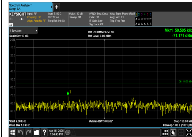
Band38-20MHz-16QAM-38000-100RB#0-0.009~0.15-PASS
