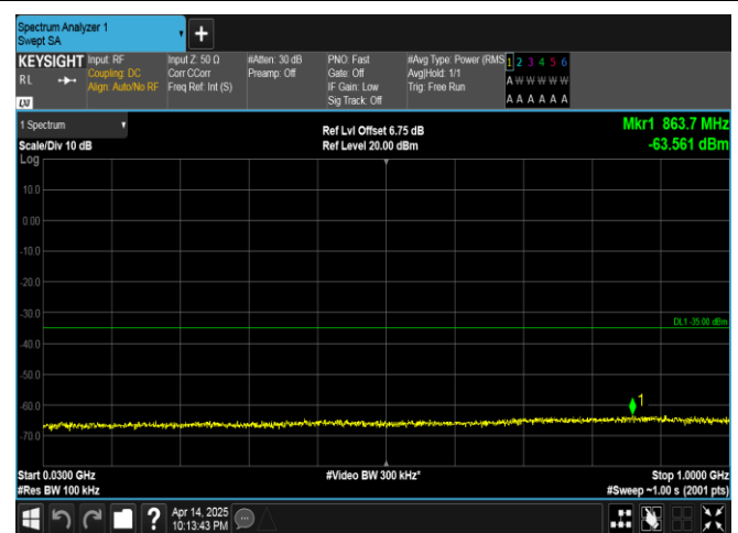
Band38-20MHz-QPSK-38150-1RB#99-30~1000-PASS
