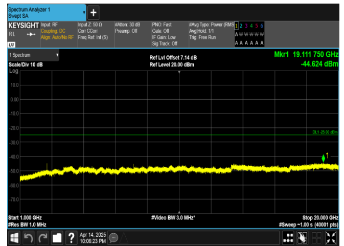
Band38-20MHz-16QAM-37850-1RB#99-1000~20000-PASS
