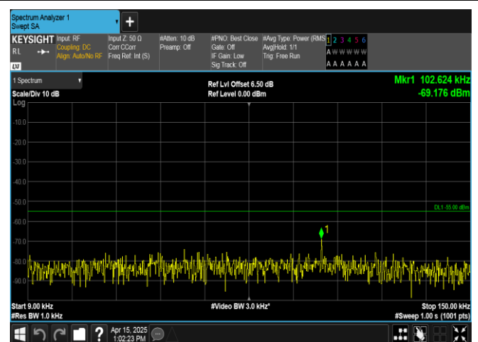
Band38-20MHz-16QAM-37850-100RB#0-0.009~0.15-PASS
