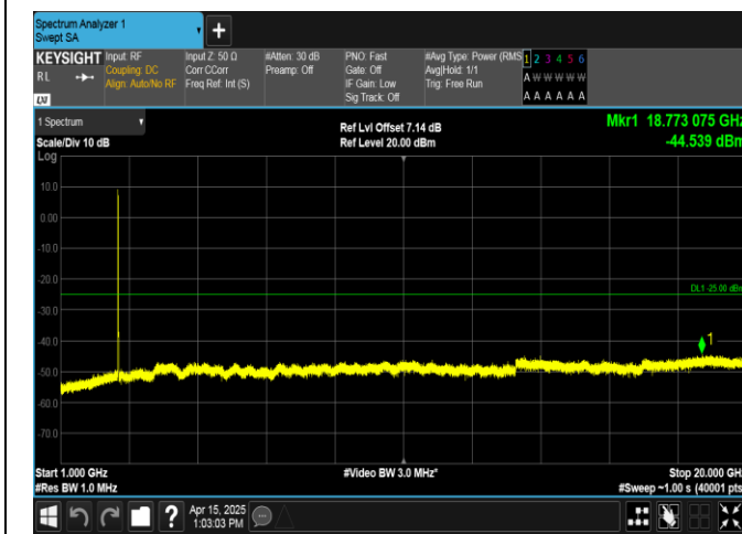
Band38-20MHz-16QAM-37850-100RB#0-1000~20000-PASS
