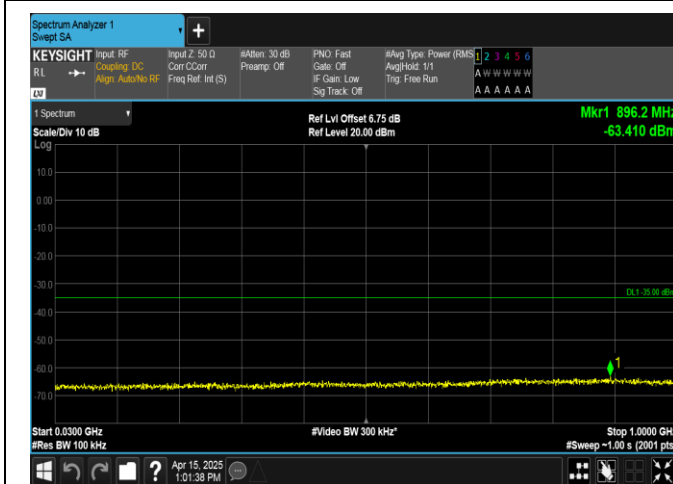
Band38-20MHz-QPSK-37850-100RB#0-30~1000-PASS
