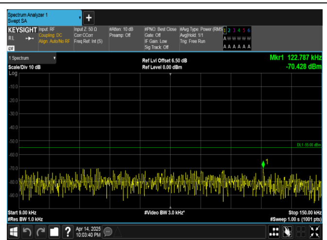
Band38-20MHz-16QAM-37850-1RB#0-0.009~0.15-PASS
