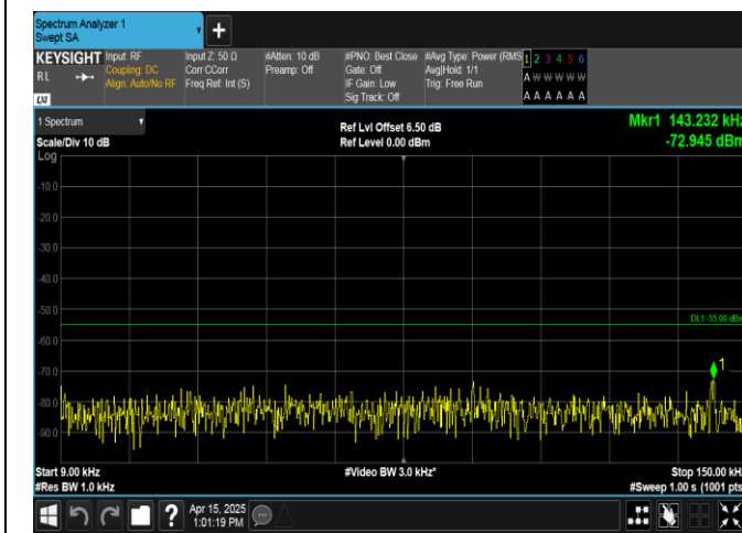
Band38-20MHz-QPSK-37850-100RB#0-0.009~0.15-PASS
