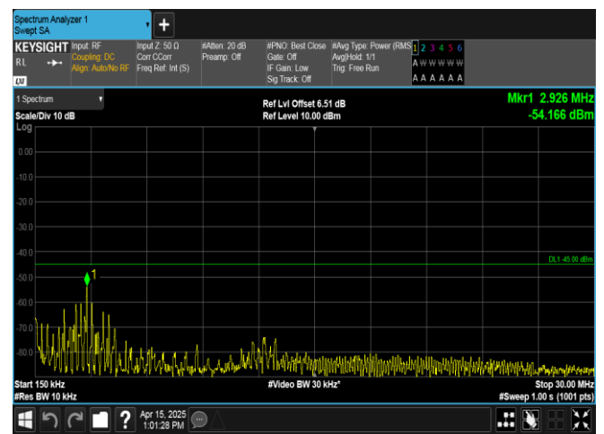
Band38-20MHz-QPSK-37850-100RB#0-0.15~30-PASS
