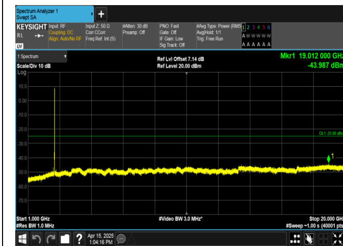
Band38-20MHz-QPSK-38000-100RB#0-1000~20000-PASS
