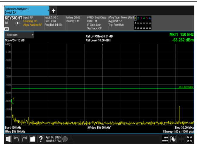
Band38-20MHz-16QAM-37850-1RB#99-0.15~30-PASS
