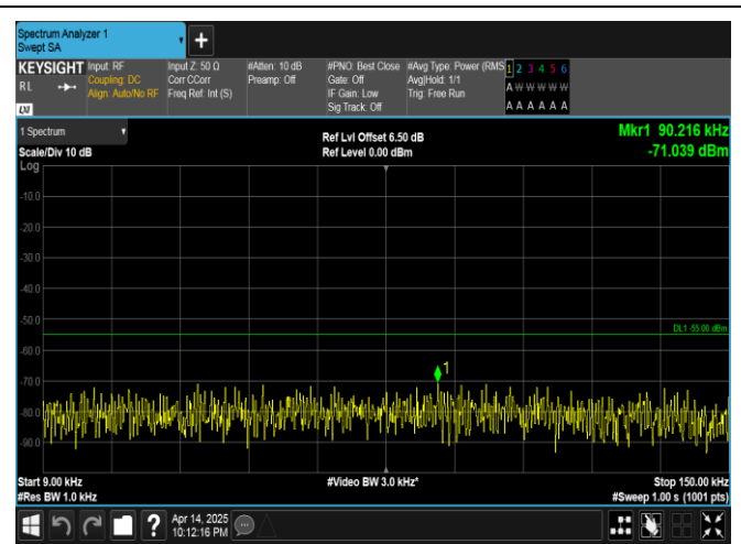
Band38-20MHz-16QAM-38150-1RB#0-0.009~0.15-PASS
