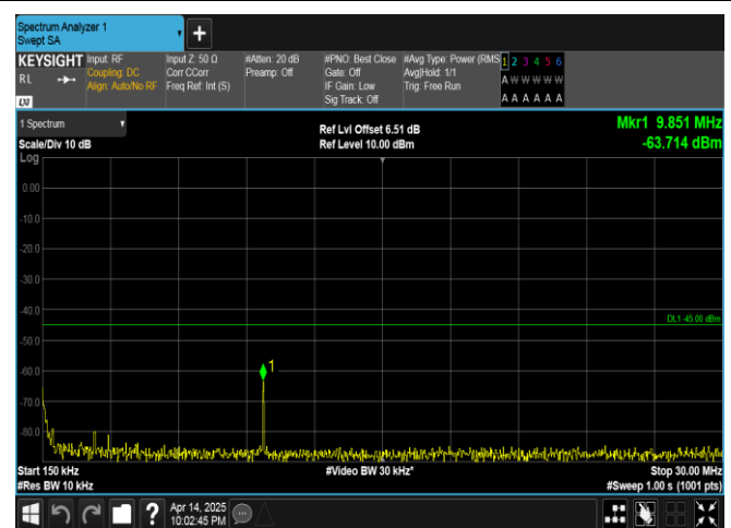
Band38-20MHz-QPSK-37850-1RB#0-0.15~30-PASS
