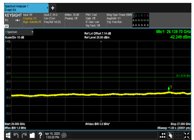
Band38-20MHz-16QAM-37850-100RB#0-20000~27000-PASS
