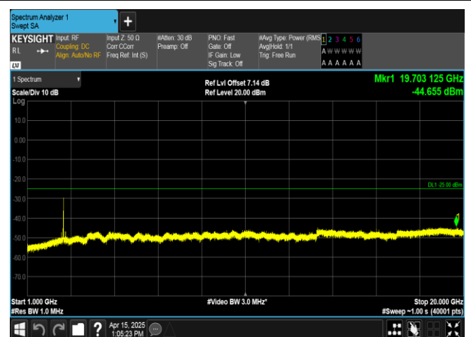
Band38-20MHz-16QAM-38000-100RB#0-1000~20000-PASS
