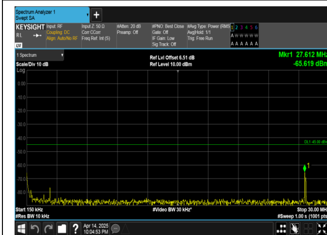
Band38-20MHz-QPSK-37850-1RB#99-0.15~30-PASS
