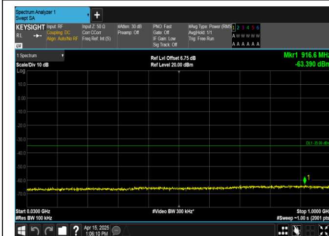
Band38-20MHz-QPSK-38150-100RB#0-30~1000-PASS
