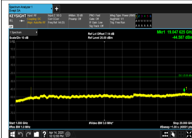
Band38-20MHz-16QAM-38150-1RB#0-1000~20000-PASS
