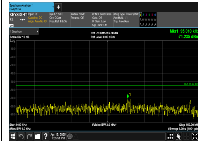
Band38-20MHz-QPSK-38150-100RB#0-0.009~0.15-PASS
