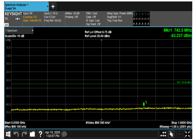
Band38-20MHz-QPSK-38000-100RB#0-30~1000-PASS
