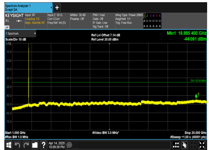
Band38-20MHz-QPSK-38000-1RB#99-1000~20000-PASS
