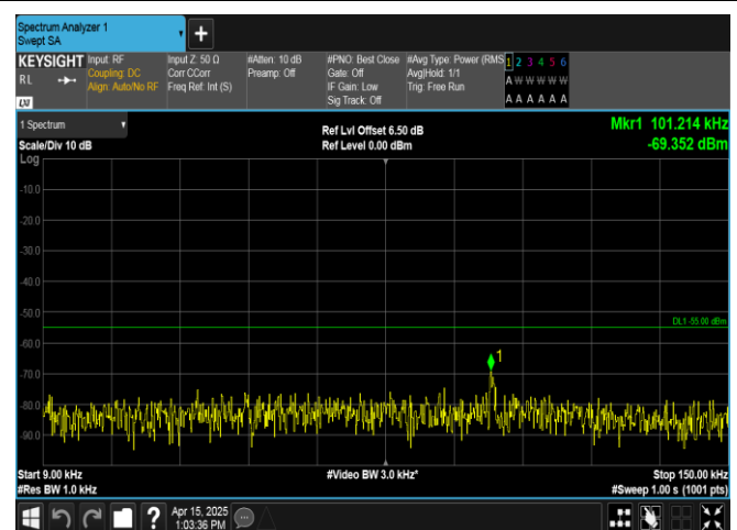
Band38-20MHz-QPSK-38000-100RB#0-0.009~0.15-PASS
