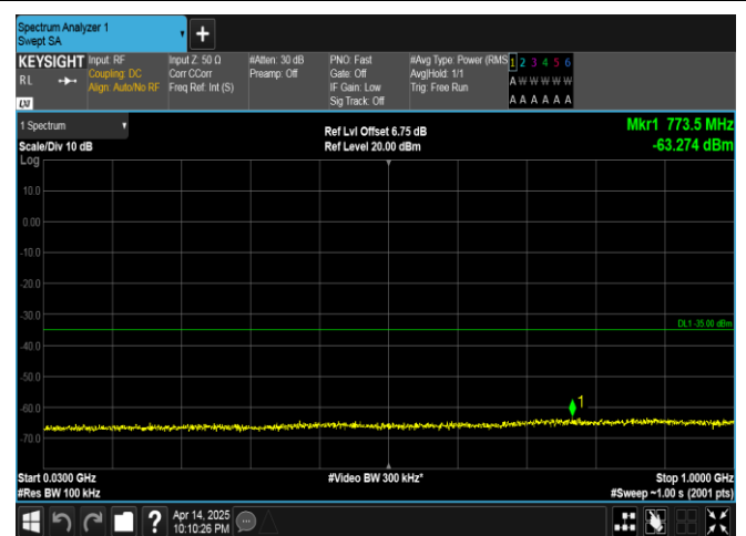
Band38-20MHz-16QAM-38000-1RB#99-30~1000-PASS
