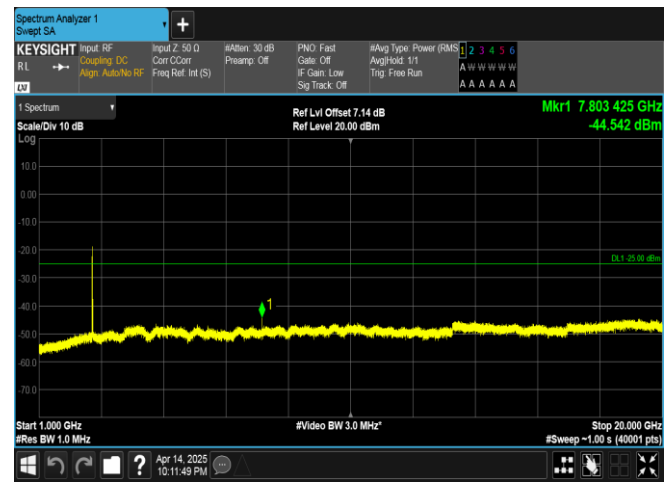
Band38-20MHz-QPSK-38150-1RB#0-1000~20000-PASS
