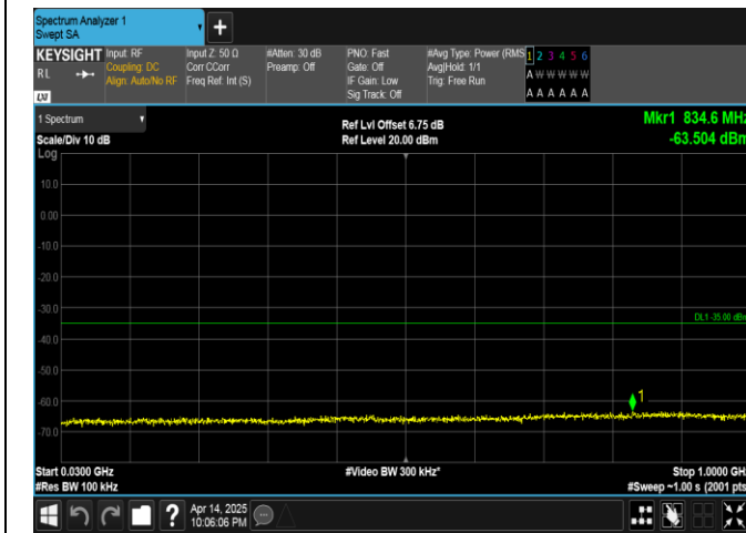
Band38-20MHz-16QAM-37850-1RB#99-30~1000-PASS
