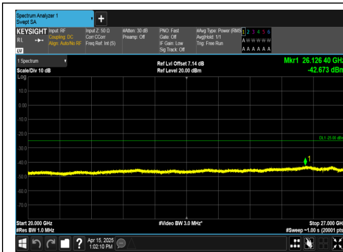
Band38-20MHz-QPSK-37850-100RB#0-20000~27000-PASS
