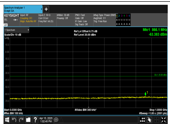
Band38-20MHz-16QAM-37850-100RB#0-30~1000-PASS
