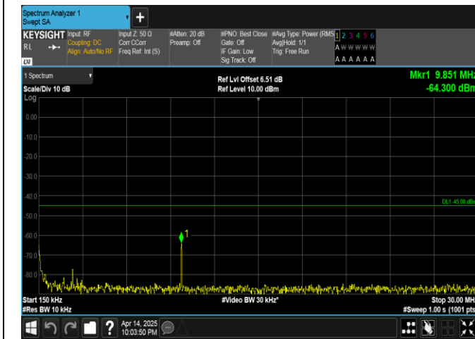
Band38-20MHz-16QAM-37850-1RB#0-0.15~30-PASS
