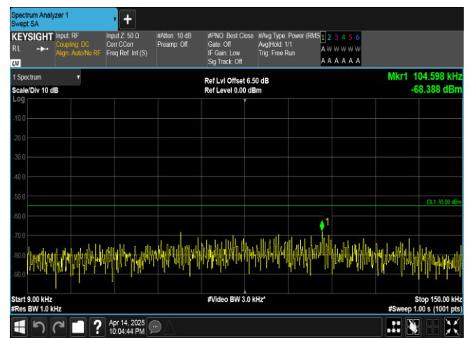
Band38-20MHz-QPSK-37850-1RB#99-0.009~0.15-PASS
