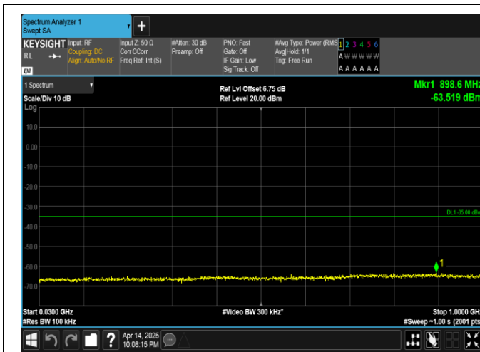
Band38-20MHz-16QAM-38000-1RB#0-30~1000-PASS
