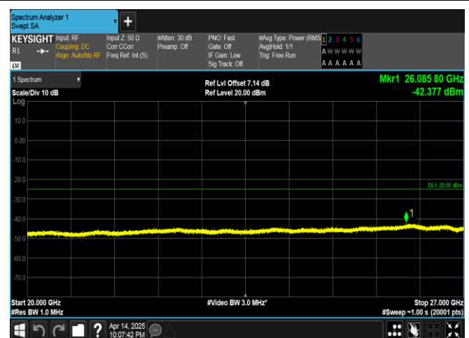
Band38-20MHz-QPSK-38000-1RB#0-20000~27000-PASS
