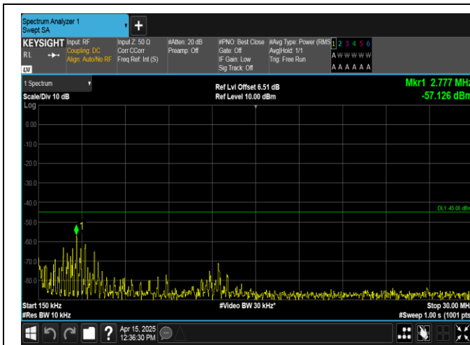
Band38-15MHz-16QAM-38175-75RB#0-0.15~30-PASS
