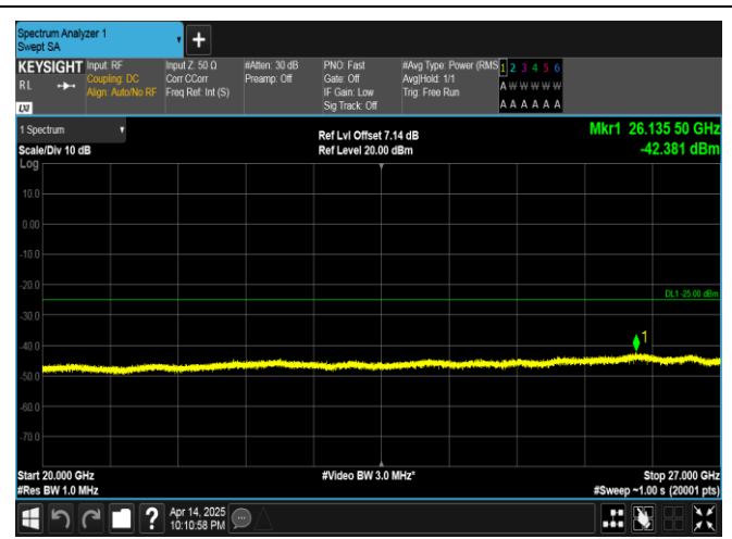
Band38-20MHz-16QAM-38000-1RB#99-20000~27000-PASS
