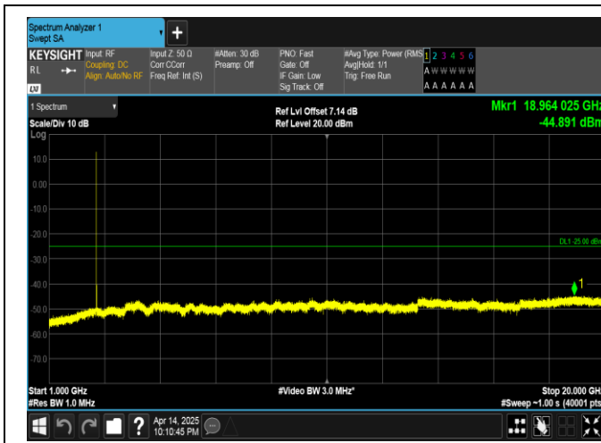
Band38-20MHz-16QAM-38000-1RB#99-1000~20000-PASS
