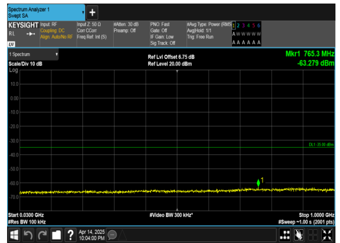
Band38-20MHz-16QAM-37850-1RB#0-30~1000-PASS
