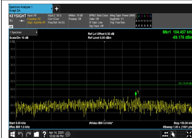
Band38-20MHz-QPSK-37850-1RB#0-0.009~0.15-PASS
