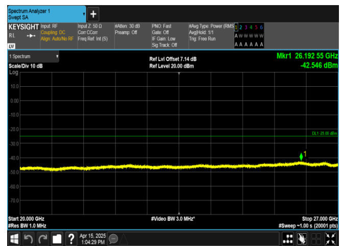
Band38-20MHz-QPSK-38000-100RB#0-20000~27000-PASS
