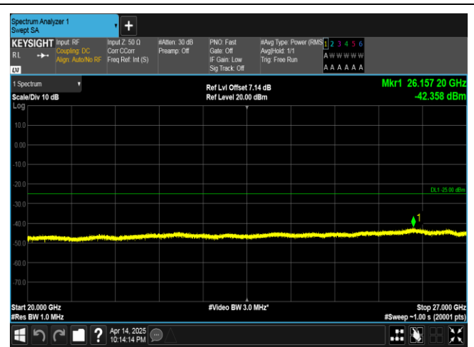
Band38-20MHz-QPSK-38150-1RB#99-20000~27000-PASS
