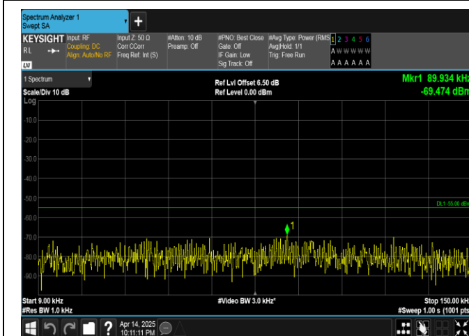
Band38-20MHz-QPSK-38150-1RB#0-0.009~0.15-PASS
