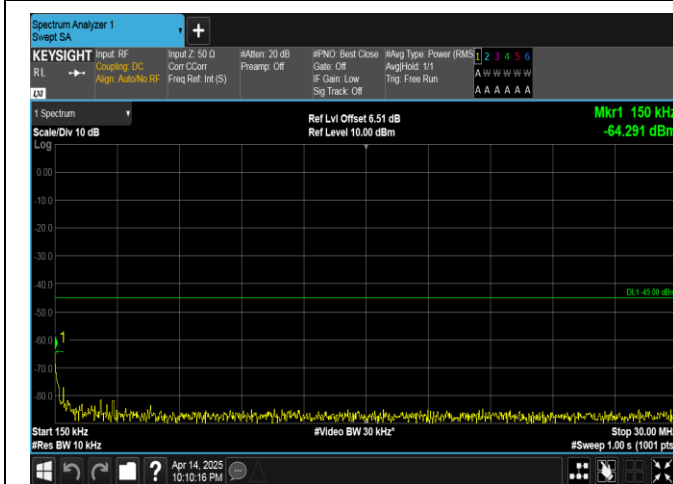
Band38-20MHz-16QAM-38000-1RB#99-0.15~30-PASS
