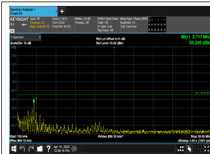
Band38-10MHz-QPSK-38000-50RB#0-0.15~30-PASS
