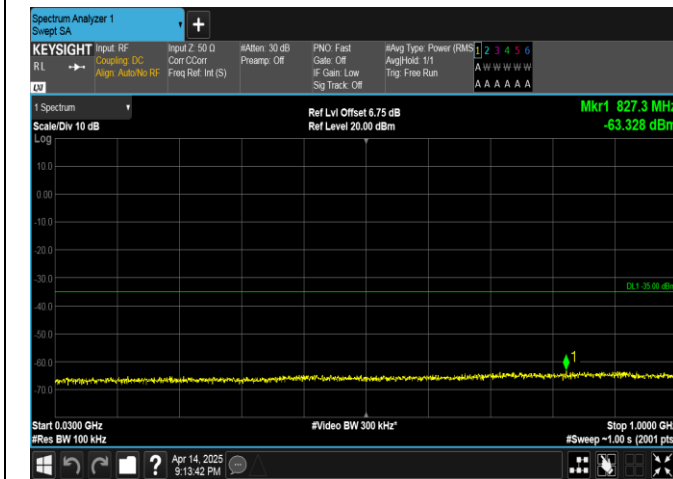
Band38-10MHz-16QAM-37800-1RB#49-30~1000-PASS
