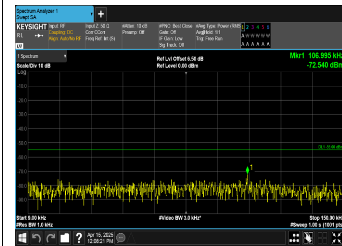
Band38-10MHz-QPSK-38200-50RB#0-0.009~0.15-PASS
