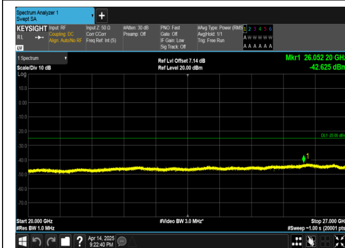
Band38-10MHz-16QAM-38200-1RB#49-20000~27000-PASS
