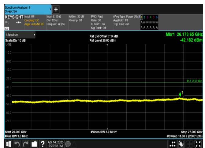
Band38-10MHz-16QAM-38200-1RB#0-20000~27000-PASS
