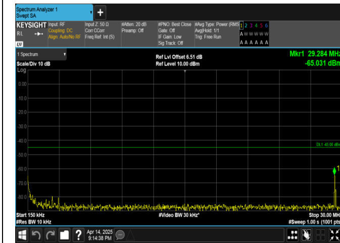
Band38-10MHz-QPSK-38000-1RB#0-0.15~30-PASS
