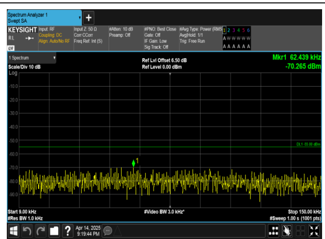
Band38-10MHz-16QAM-38200-1RB#0-0.009~0.15-PASS
