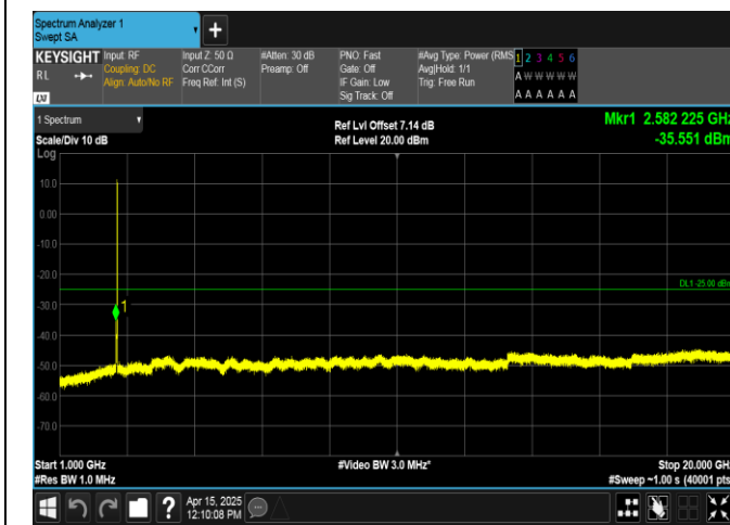
Band38-10MHz-16QAM-38200-50RB#0-1000~20000-PASS
