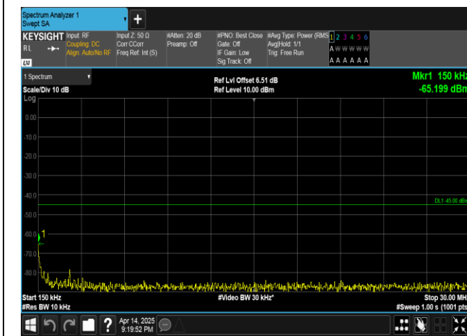
Band38-10MHz-16QAM-38200-1RB#0-0.15~30-PASS
