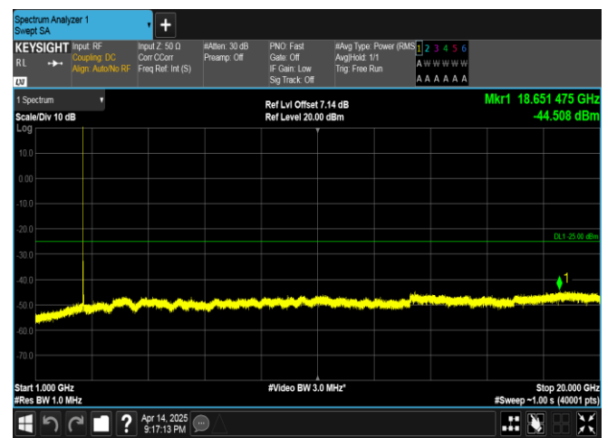
Band38-10MHz-QPSK-38000-1RB#49-1000~20000-PASS
