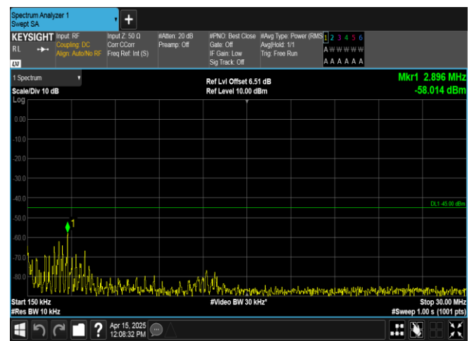
Band38-10MHz-QPSK-38200-50RB#0-0.15~30-PASS
