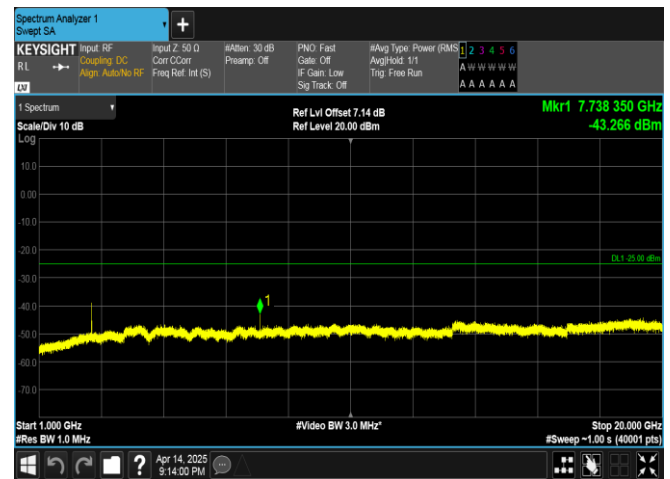
Band38-10MHz-16QAM-37800-1RB#49-1000~20000-PASS
