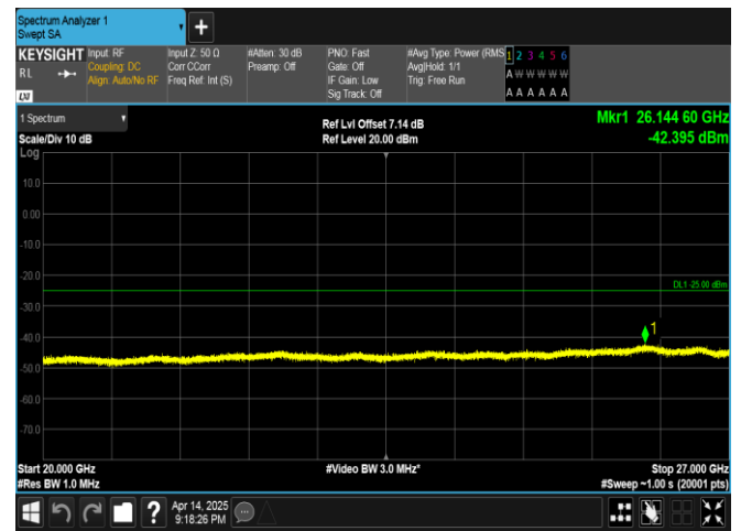
Band38-10MHz-16QAM-38000-1RB#49-20000~27000-PASS
