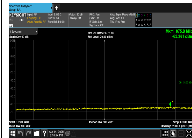
Band38-10MHz-QPSK-38000-1RB#49-30~1000-PASS
