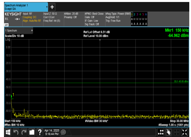
Band38-10MHz-QPSK-38000-1RB#49-0.15~30-PASS
