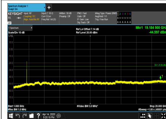
Band38-10MHz-16QAM-38200-1RB#0-1000~20000-PASS
