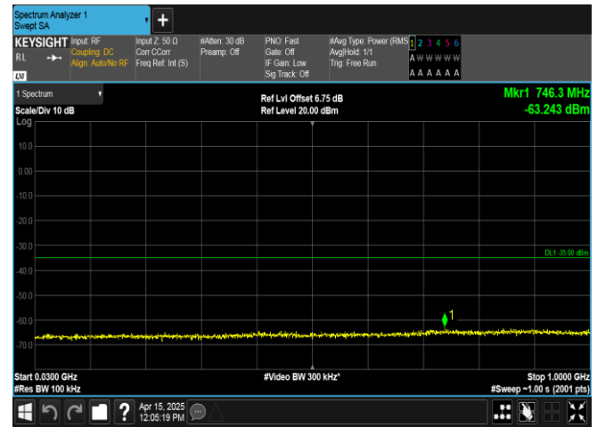
Band38-10MHz-16QAM-37800-50RB#0-30~1000-PASS
