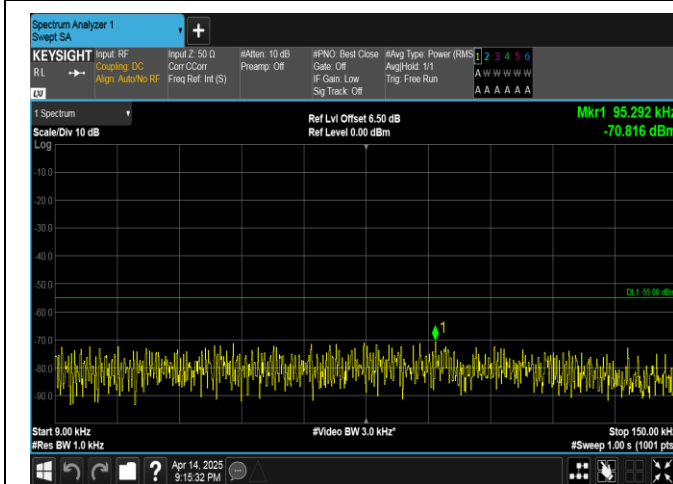
Band38-10MHz-16QAM-38000-1RB#0-0.009~0.15-PASS
