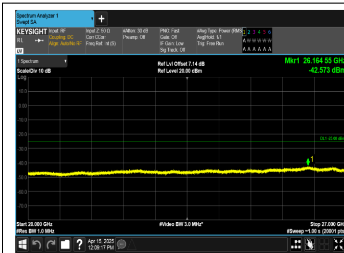
Band38-10MHz-QPSK-38200-50RB#0-20000~27000-PASS
