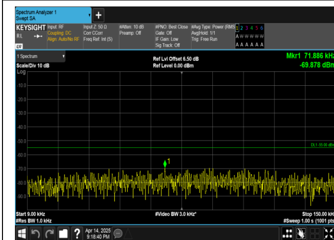
Band38-10MHz-QPSK-38200-1RB#0-0.009~0.15-PASS
