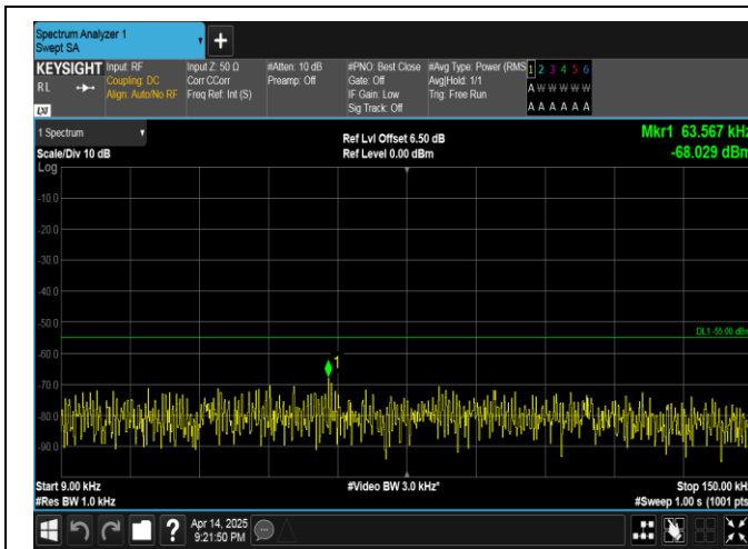
Band38-10MHz-16QAM-38200-1RB#49-0.009~0.15-PASS
