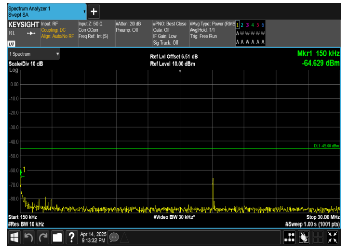
Band38-10MHz-16QAM-37800-1RB#49-0.15~30-PASS
