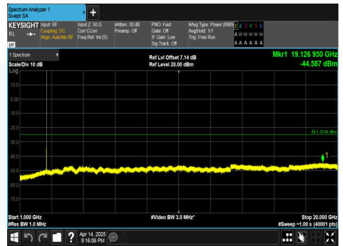
Band38-10MHz-16QAM-38000-1RB#0-1000~20000-PASS
