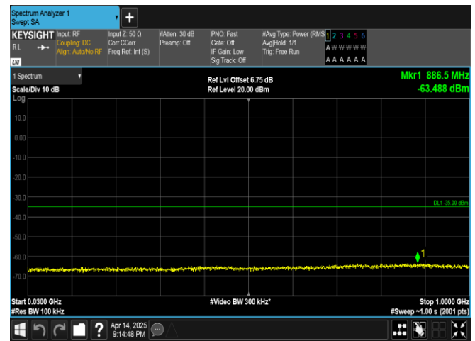
Band38-10MHz-QPSK-38000-1RB#0-30~1000-PASS
