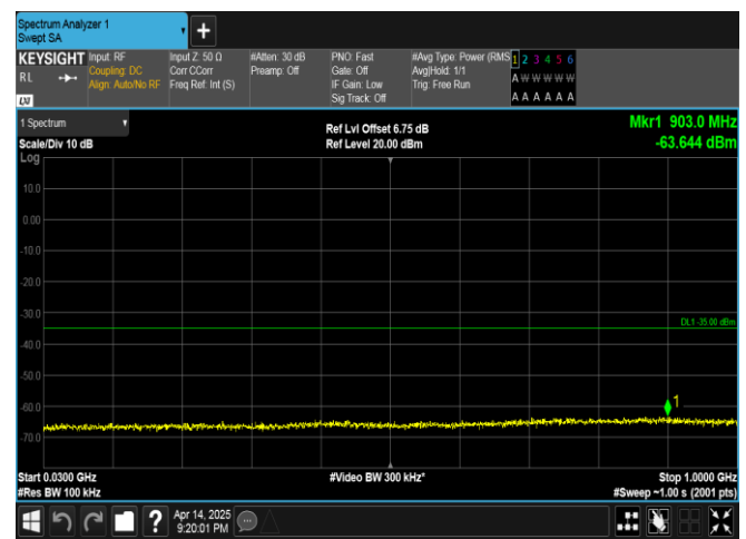
Band38-10MHz-16QAM-38200-1RB#0-30~1000-PASS
