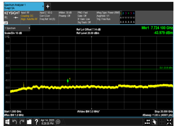
Band38-5MHz-16QAM-37775-1RB#24-1000~20000-PASS
