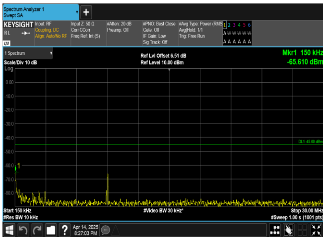
Band38-5MHz-16QAM-37775-1RB#0-0.15~30-PASS
