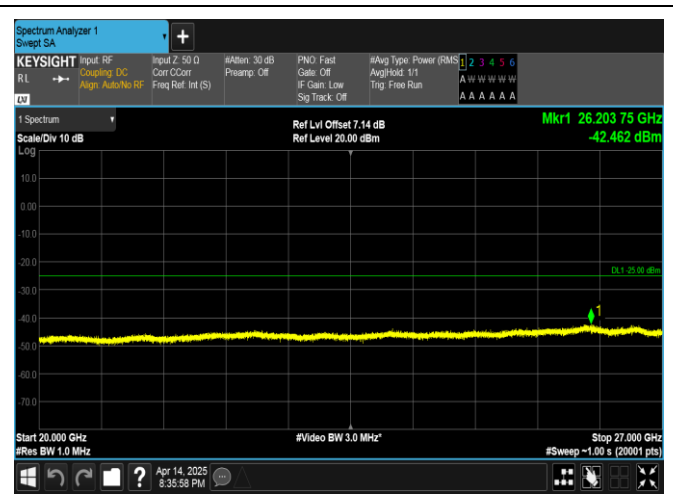
Band38-5MHz-16QAM-38000-1RB#24-20000~27000-PASS
