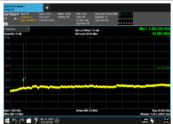
Band38-5MHz-16QAM-38000-25RB#0-1000~20000-PASS
