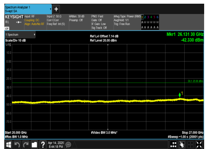
Band38-5MHz-16QAM-38225-25RB#0-20000~27000-PASS
