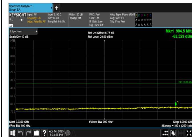
Band38-5MHz-QPSK-38000-1RB#24-30~1000-PASS
