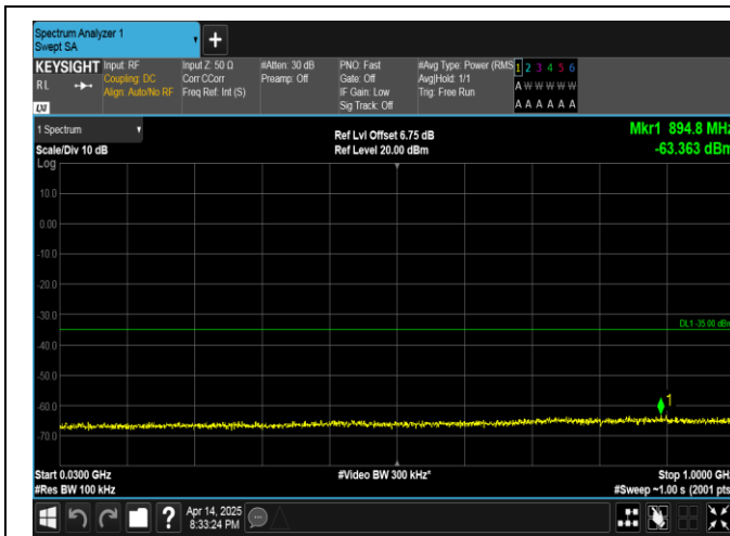
Band38-5MHz-16QAM-38000-1RB#0-30~1000-PASS
