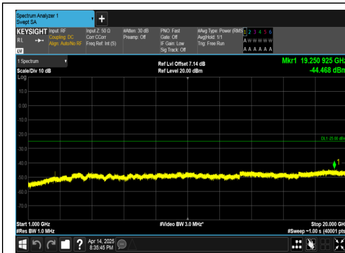
Band38-5MHz-16QAM-38000-1RB#24-1000~20000-PASS
