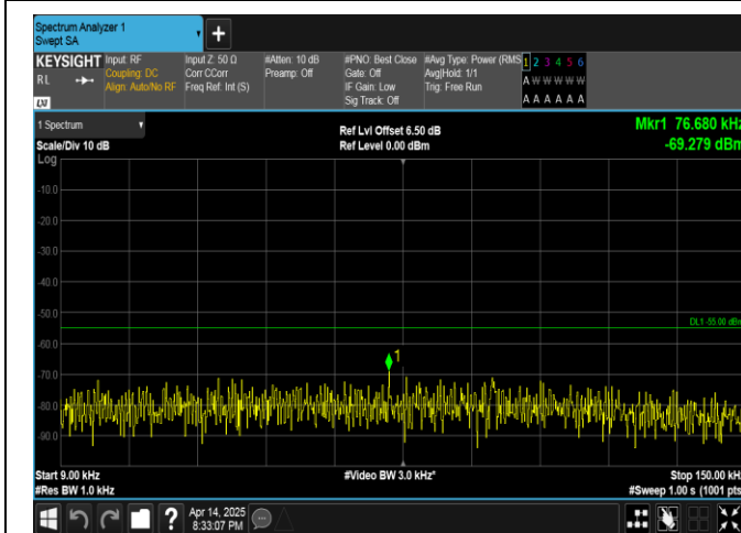
Band38-5MHz-16QAM-38000-1RB#0-0.009~0.15-PASS
