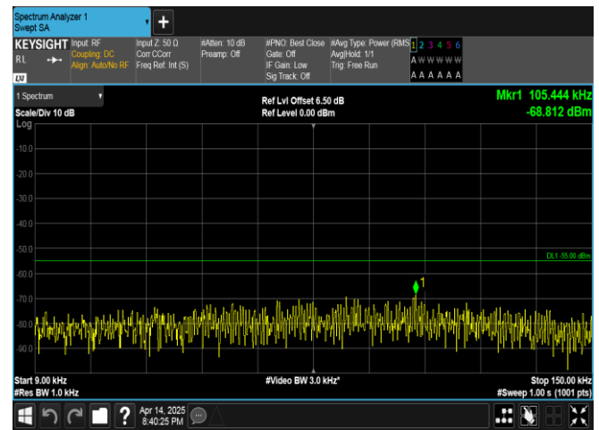
Band38-5MHz-QPSK-38225-1RB#24-0.009~0.15-PASS
