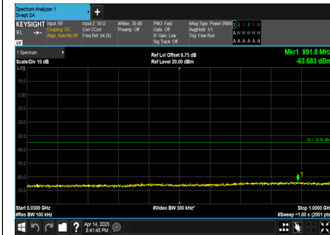
Band38-5MHz-16QAM-38225-1RB#24-30~1000-PASS
