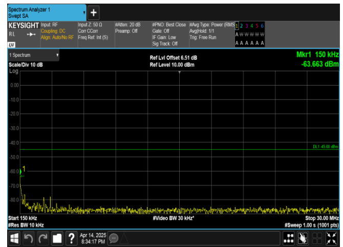
Band38-5MHz-QPSK-38000-1RB#24-0.15~30-PASS
