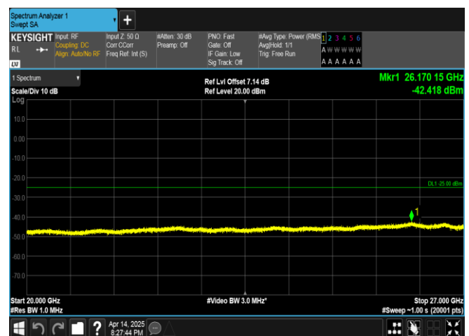
Band38-5MHz-16QAM-37775-1RB#0-20000~27000-PASS
