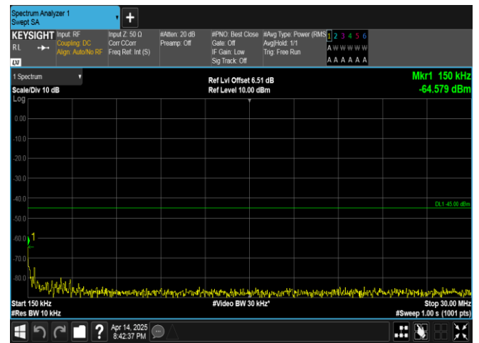
Band38-5MHz-QPSK-38225-25RB#0-0.15~30-PASS
