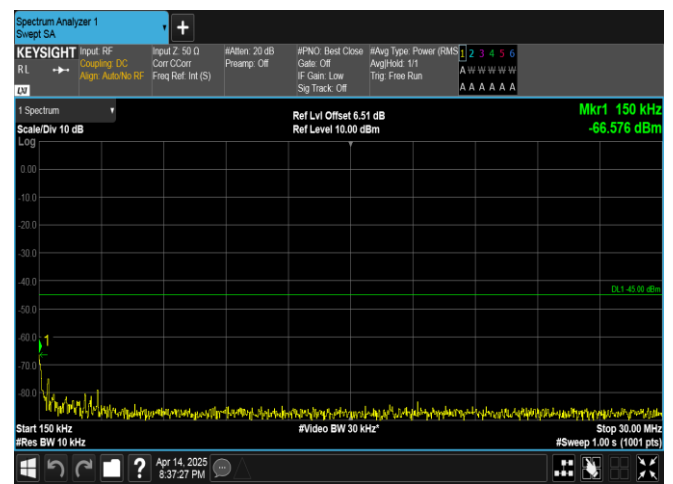
Band38-5MHz-16QAM-38000-25RB#0-0.15~30-PASS
