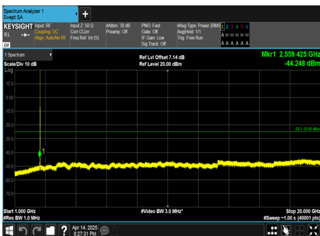
Band38-5MHz-16QAM-37775-1RB#0-1000~20000-PASS
