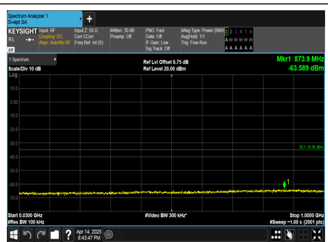
Band38-5MHz-16QAM-38225-25RB#0-30~1000-PASS
