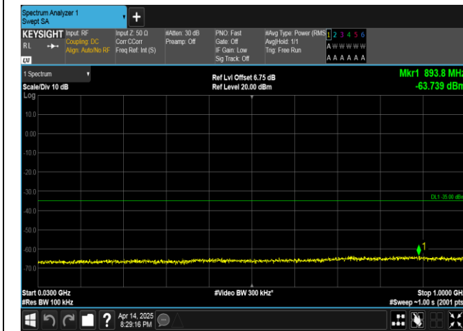
Band38-5MHz-16QAM-37775-1RB#24-30~1000-PASS
