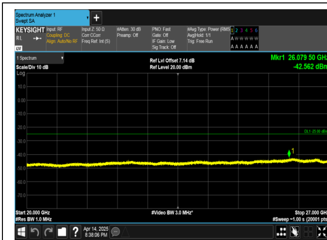
Band38-5MHz-16QAM-38000-25RB#0-20000~27000-PASS
