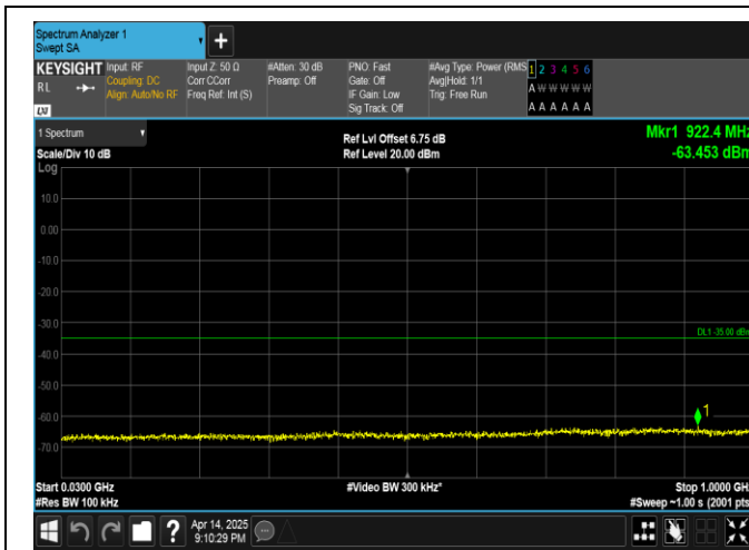
Band38-10MHz-QPSK-37800-1RB#0-30~1000-PASS
