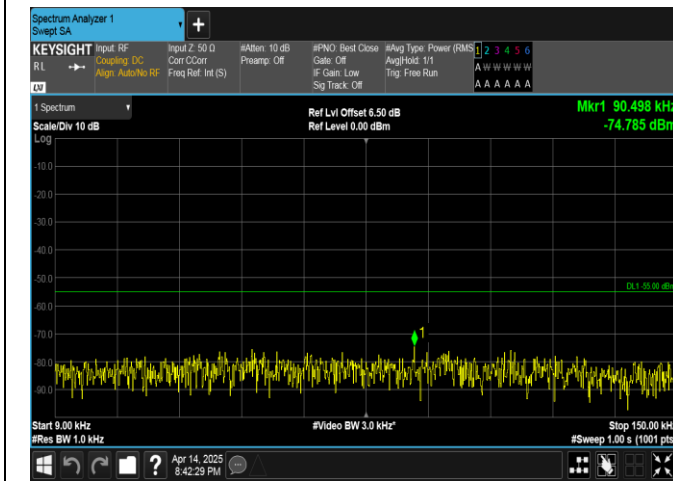
Band38-5MHz-QPSK-38225-25RB#0-0.009~0.15-PASS
