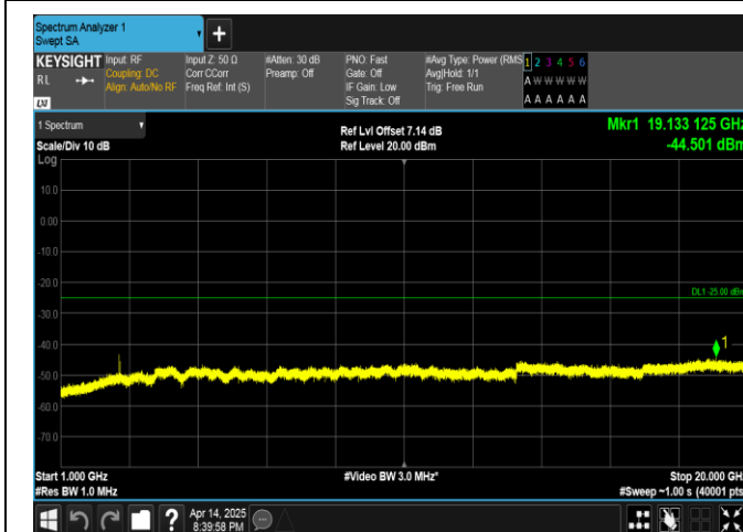
Band38-5MHz-16QAM-38225-1RB#0-1000~20000-PASS
