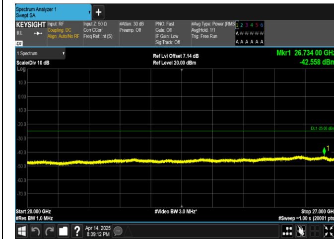
Band38-5MHz-QPSK-38225-1RB#0-20000~27000-PASS
