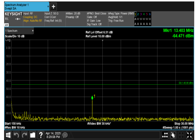
Band38-5MHz-16QAM-37775-1RB#24-0.15~30-PASS
