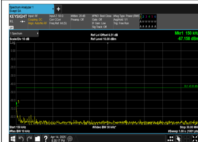
Band38-5MHz-16QAM-38000-1RB#24-0.15~30-PASS
