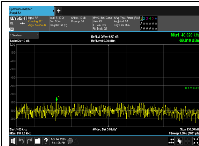
Band38-5MHz-16QAM-38225-1RB#24-0.009~0.15-PASS
