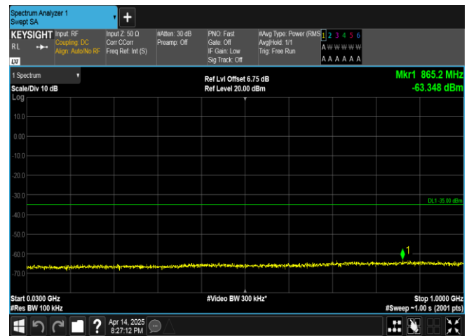
Band38-5MHz-16QAM-37775-1RB#0-30~1000-PASS
