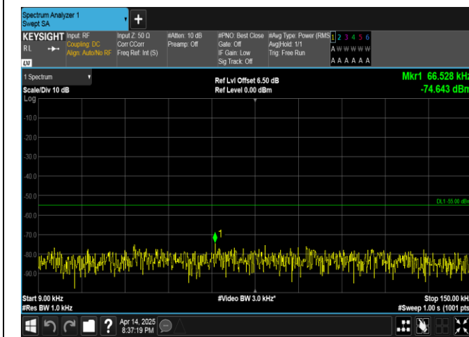
Band38-5MHz-16QAM-38000-25RB#0-0.009~0.15-PASS
