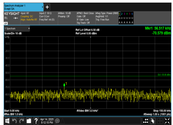
Band38-10MHz-QPSK-37800-1RB#49-0.009~0.15-PASS
