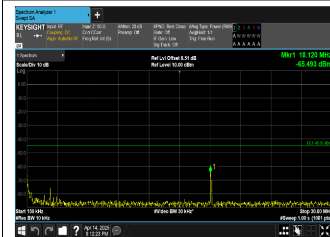
Band38-10MHz-QPSK-37800-1RB#49-0.15~30-PASS
