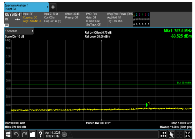
Band38-5MHz-16QAM-38225-1RB#0-30~1000-PASS
