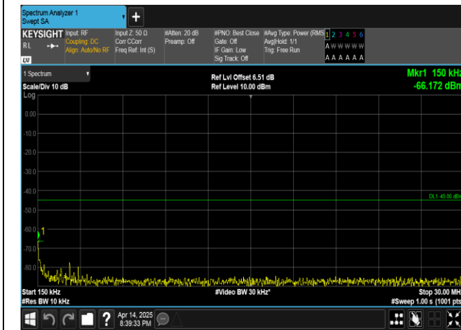
Band38-5MHz-16QAM-38225-1RB#0-0.15~30-PASS
