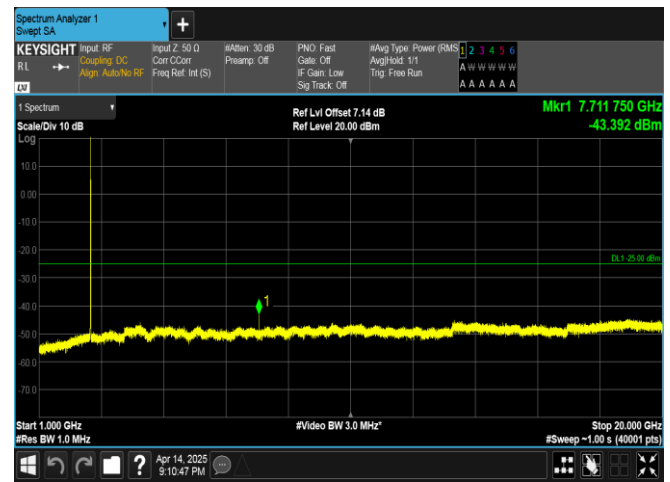
Band38-10MHz-QPSK-37800-1RB#0-1000~20000-PASS
