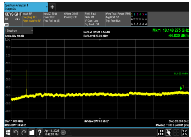
Band38-5MHz-16QAM-38225-1RB#24-1000~20000-PASS
