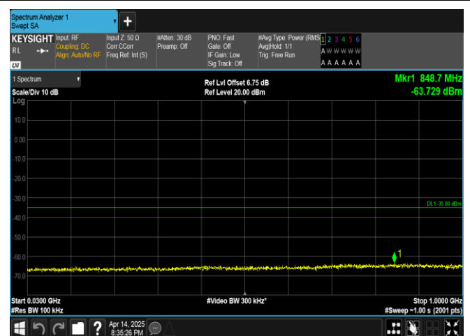
Band38-5MHz-16QAM-38000-1RB#24-30~1000-PASS
