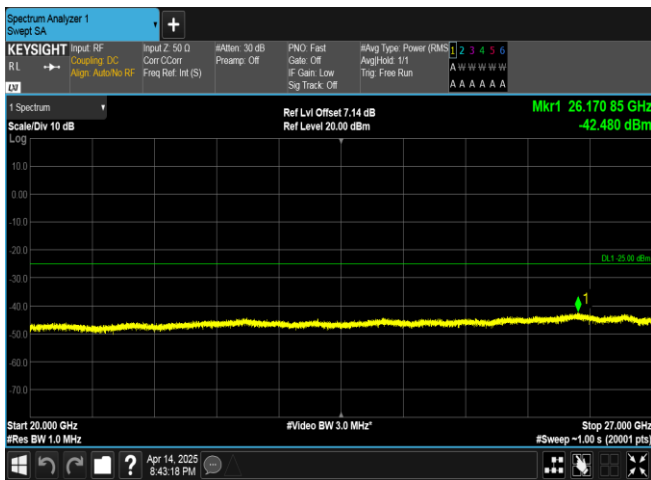
Band38-5MHz-QPSK-38225-25RB#0-20000~27000-PASS
