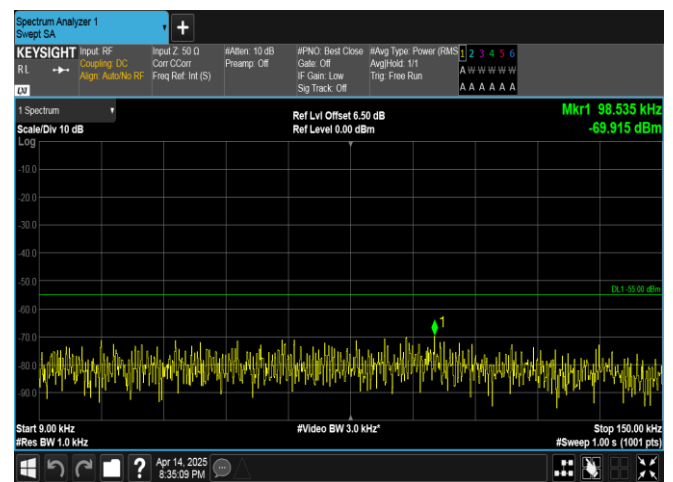
Band38-5MHz-16QAM-38000-1RB#24-0.009~0.15-PASS
