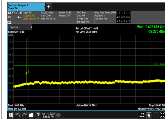
Band38-5MHz-QPSK-38000-25RB#0-1000~20000-PASS
