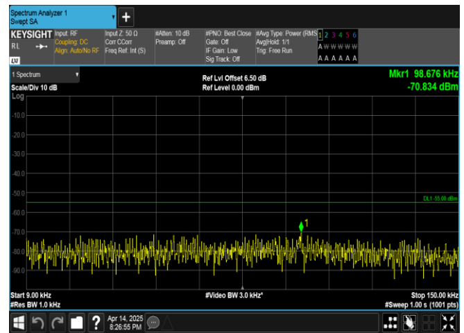
Band38-5MHz-16QAM-37775-1RB#0-0.009~0.15-PASS
