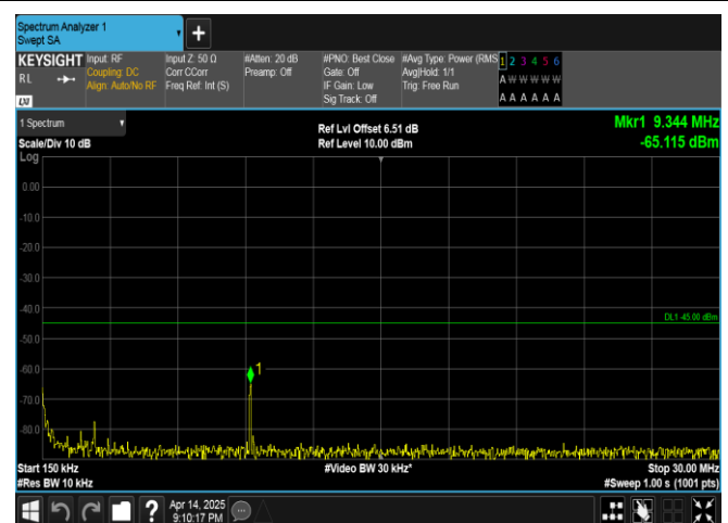
Band38-10MHz-QPSK-37800-1RB#0-0.15~30-PASS
