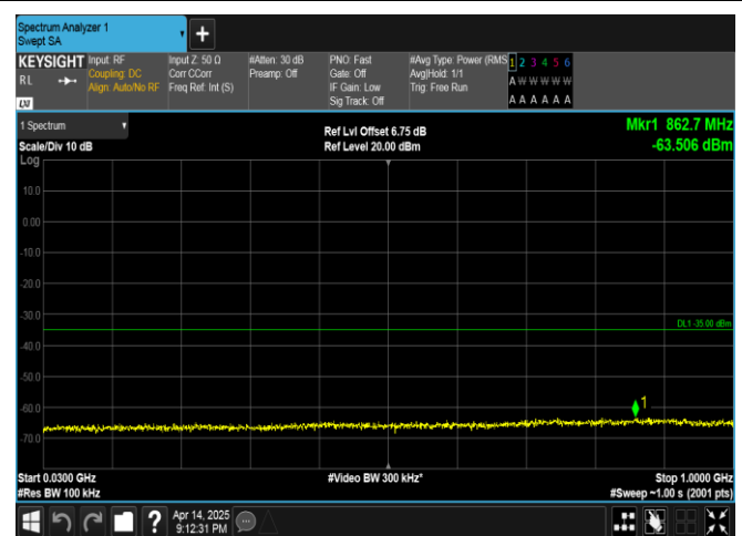
Band38-10MHz-QPSK-37800-1RB#49-30~1000-PASS
