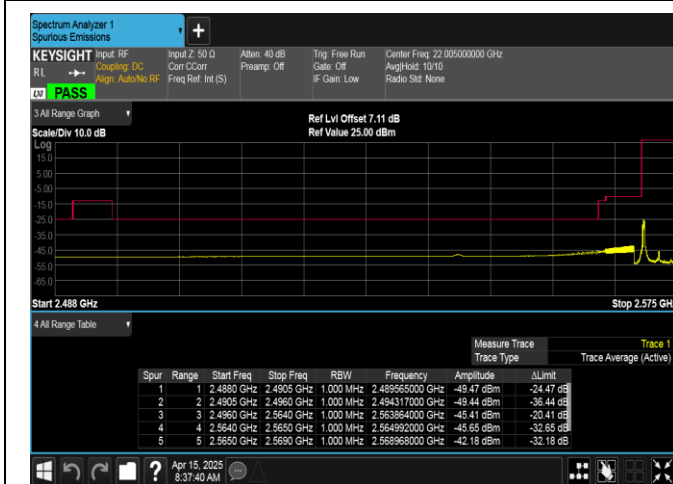
Band38-5MHz-16QAM-37775-1RB#0-PASS
