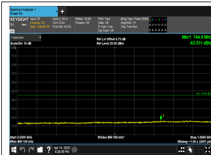
Band38-5MHz-QPSK-37775-1RB#0-30~1000-PASS
