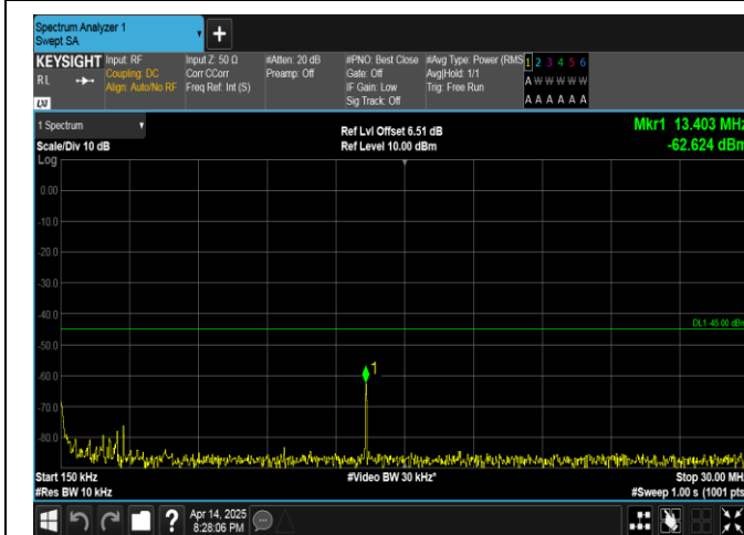
Band38-5MHz-QPSK-37775-1RB#24-0.15~30-PASS
