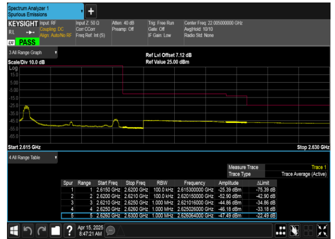
Band38-5MHz-QPSK-38225-1RB#0-PASS
