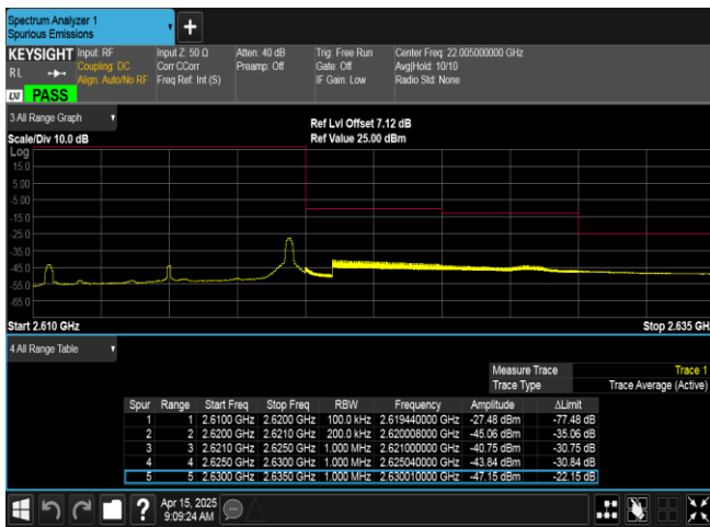
Band38-10MHz-QPSK-38200-1RB#49-PASS
