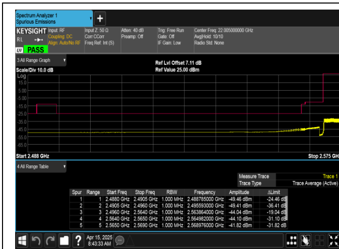
Band38-5MHz-QPSK-37775-25RB#0-PASS
