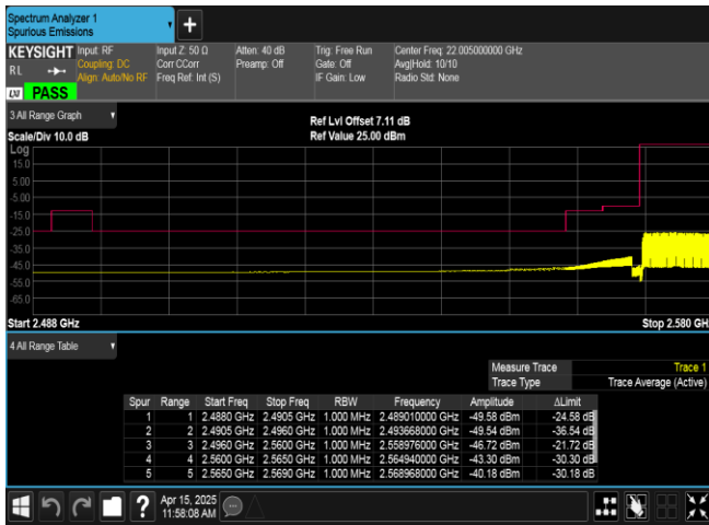
Band38-10MHz-QPSK-37800-50RB#0-PASS
