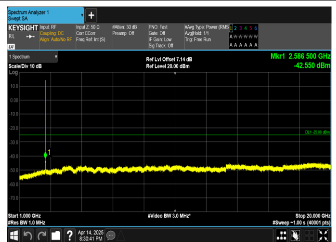
Band38-5MHz-QPSK-37775-25RB#0-1000~20000-PASS
