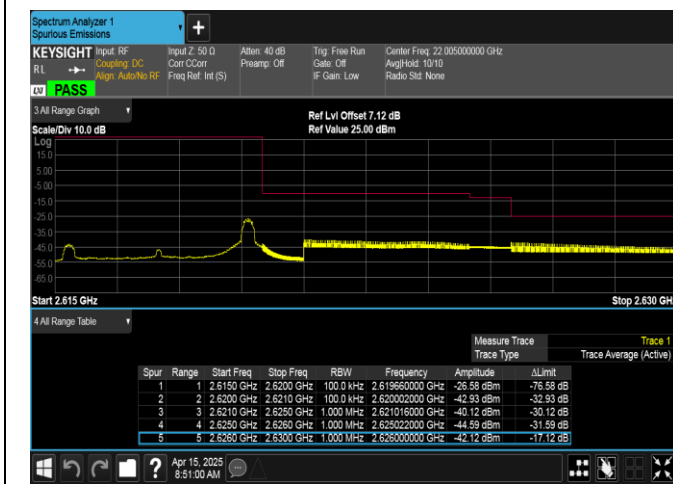
Band38-5MHz-QPSK-38225-1RB#24-PASS
