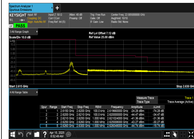
Band38-5MHz-16QAM-38225-1RB#24-PASS
