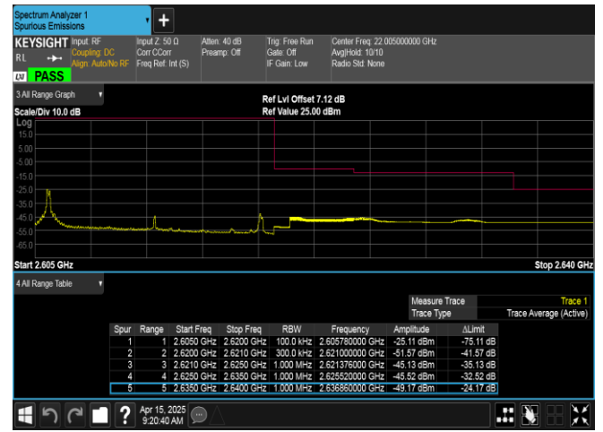
Band38-15MHz-QPSK-38175-1RB#0-PASS
