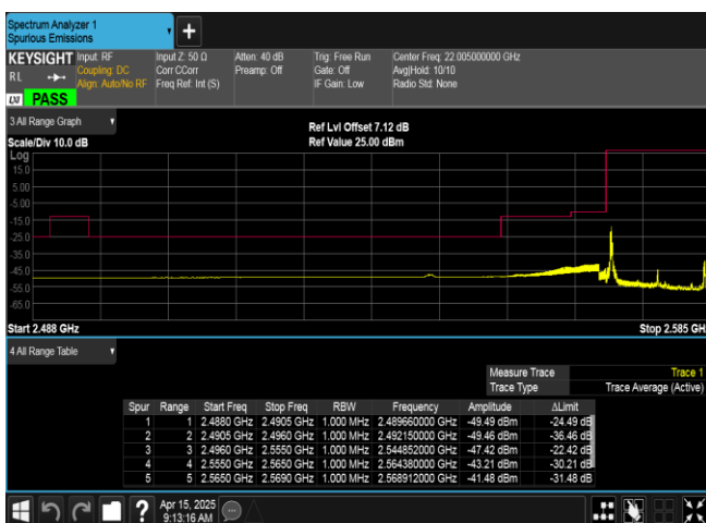
Band38-15MHz-QPSK-37825-1RB#0-PASS
