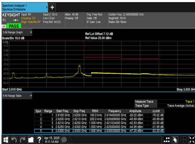
Band38-10MHz-16QAM-38200-1RB#49-PASS
