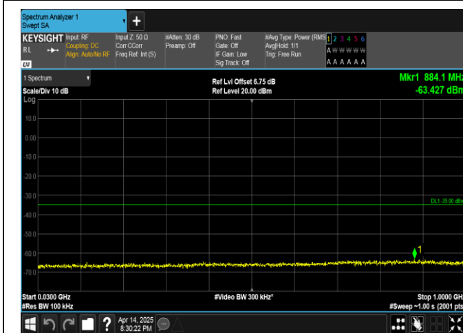
Band38-5MHz-QPSK-37775-25RB#0-30~1000-PASS
