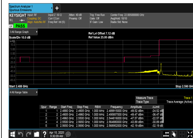
Band38-20MHz-16QAM-37850-1RB#0-PASS
