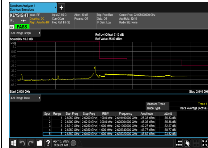
Band38-15MHz-QPSK-38175-1RB#74-PASS
