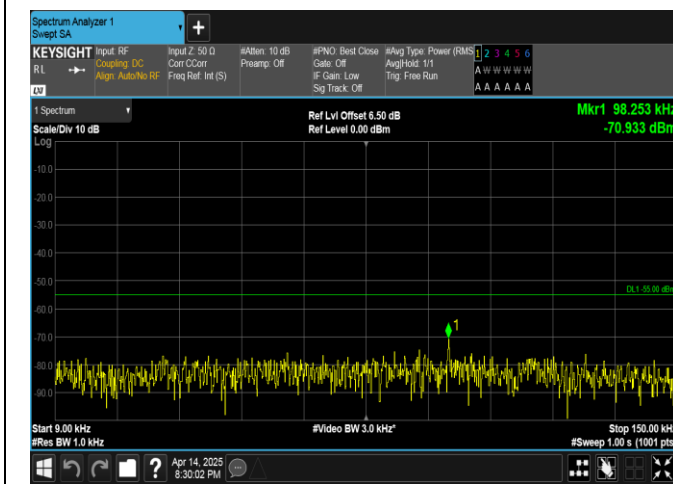
Band38-5MHz-QPSK-37775-25RB#0-0.009~0.15-PASS
