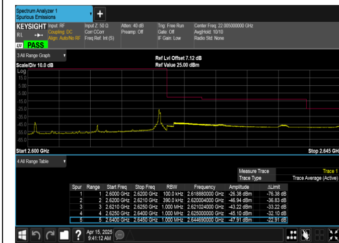
Band38-20MHz-16QAM-38150-1RB#99-PASS
