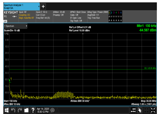
Band38-5MHz-QPSK-37775-25RB#0-0.15~30-PASS
