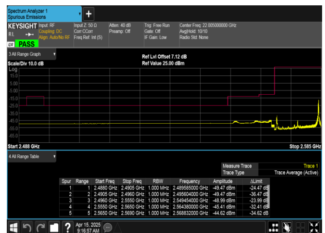
Band38-15MHz-QPSK-37825-1RB#74-PASS
