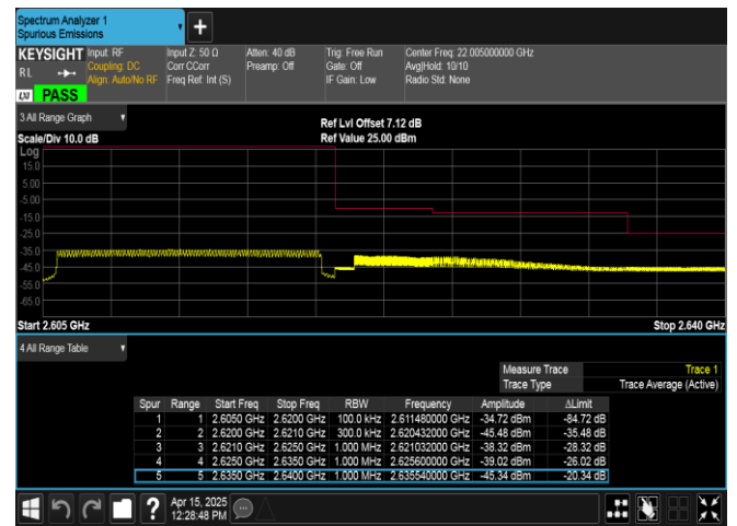
Band38-15MHz-QPSK-38175-75RB#0-PASS
