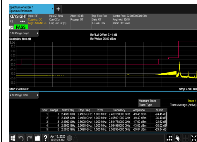
Band38-10MHz-QPSK-37800-1RB#0-PASS
