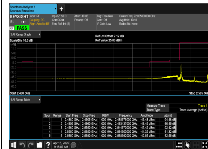
Band38-15MHz-16QAM-37825-1RB#0-PASS
