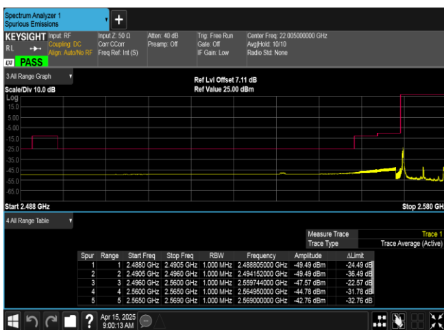
Band38-10MHz-16QAM-37800-1RB#0-PASS
