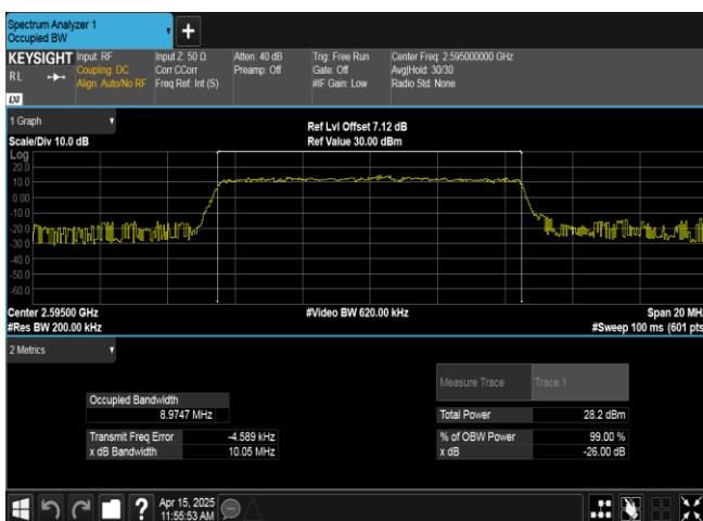
Band38-10MHz-16QAM-38000-50RB#0-PASS
