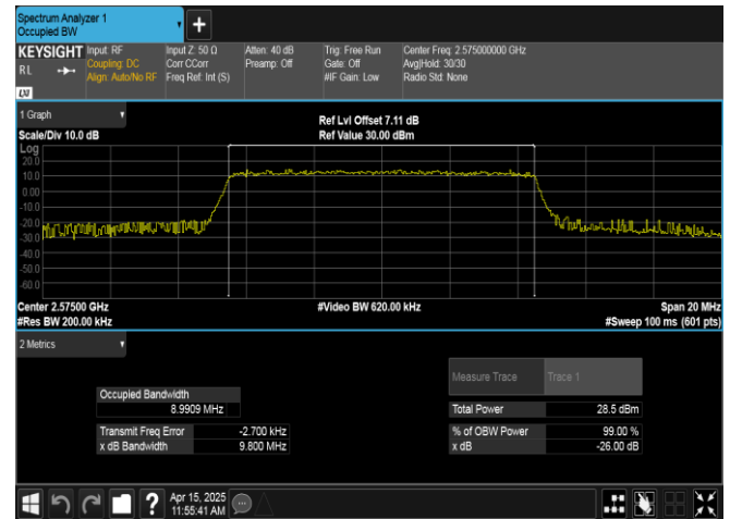
Band38-10MHz-16QAM-37800-50RB#0-PASS
