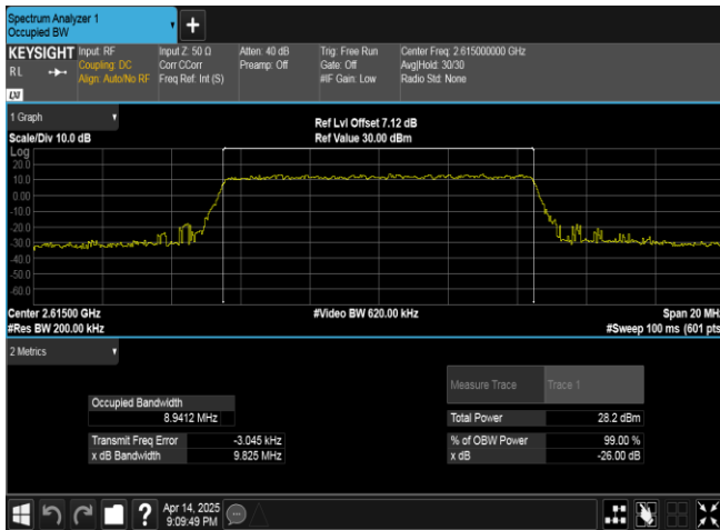
Band38-10MHz-QPSK-38200-50RB#0-PASS
