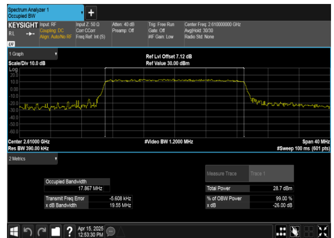
Band38-20MHz-16QAM-38150-100RB#0-PASS
